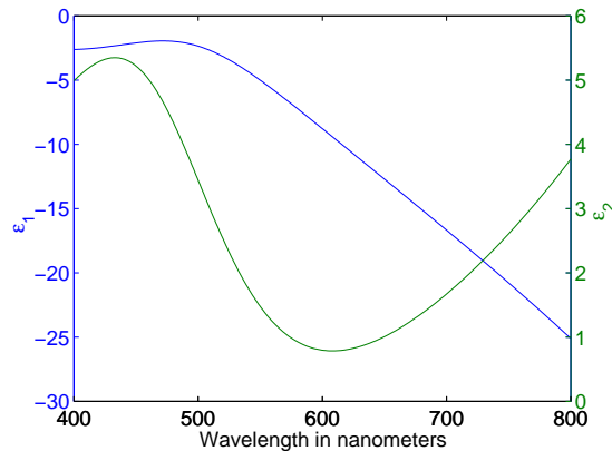
FIGURE 4.3: Epsilon value of Gold is plotted from the values present in the Lumerical's FDTD software for Gold (Johnson and Christy) with the help of function getfddindex .
