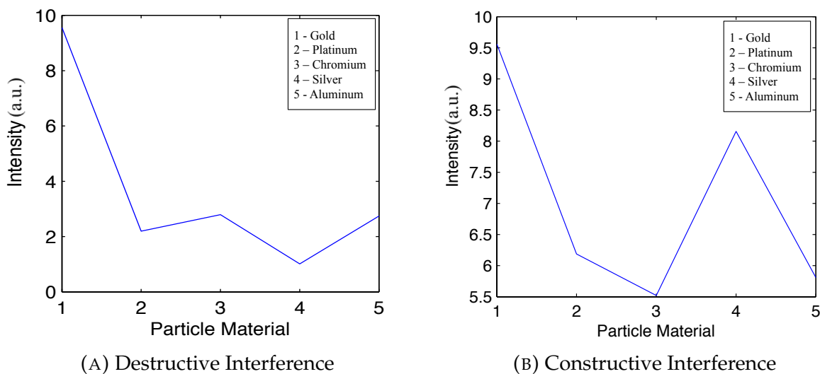
FIGURE A.6: In this calculation a rectangular particle of base 150 nm and height 100 nm is considered. The rectangular particle of different materials like Gold, Platinum, Chromium, Silver and Aluminium are used for simulation. Total Intensity of each material is calculated when observed in air.
