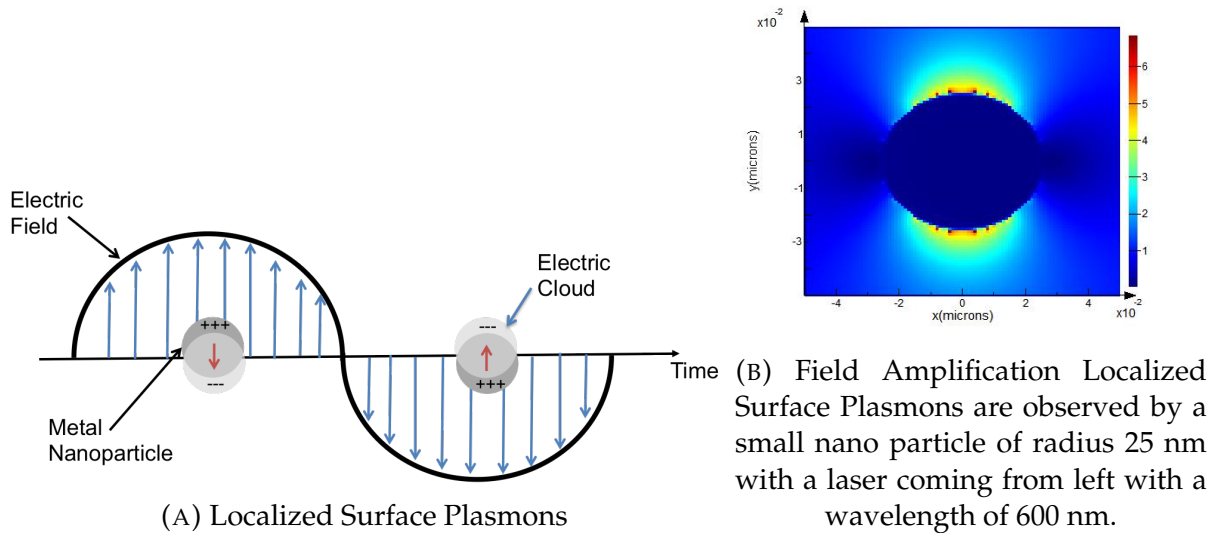
FIGURE 4.5: Localized Surface Plasmons and Field amplification in and around the near Field of the Nanoparticle
