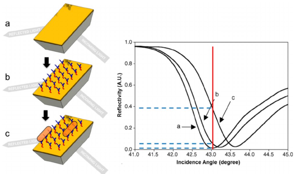
FIGURE 4.2: Shift of Resonance from the initial state to functionalized Gold Layer and ultimately when an analyte interacts with the functionalized Gold Layer
