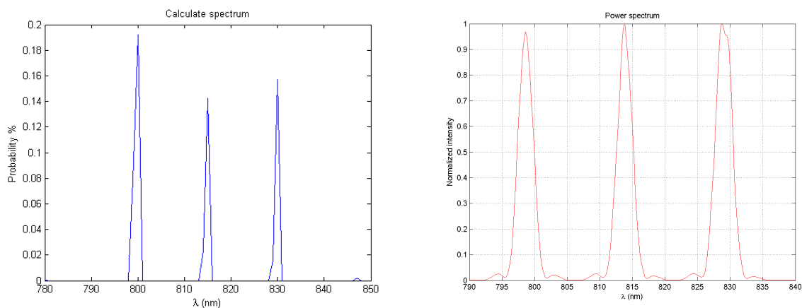
(A) 3 different Laser wavelengths as calculated (B) 3 different Laser wavelengths as viewed by a commercial spectrometer.
