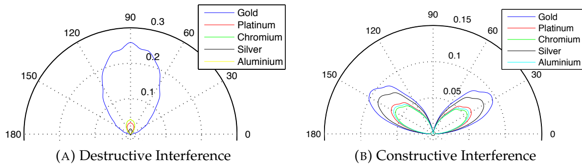
FIGURE A.4: In this calculation a rectangular particle of base 150 nm and height 100 nm is considered. The rectangular particle of different materials like Gold, Platinum, Chromium, Silver and Aluminium are used for simulation.
