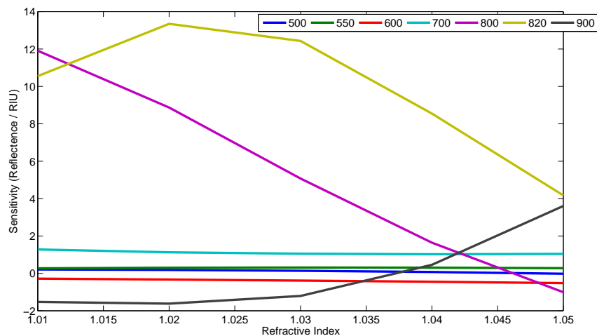
FIGURE 4.27: Graph showing the effect of sensitivity with the variation of refractive index for multiple wavelengths for "W" structure having a length of 600 nm and thickness of 25 nm.
