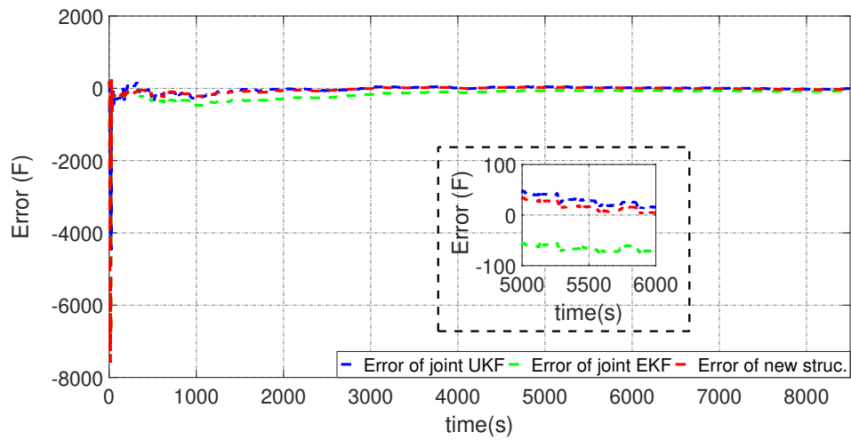
(b) Estimation error of C_1
