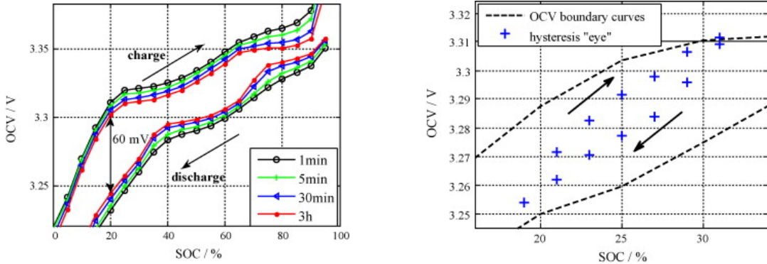
(a) OCV curves of the LFP-based cells measured after various rest periods at each step [81].
