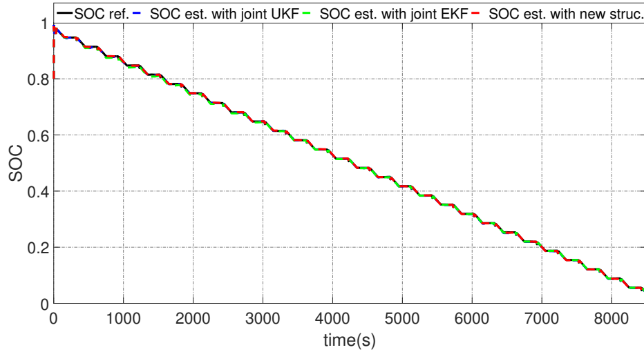
(a) Estimation result of SOC
