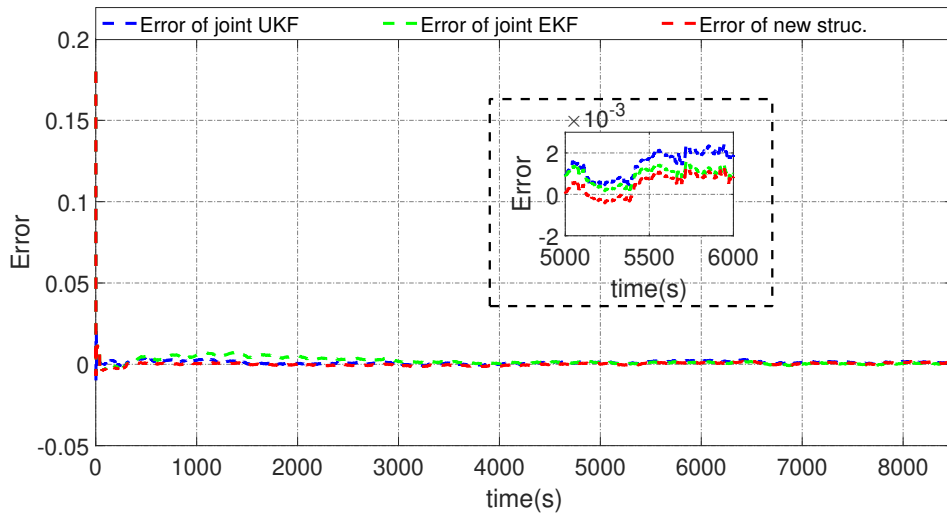
(b) Estimation error of SOC
