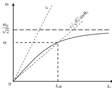
Figure 11.4: Left: Dispersion relation of the surface plasmon mode in metal. Coupling of a plasmon with an evanescent wave, in condition of total reflexion with a prism of \epsilon_1 > 1 . \omega_p is the plasmon angular frequency in a Drude model, k_0 = \omega/c . From Le champ proche optique - Theorie et applications , Daniel Courjon et Claudine Bainier [55].
