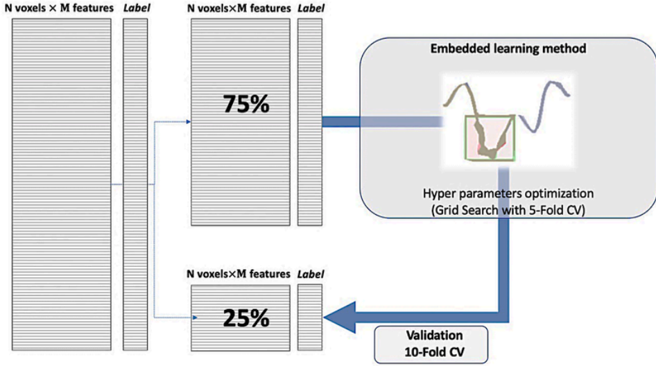
Figure 3.23: Overview of the feature selection methodology.
