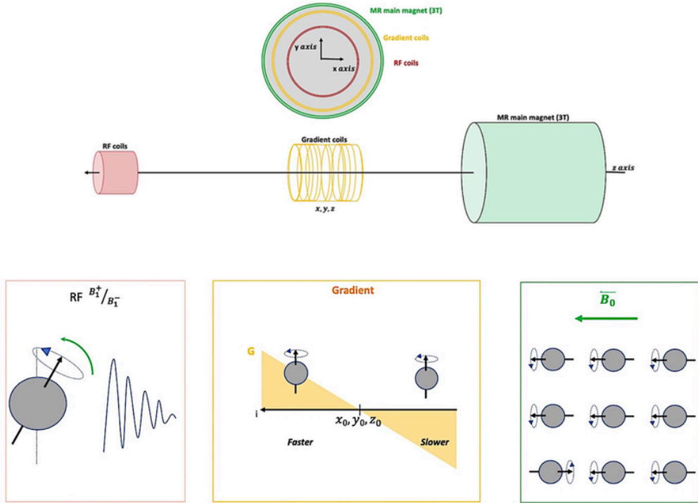
Figure 2.3: MR principles. The spins in the MR magnet are aligned to \vec{B}_0 (green); the RF chain (red) transmits a rotating RF pulse B_1^+ to the spins and receives the electromagnetic signal B_1^- generated by the spin relaxation. The received signal is spatially encoded by using transient magnetic gradient fields (orange).
