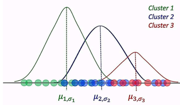
Figure 3.12: Concept of Gaussian Mixture Model clustering. All the voxels are assigned to a Gaussian X_i \sim (\mu_i; \sigma_i) .
