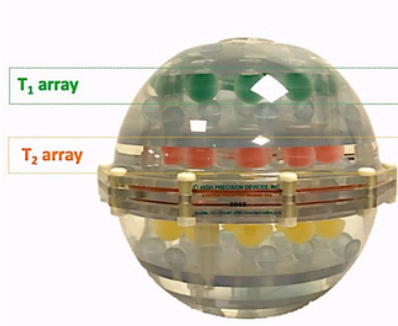
Figure 2.35 : MRI System Phantom (qMRI, High Precision Devices, Inc., Boulder, Colorado, USA). Each sphere of the T 1 and T 2 arrays have calibrated T 1 and T 2 values.
