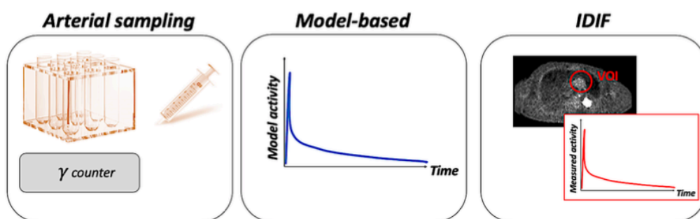
Figure 1.11: methods for AIF measurement. Arterial sampling with radioactivity counting remains the gold standard. However, this invasive procedure is rarely performed and model-based or image-derived input functions (IDIF) are preferred in practice.
