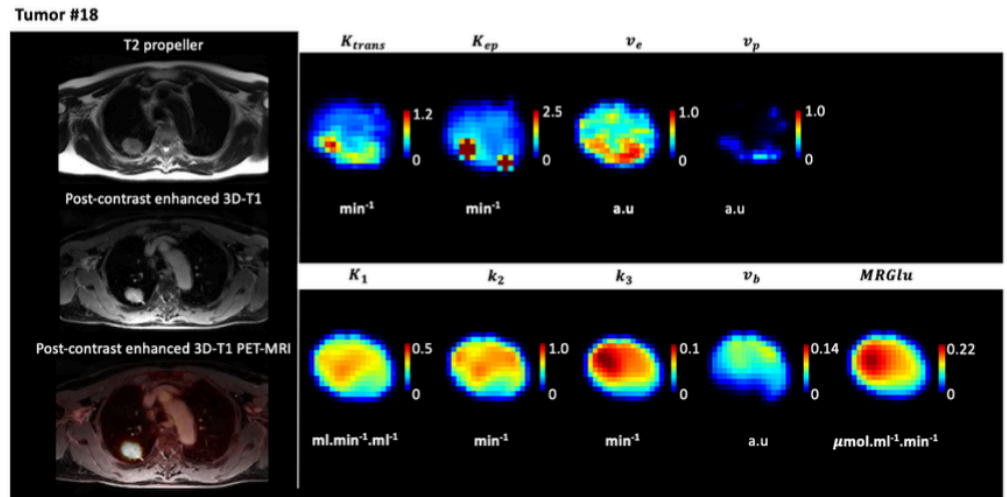
Figure 3.11: DCE and ^{18}\text{F} -FDG PET multiparametric maps of the right posterior upper lobe tumor (patient 18). For illustration, all parametric maps were smoothed with a 3mm Gaussian filter.
