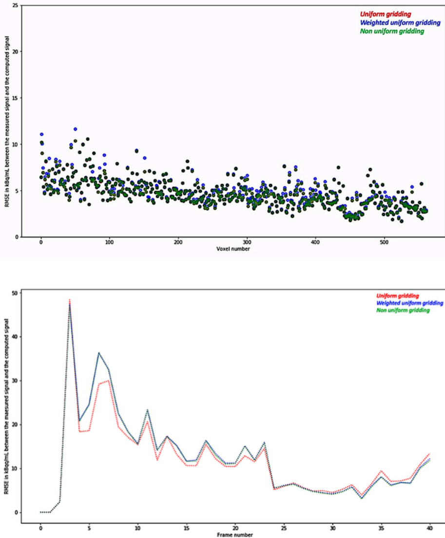
Figure A. 3: Without smoothing, the mean iteration number was increased (18.6, 28.7 and 18.2 respectively for uniform, uniform weighted and nonuniform) and for 12 voxels, the nonuniform method did not converged after the maximal 400 iterations. Also, as provided in the figures, RMSE among the frames were higher (median values were 10.6, 11.2 and 11.1 kBq/ml). In all the case, RSME between the 4th and 5th frame (40s and 50s post-injection respectively) increased together with the signal measured, corresponding to the first blood pass. Overall RMSE4 and RMSE5 were 48.4 kBq/ml and 18.3 kBq/mL; 47.4 kBq/mL and 20.9 kBq/mL; and 47.1 kBq/mL and 20.7 kBq/mL for the uniform, uniform weighted and nonuniform gridding respectively (for the smoothed PET data: 52.3 kBq/mL and 12.8 kBq/mL; 46.8 kBq/mL and 22.4 kBq/mL; and 46.8 kBq/mL and 22.4 kBq/mL for the uniform, uniform weighted and nonuniform gridding respectively).
