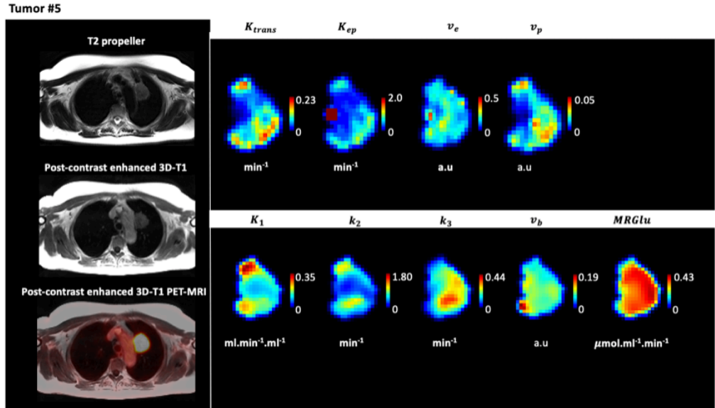
Figure 3.10: DCE and ^{18}\text{F} -FDG PET multiparametric maps of the left upper lobe tumor (patient 5). For illustration, all parametric maps were smoothed with a 3mm Gaussian filter.
