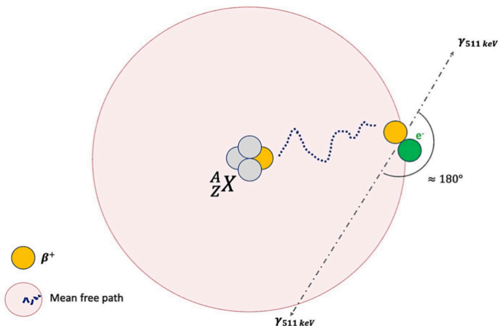
Figure 1.1 : Concept of electron-positron annihilation. The positron (in orange) interacts with an electron (green) to be converted into two photons of 511 keV. These two photons are emitted at approximately 180^\circ .
