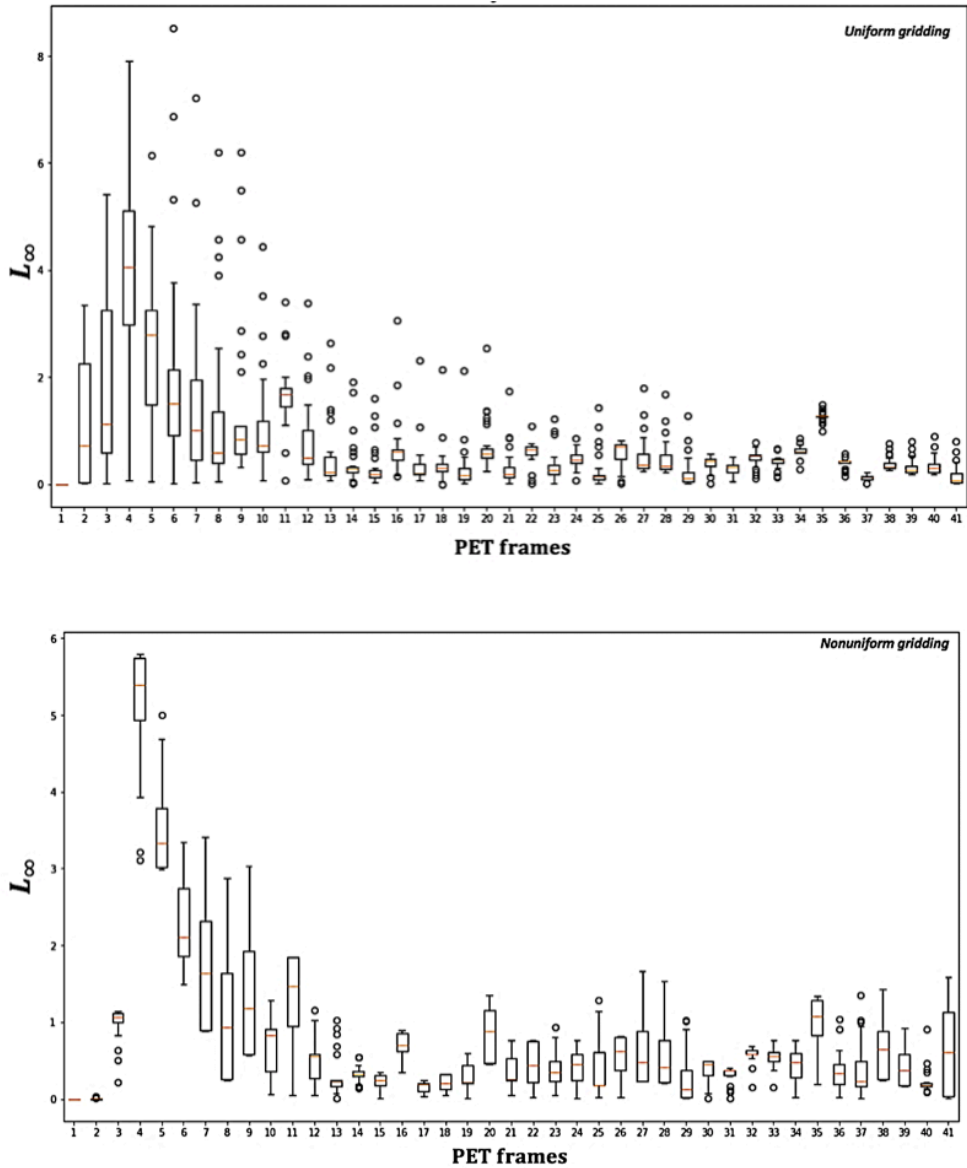
Figure A. 2 : These plots represent for each frame ( x -axis) the L_{\infty} norms of the 29 levels of points to be sampled (boxplots). We can see that, considering all the levels of data sampling, for the first 5 frames, the nonuniform gridding had better performance compared to uniform gridding (both lower L_{\infty} norm values and variability). For the 5th to the 30th frame, the nonuniform gridding provided less outliers. For the 31th to the 41th frame, the uniform gridding appeared more consistent.
