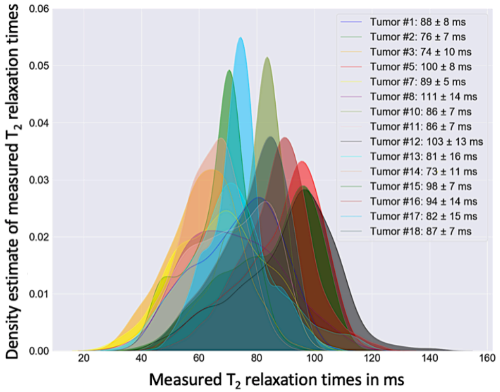
Figure 2.41: Measured T_2 values ( x -axis) and the corresponding density estimates ( y -axis). For each tumor, the mean T_2 value and standard deviation is also provided in the legend. Mean T_{2\text{MEFSE}} were in the range 73–111 ms.
