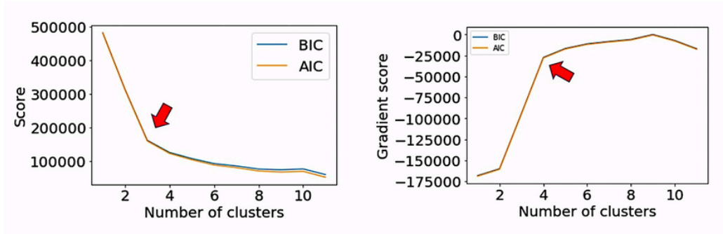
Figure 3.13: AIC and BIC scores as function of the number of clusters. The red arrows indicate, both for the AC/BIC score (left part) and their gradient versions (right part).
