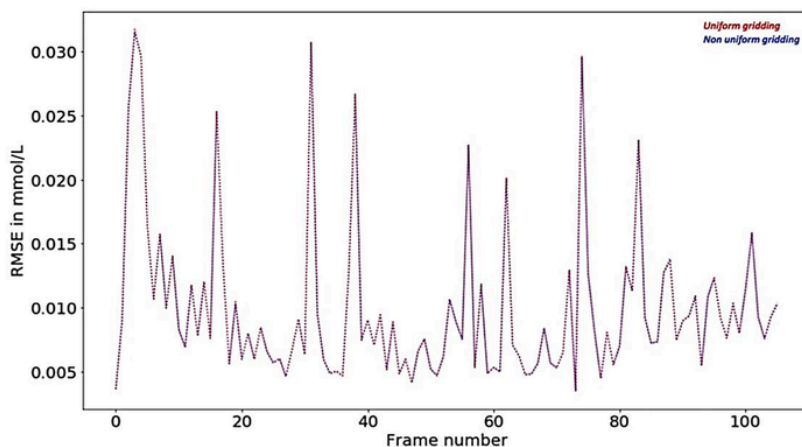
Figure 2.51: Per frame RMSE of gridding approaches for curve-fitting. The x -axis represents the frame identity numbers, and the y -axis the corresponding RMSE in mmol/L . The median RMSE (IQR) for the 106 frames were 0.008\text{ mmol/L} ( 0.006\text{--}0.01 ) both for the uniform and nonuniform gridding.
