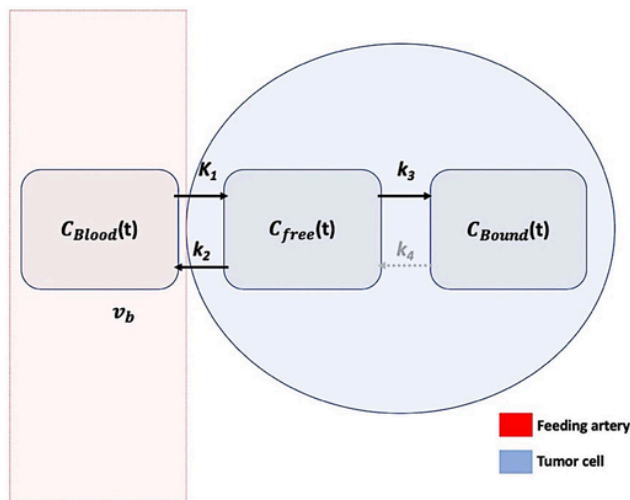
Figure 1.10: PET Sokoloff compartmental model. In this scheme, C_{Blood}(t) is the time-varying activity concentration of ^{18}\text{F} -FDG in the arterial blood. C_{free}(t) and C_{Bound}(t) are the two intracellular compartments representing ^{18}\text{F} -FDG in its non-phosphorylated and phosphorylated states respectively. K_1 , k_2 and k_3 are the microparameters to estimate (the k_4 microparameter can be neglected in this case, as no phosphorylated glucose goes out from the cell).
