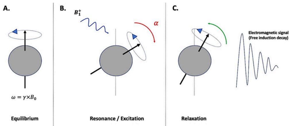
Figure 2.2: the phenomenon of Nuclear Magnetic Resonance (NMR). Under equilibrium, the spins are aligned along B_0 . A rotating RF pulse applied to the spins at Larmor frequency tilts them by energy transfer (excitation). The spins return then to equilibrium (relaxation) and generate an electromagnetic signal named free induction decay (FID).
