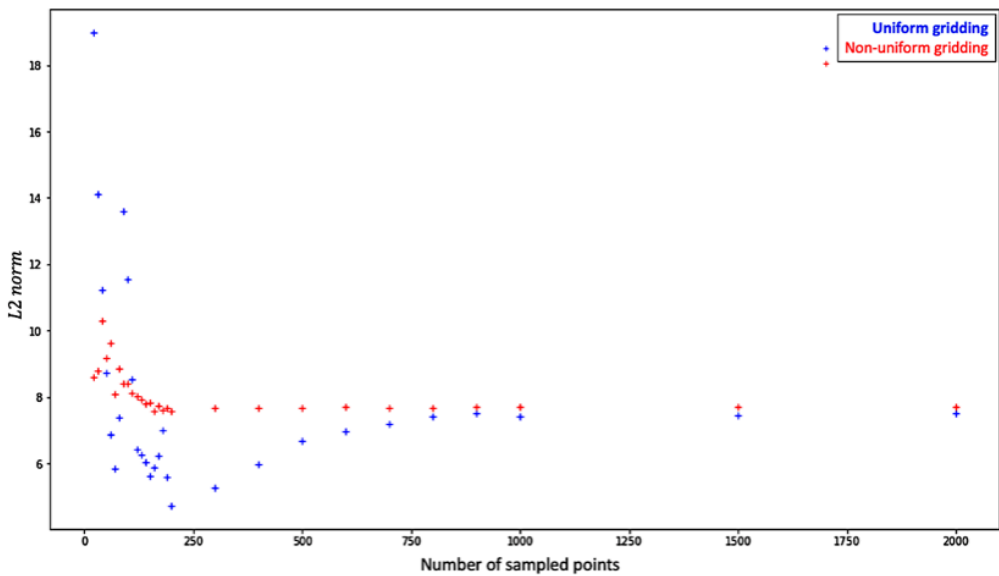
Figure A. 1 : This plot represents the number of points to be sampled (x-axis) function of the mean L2 norm of the overall voxels (y-axis) that corresponds to \sqrt{N} \times \text{RMSE} , where N is the number of frames. We can clearly see that, on this subset of 57 tumor voxels, the algorithm provides the same performance for uniform and non-uniform gridding above 1000 points.
