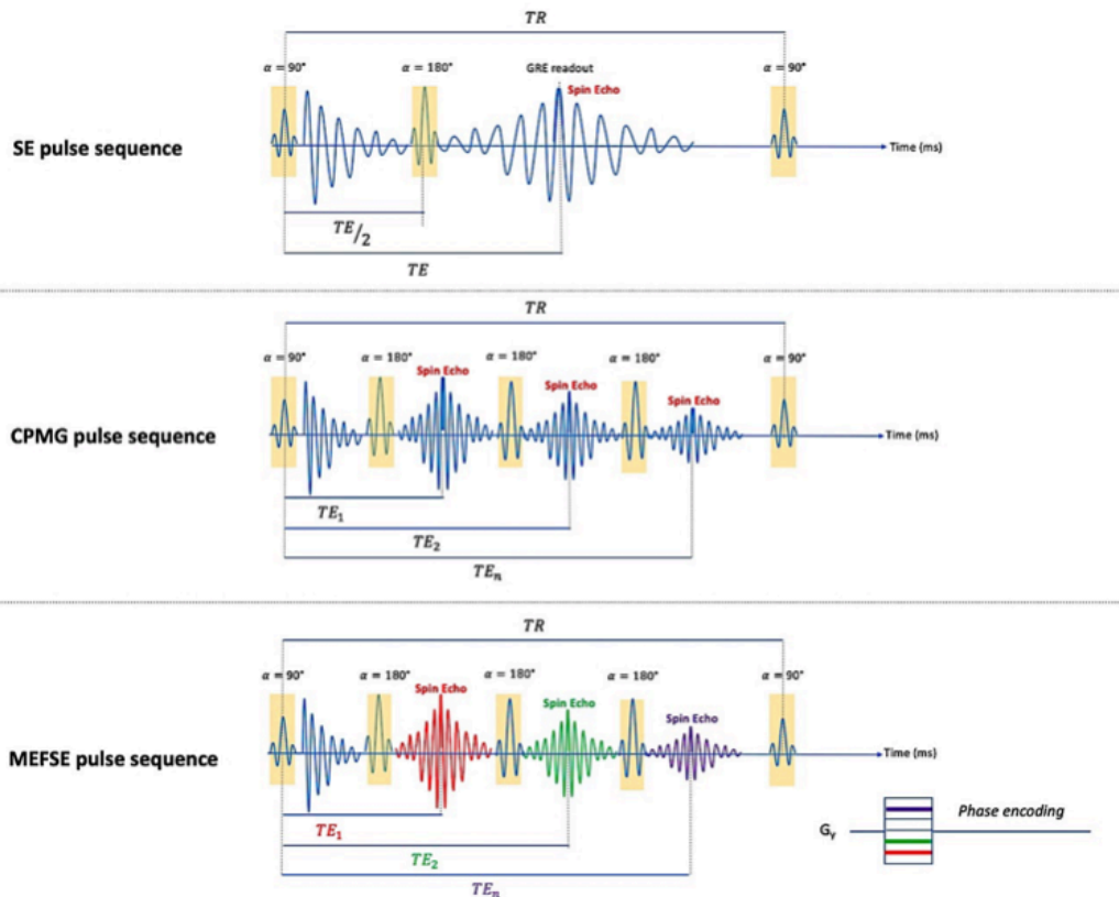
Figure 2.34: single-shot SE pulse sequence and its accelerated versions (CPMG and MEFSE). SE method consists in performing one acquisition per TE. CPMG method consist in generating a train of multiple echos by performing N successive 180^\circ refocusing pulses. The signal is measured at each TE following the initial 90^\circ RF pulse. In MEFSE, the CPMG concept is applied with ordered phase encoding to speed up the filling of k-space.
