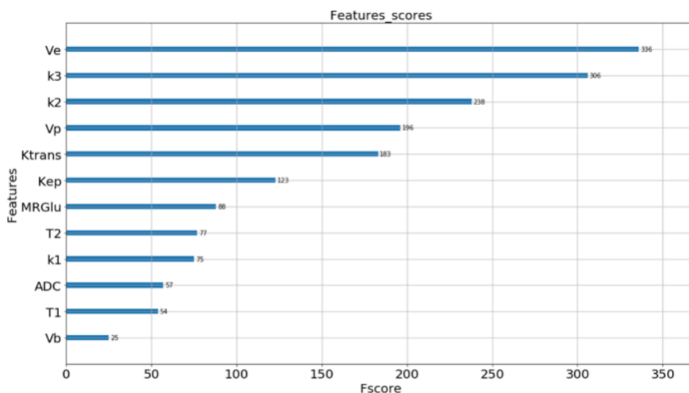
Figure 3.26: Features importance plot. F -scores ( x -axis) correspond to the number of times the features ( y -axis) are used to split the data across all trees. the most important features considered by the model are v_e , k_3 , k_2 and v_p parameters.
