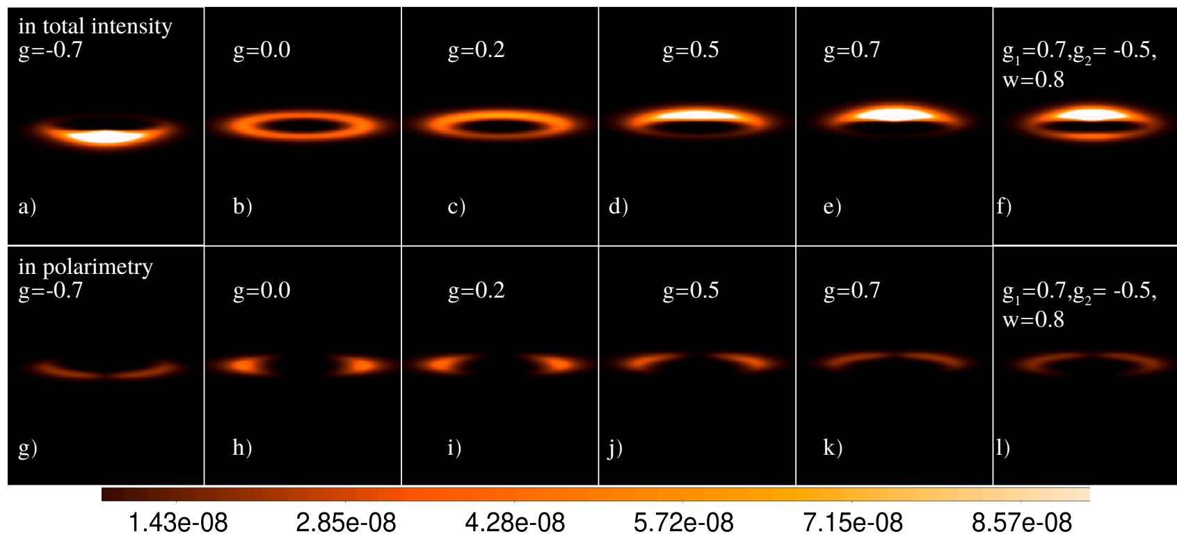
Figure 2.8 – GRaTer images including both geometrical and phase parameters to understand the affect of g in total intensity and polarimetry for an inclination i=8^\circ . The FOV of these images is 3.675'' \times 3.675'' . The colorbar represent the brightness scale of all the images.
