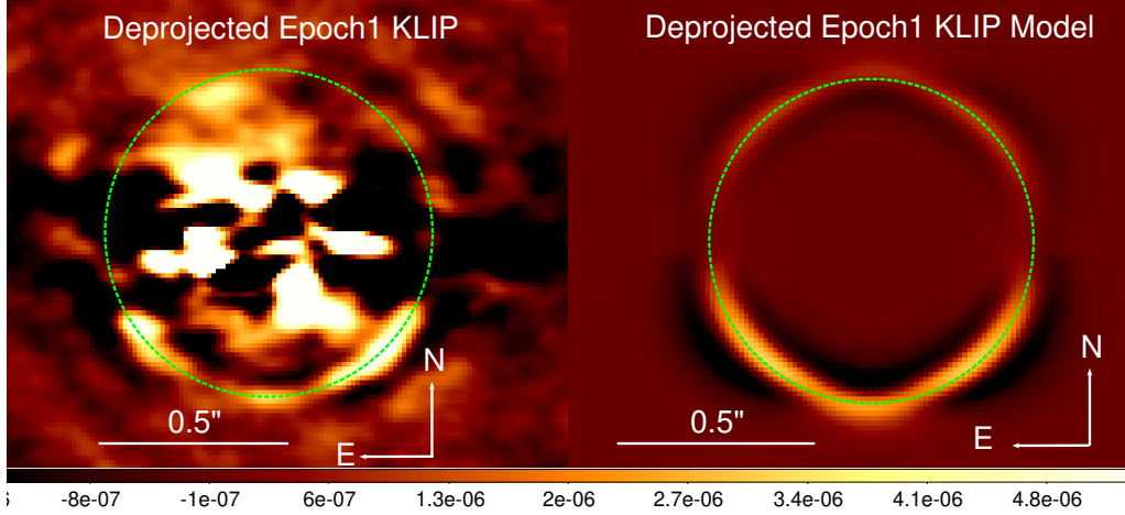
Figure 4.7 – On left is the image representing the de-projected KLIP 3 modes reduced IRDIS H2 data. On right is the image representing the de-projected KLIP 3 modes reduced best-fit model. The colorbar represent the intensity of both the images in arbitrary units. The image is cropped to 2'' \times 1.36'' and smoothed to a Gaussian kernel of 2 pixels
