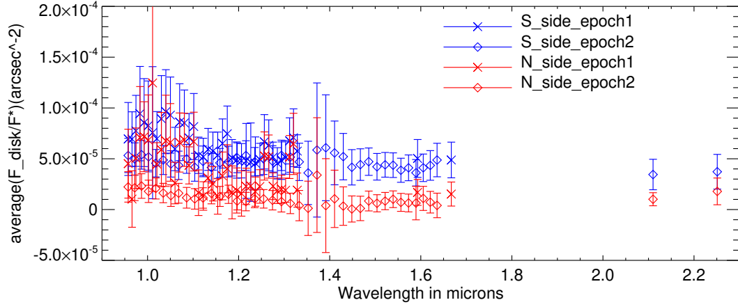
Figure 4.9 – The figure represents spectral reflectance corresponding to the northern and southern part of the ringlet R3 in both epochs.
