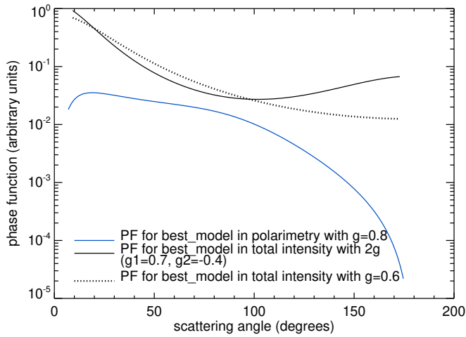
Fig. 6. Scattering phase function adopted for the total intensity and polarimetric best-fit models.
