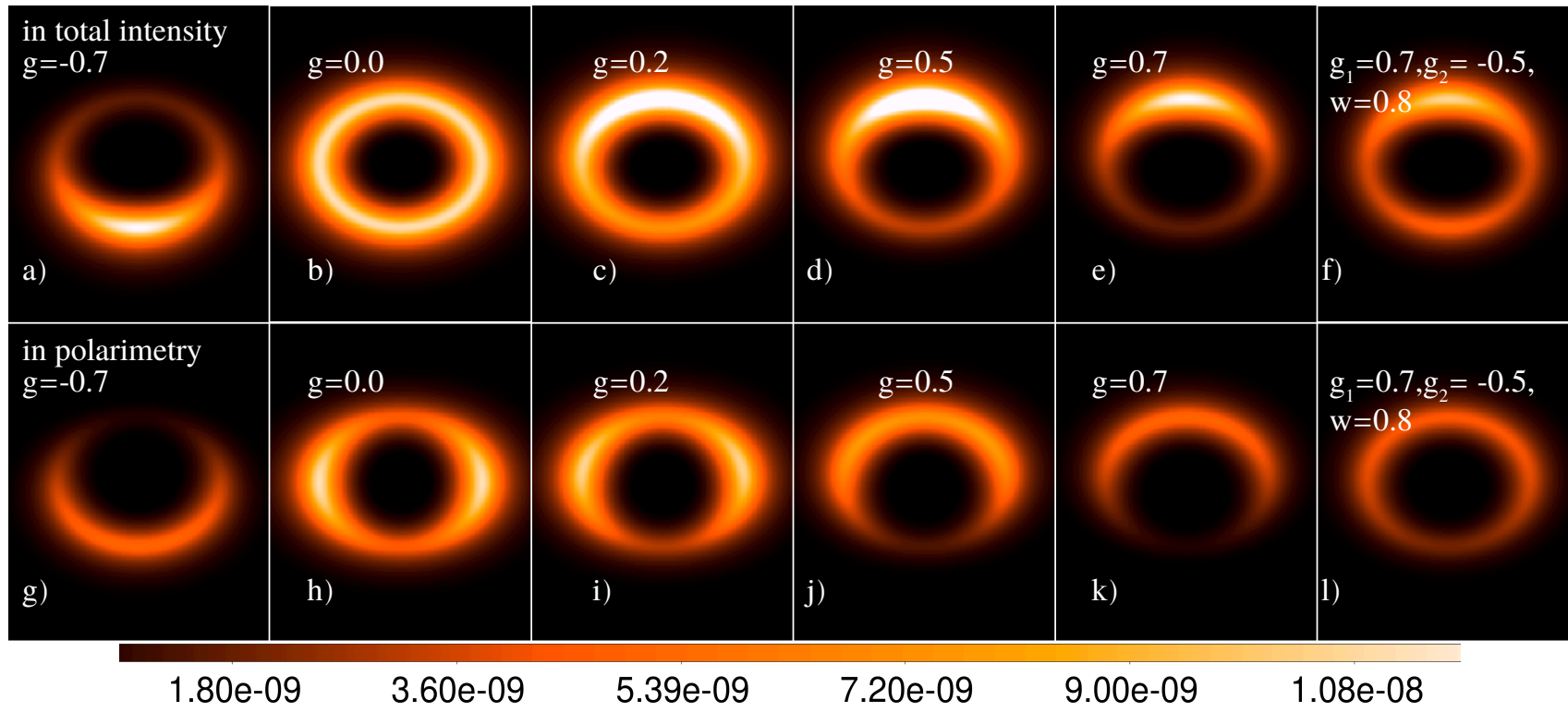
Figure 2.7 – GGrater images including both geometrical and phase parameters to understand the affect of g in total intensity and polarimetry for an inclination i=4^\circ . The FOV of these images is 3.675'' \times 3.675'' . The colorbar represent the brightness scale of all the images.
