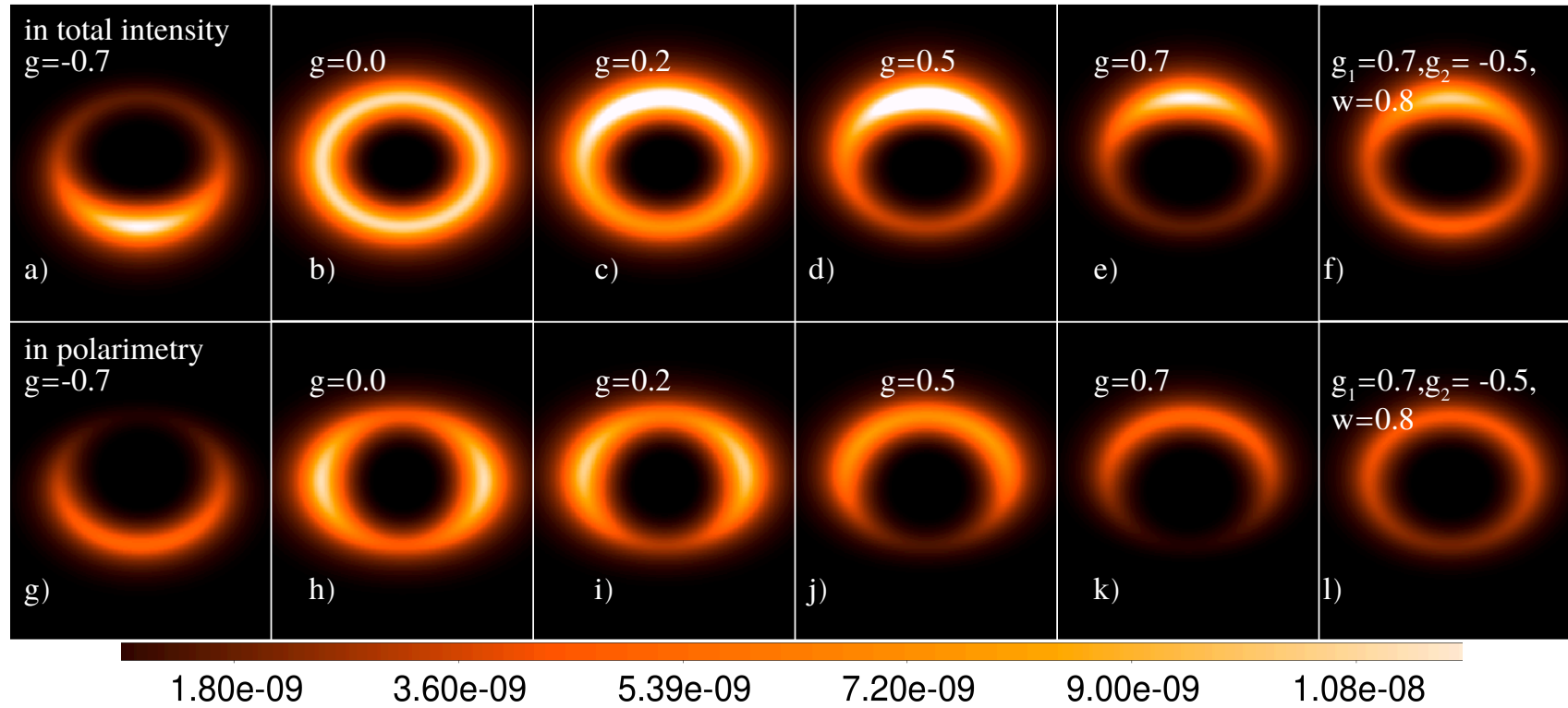
Figure 2.7 – GRaTer images including both geometrical and phase parameters to understand the affect of g in total intensity and polarimetry for an inclination i=4^\circ . The FOV of these images is 3.675'' \times 3.675'' . The colorbar represent the brightness scale of all the images.
