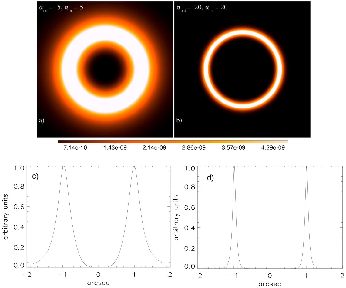
Figure 2.4 – a) and b) are the GRaTer images, using the geometrical parameters for R_0 = 100 au, h=0.04 and e=0 . The FOV of these images are 3.675'' \times 3.675'' . The colorbar represent the brightness scale of both the images. c) and d) are the plots representing the density variation across the disk corresponding to images a) and b) and normalised to the maximum of the image intensities.
