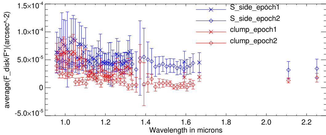
Figure 4.10 – The figure represents spectral reflectance plot corresponding to the clump and the southern part of the ringlet R3 masking out the clump in both the epochs.
