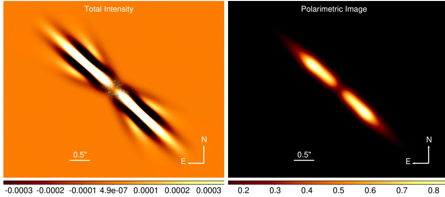
Figure 3.7 – Total Intensity model with the parameters i=88^\circ , \alpha_{out}=-6 , \alpha_{in}=2 , R_0=140 au, g_1=0.70 , g_2=-0.4 , w_1=0.80 , h=0.020 convolved with a 2D Gaussian PSF of FWHM=0.37'' . The dark stripes in the ADI processed model (Left) is an effect of ADI self-subtraction. Polarimetric model with parameters i=88.5^\circ , R_0=125 au, \alpha_{in}=10.0 , \alpha_{out}=-4.0 , g=0.8 , h=0.020 convolved with a 2D Gaussian PSF of FWHM=0.37'' .
