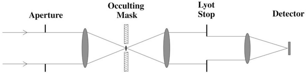
Figure 1.9 – Top: The image is of the first coronagraph used by Lyot displayed in Observatoire de Meudon, France. Bottom: Schematic sketch of operation of Lyot coronagraph (Sivaramakrishnan et al., 2001).
