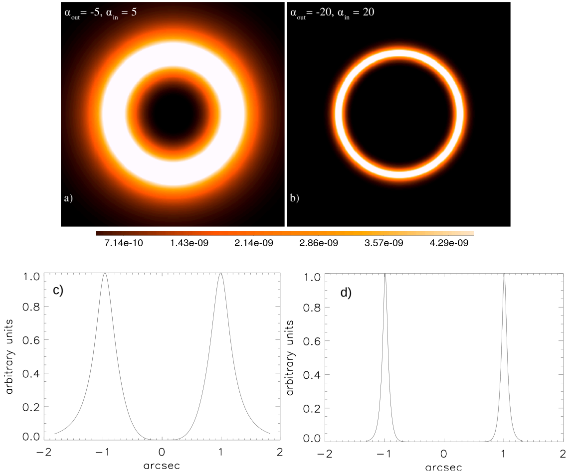
Figure 2.4 – a) and b) are the GRAFTer images, using the geometrical parameters for R_0 = 100 \text{ au} , h=0.04 and e=0 . The FOV of these images are 3.675'' \times 3.675'' . The colorbar represent the brightness scale of both the images. c) and d) are the plots representing the density variation across the disk corresponding to images a) and b) and normalised to the maximum of the image intensities.
