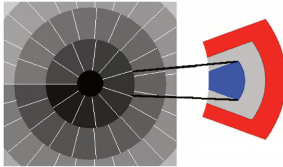
Figure 2.3 – The section of interest (blue) and the section of optimisation (blue) representation for LOCI. The section of interest (blue) and the section of optimisation (red) representation for TLOCI as in Galicher et al. (2018)
