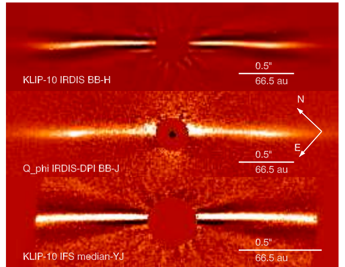
Fig. 2. Inner part of the disk with IRDIS in BB_H (KLIP, top ), IRDIS in DPI ( Q_\phi , middle ), and IFS ( YJ combined, bottom ). The top two images are cropped at 3'' \times 0.8'' and the IFS image is cropped at 2'' \times 0.5'' . All images are rotated to 90^\circ - \text{PA} . All images are scaled linearly in the range [-1 \times 10^{-5}, 1 \times 10^{-5}] .
