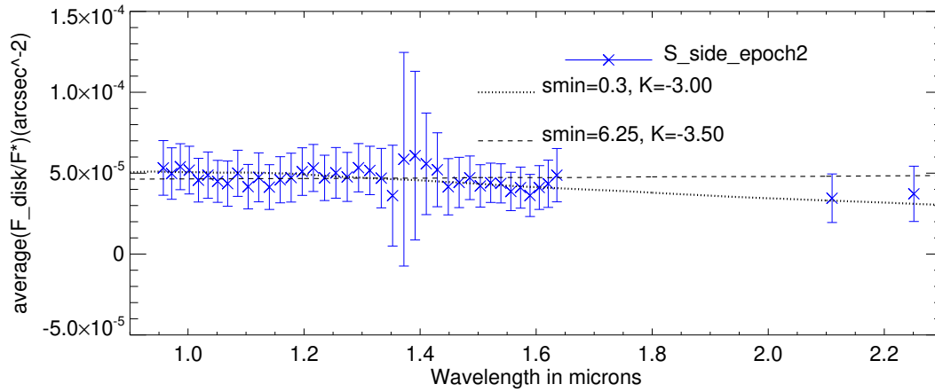
Figure 4.12 – Fitted synthetic spectra to the reflectance spectrum of epoch2. The dotted line represents the best-fit spectra with s_{min} = 0.30 \mu\text{m} and \kappa = -3.00 and the dashed line represent the spectra for fiducial case where s_{min} = s_{blow} and \kappa = -3.5 .
