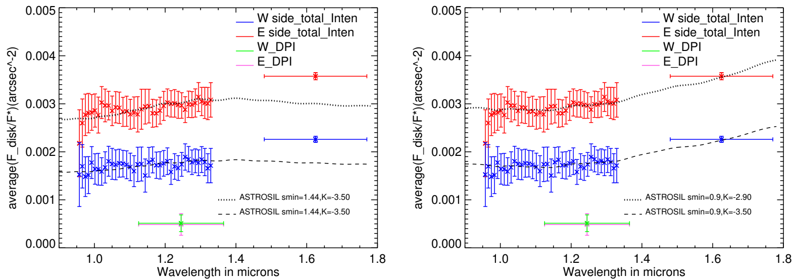
Figure 4.20 – Best fits of the reflectance spectrum obtained for a fiducial case with s_{min} = s_{low} and \kappa = -3.5 (left), and for best-fit when s_{min} and \kappa are free parameters (right).
