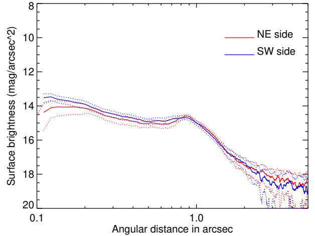
Fig. 11. Surface brightness profile of the disk measured in the IRDIS BB_J DPI Q_p science image. The blue line represents the SW side of the disk and the red line represents its counterpart on the NE side. The dotted lines represent the error bars.
