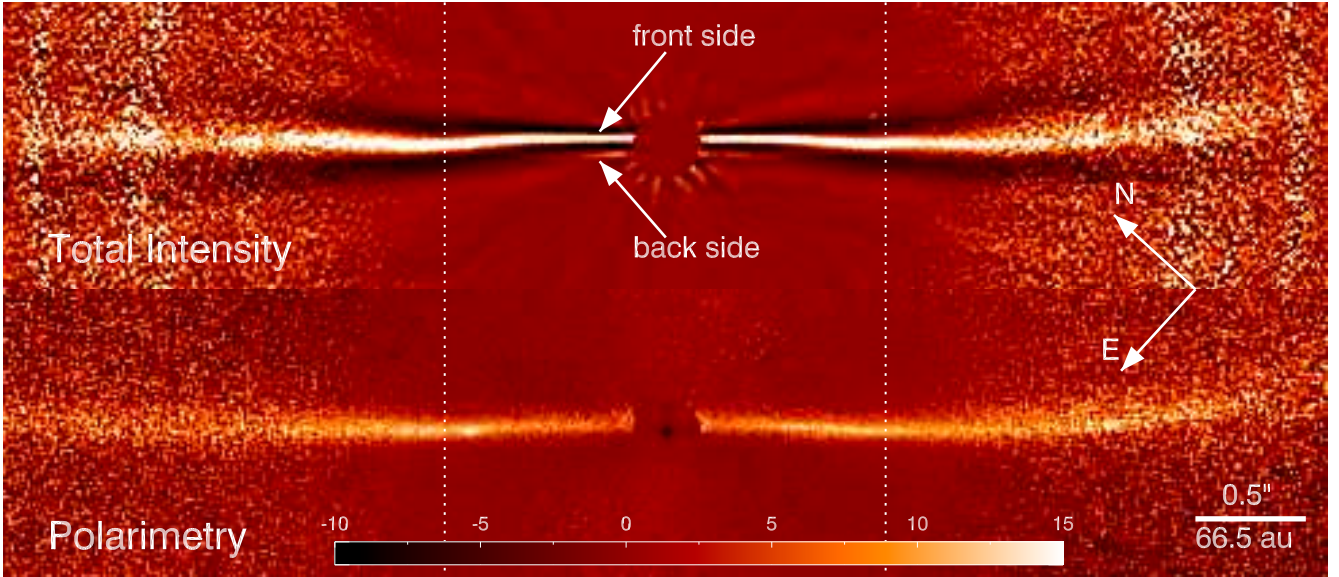
Fig. 1. Top: S/N map of total intensity with IRDIS in BB_H filter. Bottom: S/N map of polarimetric image observed with IRDIS in BB_J filter. The dashed line indicates approximate position of the ansa in both images and the arrows indicate front and back sides of the disk. Both images are rotated to 90^\circ - \text{PA} and cropped at 6'' \times 1.3'' . The color bar shows the intensity in both the images.
