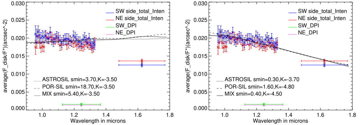
Fig. 14. Best fits of the reflectance spectrum (method 2) obtained for three different grain compositions, for a fiducial case where we force s_{\min} = s_{\text{blow}} and \kappa = -3.5 (left), and when s_{\min} and \kappa are free parameters (right).
