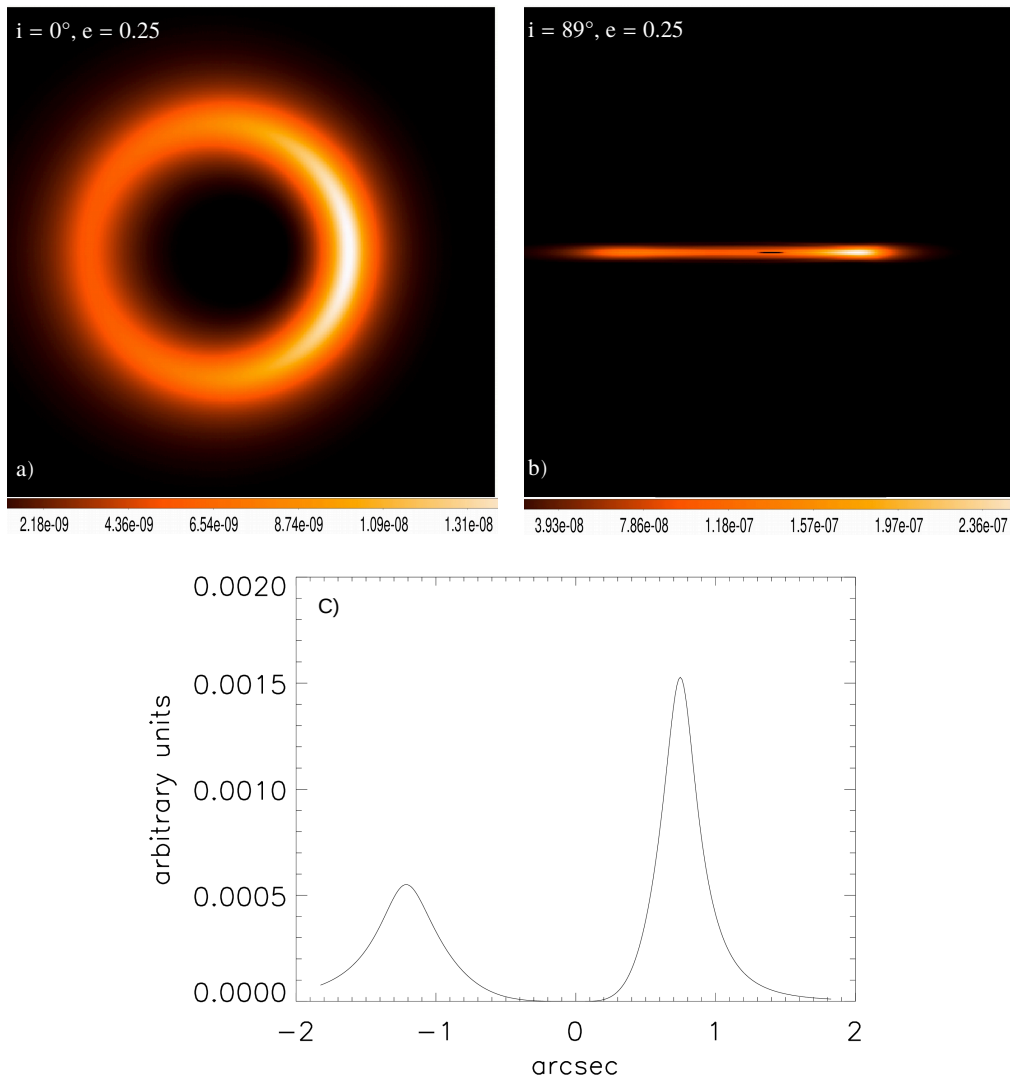
Figure 2.6 – a) and b) are the GRaTer images, using the geometrical parameters R_0 = 100 \text{ au} , \alpha_{in} = 5 , \alpha_{out} = -5 . The FOV of these images are 3.675'' \times 3.675'' . The colorbars represent the brightness scale in the images. c) is the plot representing the density variation across the disk corresponding to images a) and normalised to the maximum of the image intensities.
