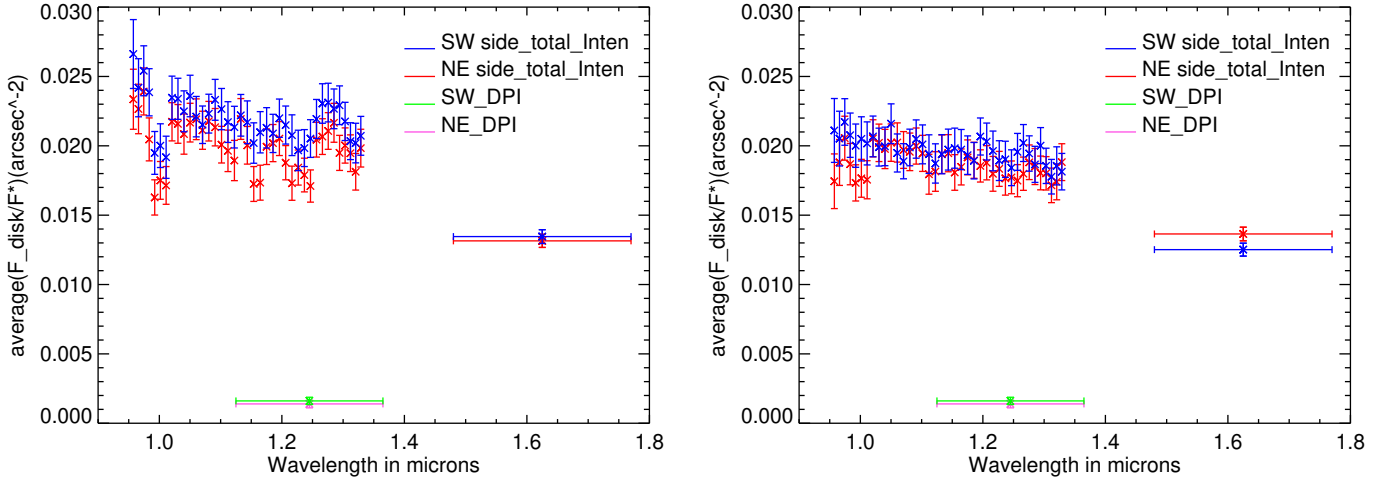
Fig. 12. Average spectral reflectance of HD 32297 as measured with method 1 ( left ) and method 2 ( right ), for total intensity data in IFS YJ and IRDIS BB_H , as well as polarimetric data in IRDIS BB_J .
