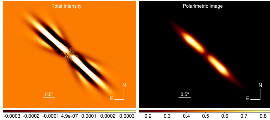
Figure 3.7 – Total Intensity model with the parameters i=88^\circ , \alpha_{out}=-6 , \alpha_{in}=2 , R_0=140 au, g_1=0.70 , g_2=-0.4 , w_1=0.80 , h=0.020 convolved with a 2D Gaussian PSF of HWHM= 0.37'' . The dark stripes in the ADI processed model (Left) is an effect of ADI self-subtraction. Polarimetric model with parameters i=88.5^\circ , R_0 = 125 au, \alpha_{in} = 10.0 , \alpha_{out}=-4.0 , g=0.8 , h=0.020 convolved with a 2D Gaussian PSF of HWHM= 0.37'' .
