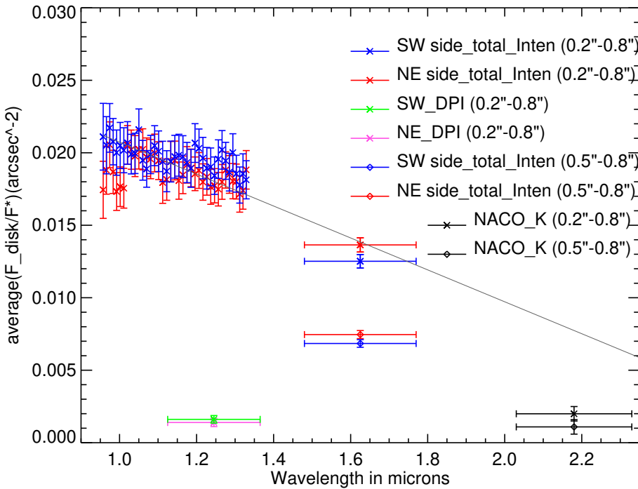
Fig. 12. Average spectral reflectance of HD 32297 as measured with method 1 ( left ) and method 2 ( right ), for total intensity data in IFS YJ and IRDIS BB_H , as well as polarimetric data in IRDIS BB_J .
