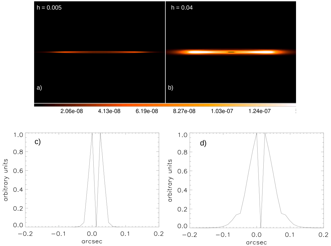
Figure 2.5 – a) and b) are the GRAFTer images, using the geometrical parameters R_0 = 100 \text{ au} , \alpha_{in} = 5 , \alpha_{out} = -5 , i = 89^\circ and e = 0 . The FOV of these images are 3.675'' \times 3.675'' . The colorbar represent the brightness scale of both the images. c) and d) are the plots representing the density variation across the disk corresponding to images a) and b) and normalised to the maximum of the image intensities.
