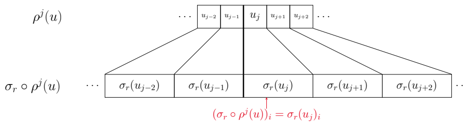
Figure 3.8 – Illustration of Lemma 3.3.6.
