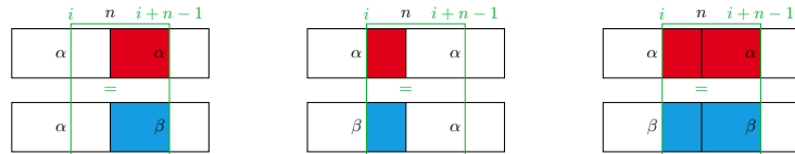
Figure 3.10 – The three cases for S_i to be of cardinal 2: the window in green represents an equality, and the colored portions are the consequent parts of \alpha and \beta made equal.
