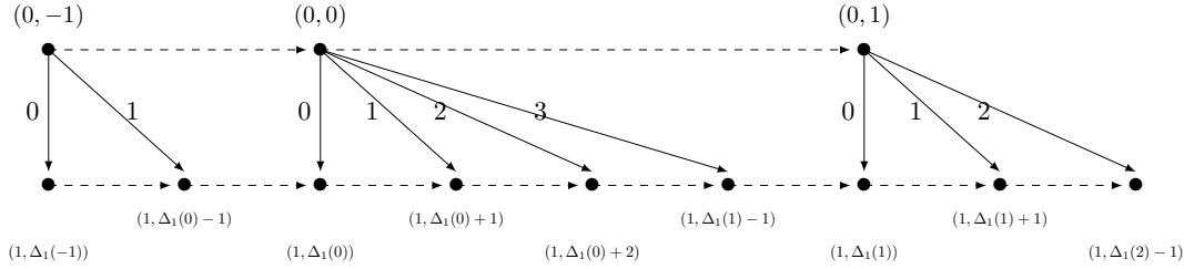
Figure 3.2 – Part of an orbit graph. Dashed arrow are edges of the graph labeled with \mathbf{next} .
