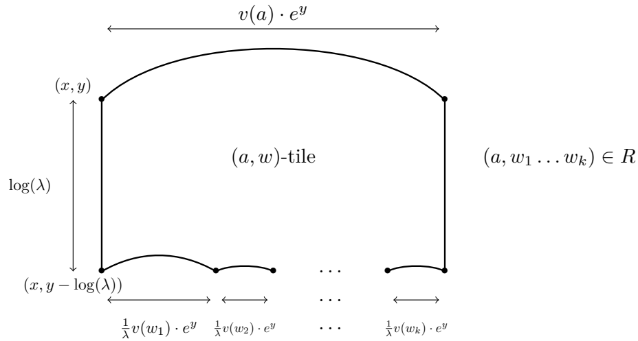
Figure 3.3 – An (a, w) -tile for some production rule (a, w) \in R with w = w_1 \dots w_k .
