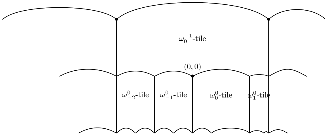
Figure 3.4 – A tiling \Psi_\Omega of an orbit into \mathbb{R}^2 .
