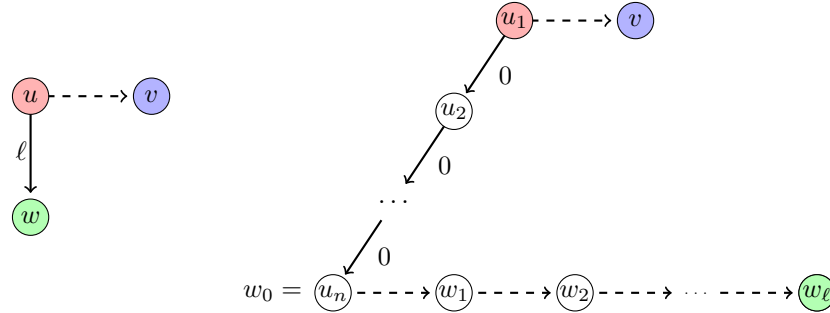
Figure 3.26 – On the left a pattern p \in F_{\mathcal{B}, \Sigma}^n . The corresponding patterns have the support shown on the right and coincide with p in the three colored vertices.
