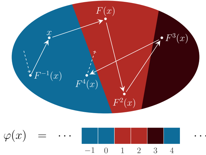
Figure 1 – A partition of X in three sets indexed by colors and the corresponding coding of an orbit.
