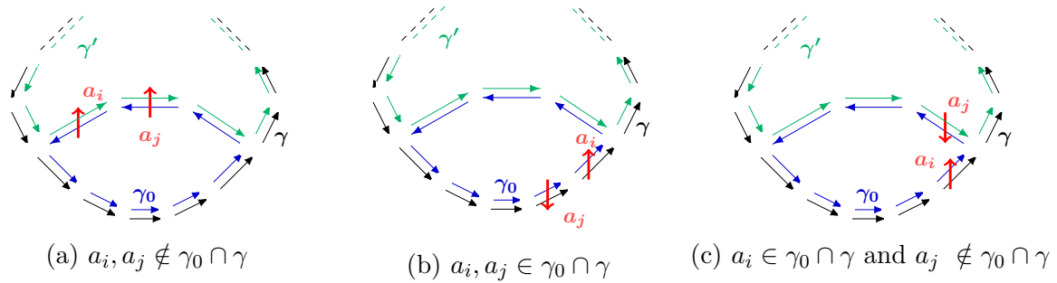
Figure 3.18 – Possible cases for the induction. The cycle \gamma' (in green) is obtained from the cycle \gamma (in black) by deletion of one elementary cycle \gamma_0 (in blue).
