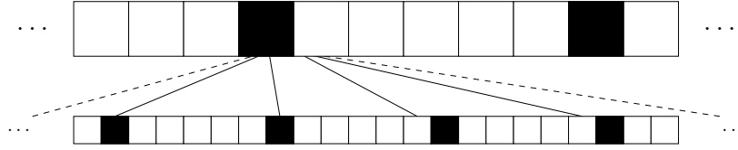
Figure 3.17 – Infinite lines of X .
