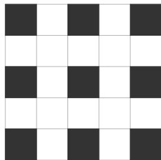
Figure 2.7 – The shape D of low complexity.
