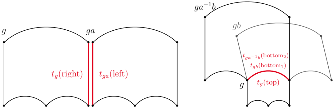
Figure 3.6 – Illustration of the neighbor rules for BS(1,2) .
