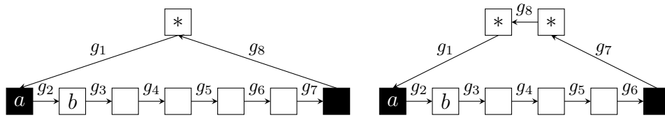
Figure 3.13 – The two possible types of colorings of elementary cycles. There are no color constraints on \boxed{*} , and the cycle g_1 \dots g_8 is any cyclic permutation of [a, b][c, d] .
