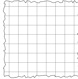
(b) The all white configuration is in \overline{\mathcal{O}(x)} but is not a translation of c .
