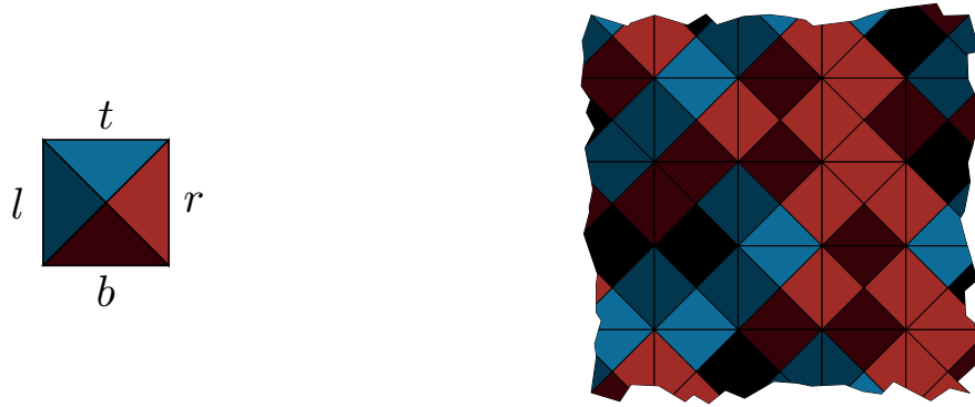
Figure 1.3 – A two-dimensional Wang tile and a portion of valid tiling.
