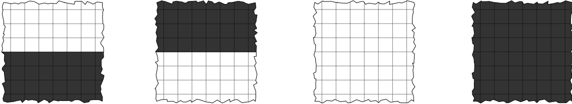
Figure 1.1 – The four types of configurations in X_F defined in Example 1.1.
