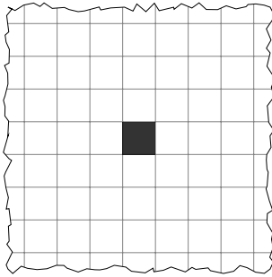
(a) All configurations of \mathcal{O}(x) are shifts of c : they have exactly one black cell.
