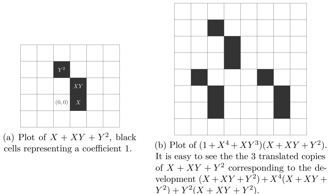
Figure 2.5 – The opposite is also interesting: the configuration gives a way of visualizing a formal series, and by extension any polynomials. Here are two examples for d = 2 .
