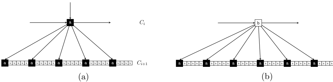
Figure 3.12 – The two types of elements in \mathcal{C}_G and the corresponding sequences of type under them in C_{i+1} .
