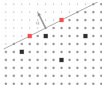
Figure 2.3 – The set of square cells has an outer edge perpendicular to vector \mathbf{u} = (-1, 2) .
