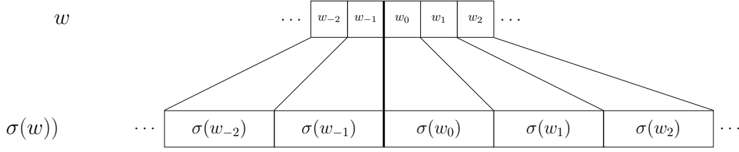
Figure 3.1 – Application of a substitution \sigma to a biinfinte word w .
