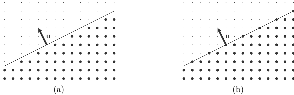
Figure 2.1 – Open (a) and closed (b) discrete half-planes with \mathbf{u} = (-1, 2) .
