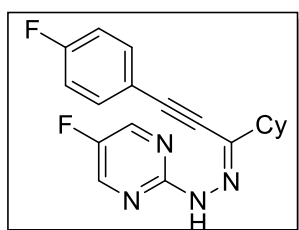
(Z)-2-(2-(1-Cyclohexyl-3-(4-fluorophenyl)prop-2-yn-1-ylidene)hydrazinyl)-5-fluoropyrimidine (93s)
