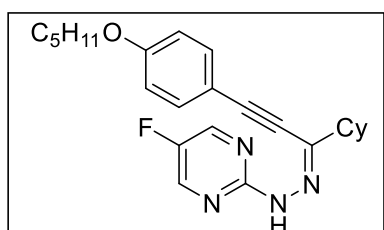
(Z)-2-(2-(1-Cyclohexyl-3-(4-(pentyloxy)phenyl)prop-2-yn-1-ylidene)hydrazinyl)-5-fluoropyrimidine (93u)
