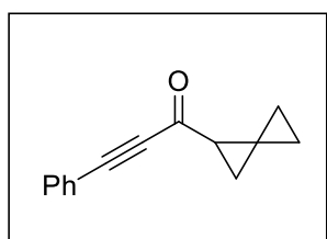
3-Phenyl-1-(spiro[2.2]pentan-1-yl)prop-2-yn-1-one (162x)
