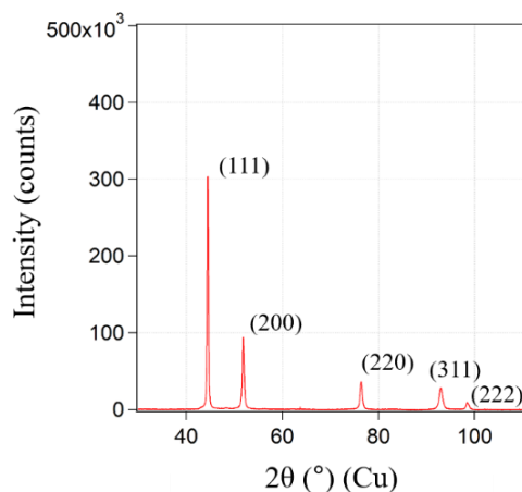
Fig. B-3 Diffractogram corresponding to powder P2.
