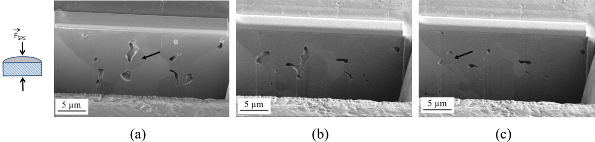
Fig. V-14 SEM images of sample S1 in state E1 after preparation by FIB at three consecutive depths. Arrows indicate two pores that become interconnected.
