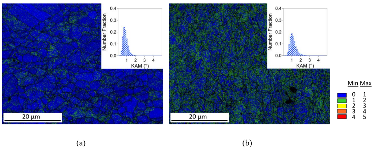
Fig. E-14 First neighbor KAM+IQ cartographies of sample 3 at the initial state (a) and after deformation to failure (b). Color legend represents the kernel average misorientation in ^{\circ} .
