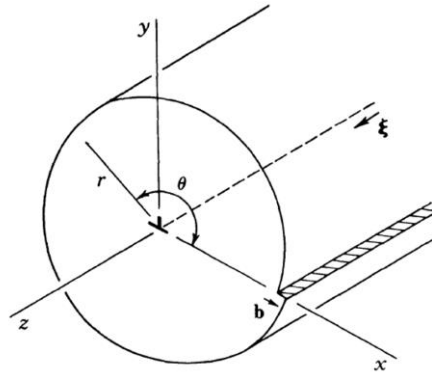
Fig. II-9 Illustration of an edge dislocation [149].
