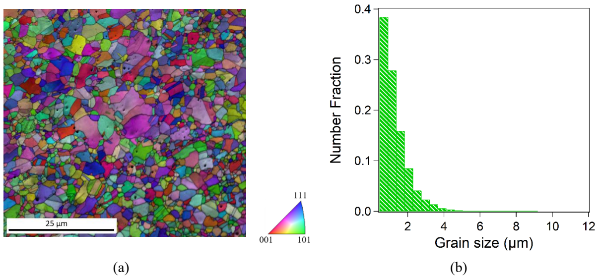
Fig. C-13 Cartography IPF+IQ of sample S-P6 (a) and grain size distribution (b).
