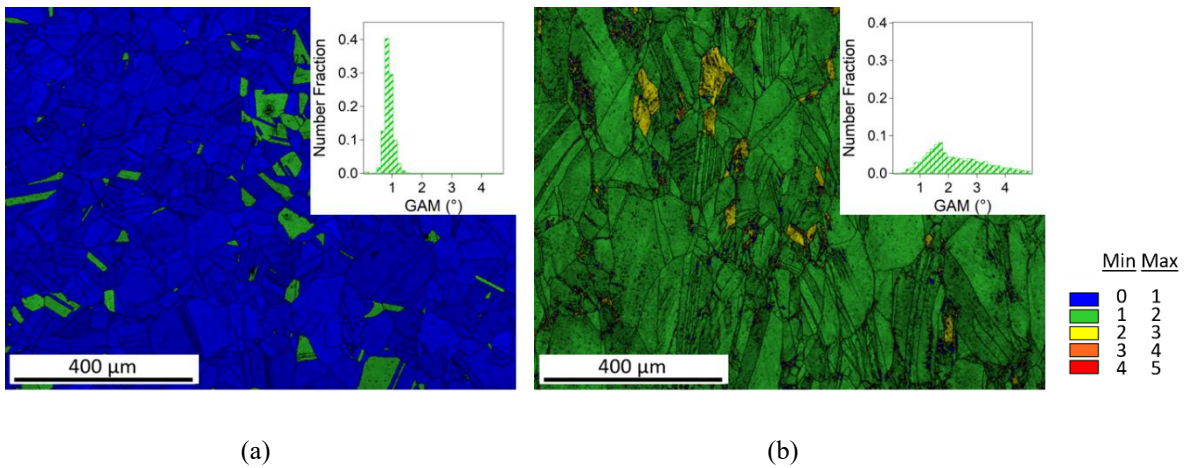
Fig. E-23 GAM+IQ cartographies of sample 4 at the initial state (a) and after deformation to failure (b). Color legend represents the grain average misorientation in ^{\circ} .
