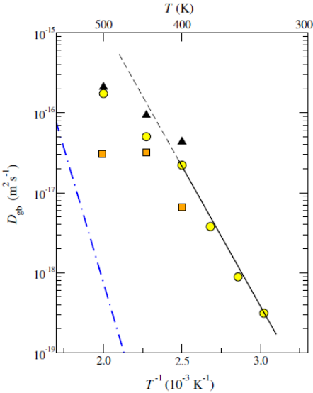
Fig. V-13 Effect of crack formation (black triangles) after subsequent annealing processes on GB diffusion coefficient [125]. The blue dashed line corresponds to annealed coarse-grained Ni with relaxed HAB. Yellow circles represent D_{gb} in the initial state of ECAP Ni and orange squares to D_{gb} of the same samples after the first relaxation annealing.
