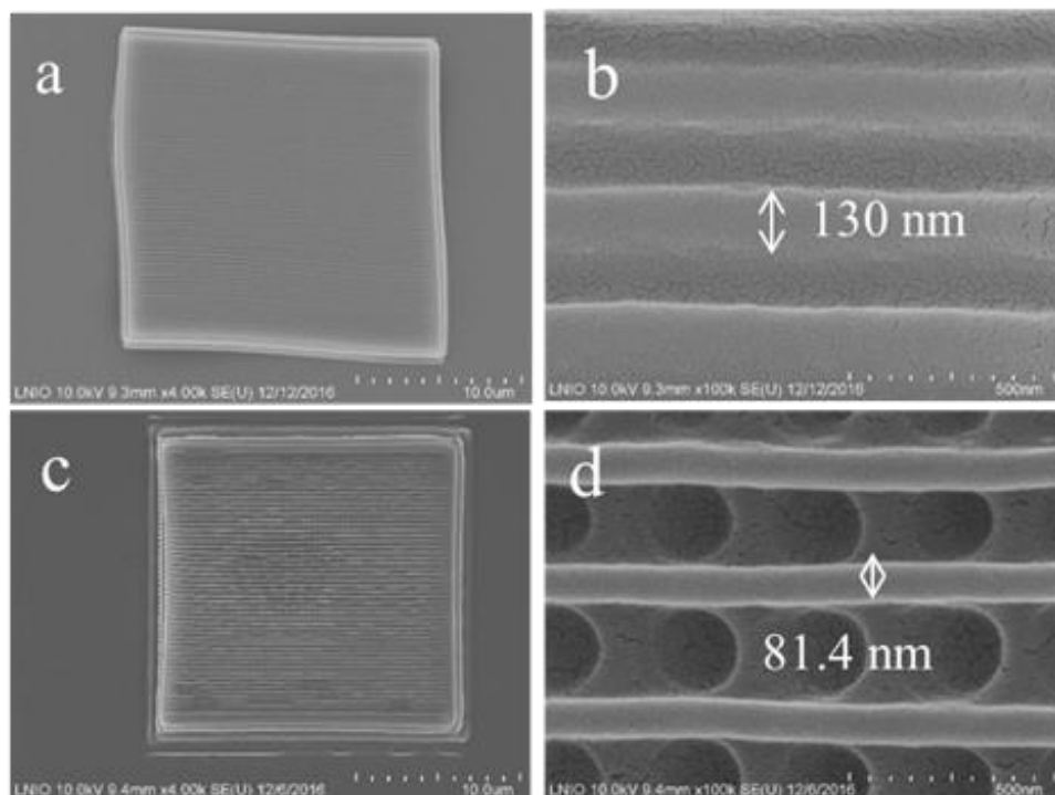
Figure 3.20: SEM images of woodpile in a period of 350 nm fabricated at 8 mW by TPP-DLW in a scanning speed of 100 \mu m/s (a, b) without QDs; (c, d) with QDs.
