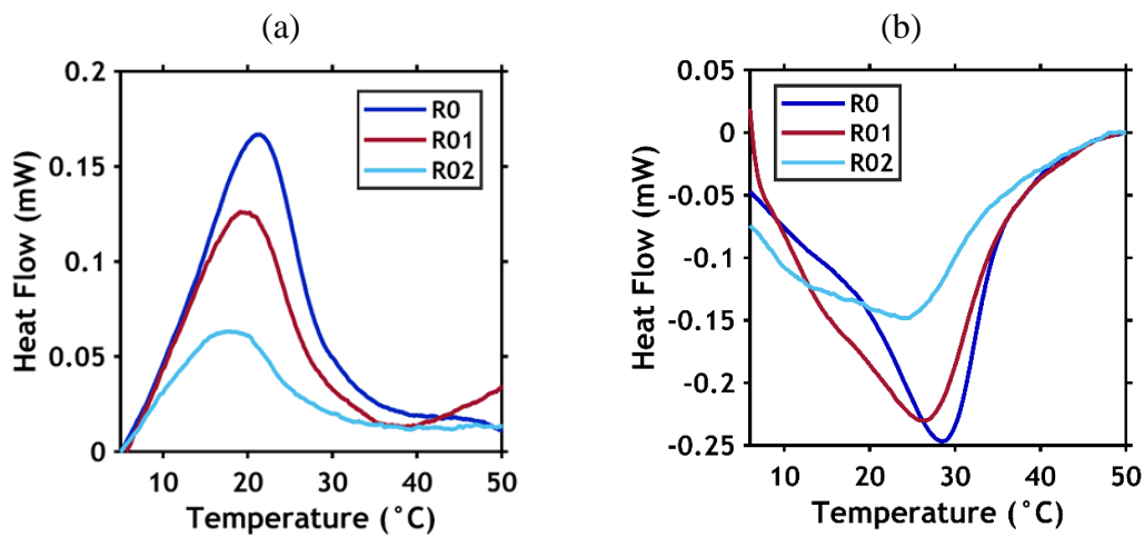
Figure 4-14. Differential Scanning Calorimetry analysis of chemically un-crosslinked and crosslinked Gel A hydrogels when cooling (a) and heating (b) between 5 °C and 50 °C at a scanning rate of 2^{\circ}\text{C}/\text{min} .
