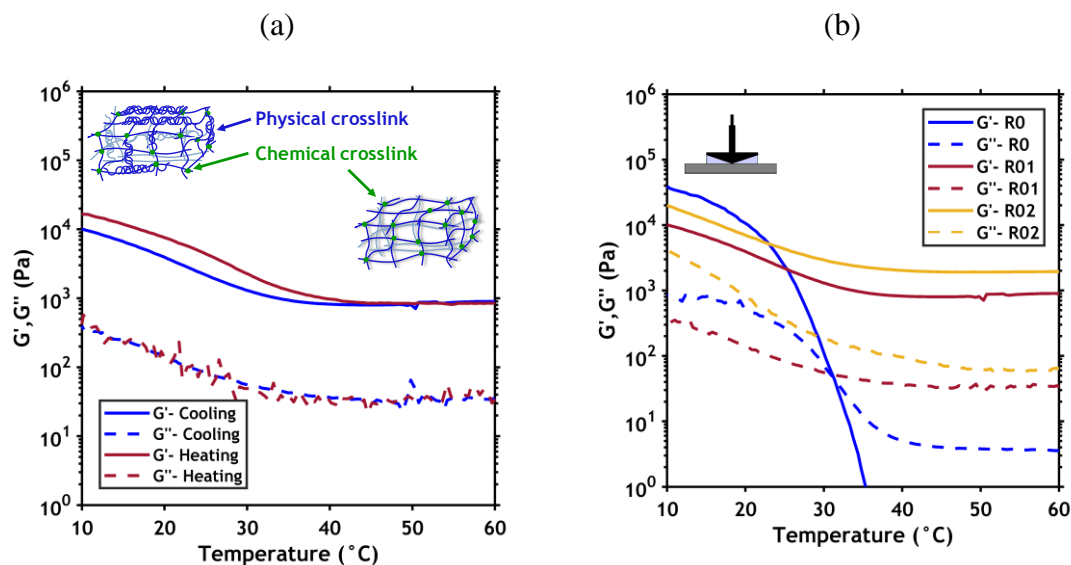
Figure 4-16. (a) Cooling and heating temperature sweep of dual-crosslinked Gelatin A hydrogel R01. (b) Linear rheology of a cooling temperature sweep from 60°C to 10°C of non-chemically crosslinked (R0) and chemically crosslinked Gelatin A hydrogels (R01 and R02) at preparation state (Gel A concentration: 20 wt%). Cone-plate geometry.
