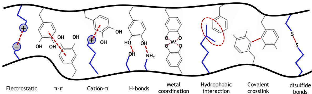
Figure 1-3. Overview of some of the different adhesive and cohesive interactions as found or hypothesized for wet adhesion by sandcastle worms and mussels. There are more interactions such as hydrophobic, disulfide bonds, metal coordination and covalent crosslinks. 32
