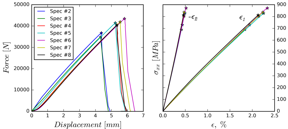
Figure B.3: Force-displacement and stress-strain \sigma_{xx} results of tensile tests on [0^\circ]_8 specimens.
