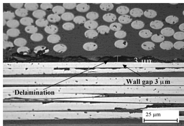
Figure 1.5: Delamination between two differently oriented composite laminae [28].
