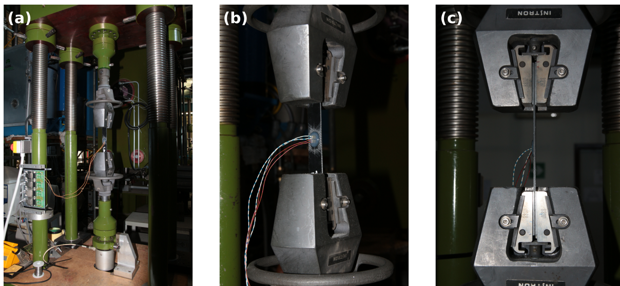
Figure B.1: Tensile testing apparatus used for 0° and 90° tensile tests and \pm 45 in-plane shear tests. Global view (a) and close-up views from different angles (b-c).
