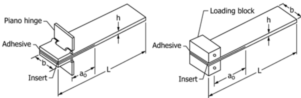
Figure 3.2: Representation of the DCB specimen with piano hinges or loading blocks [49].
