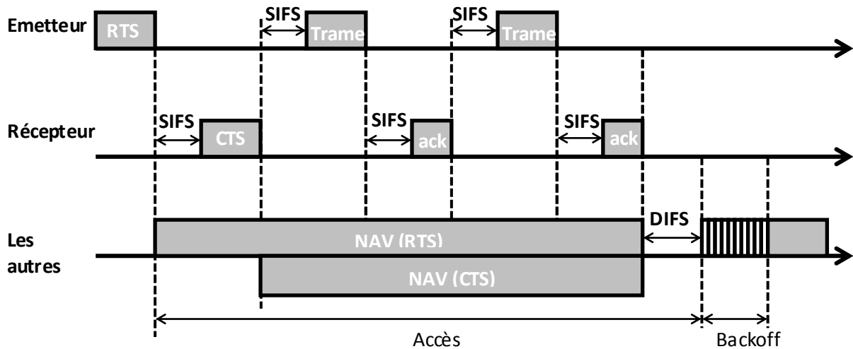
Figure 9 : Protocole DCF
