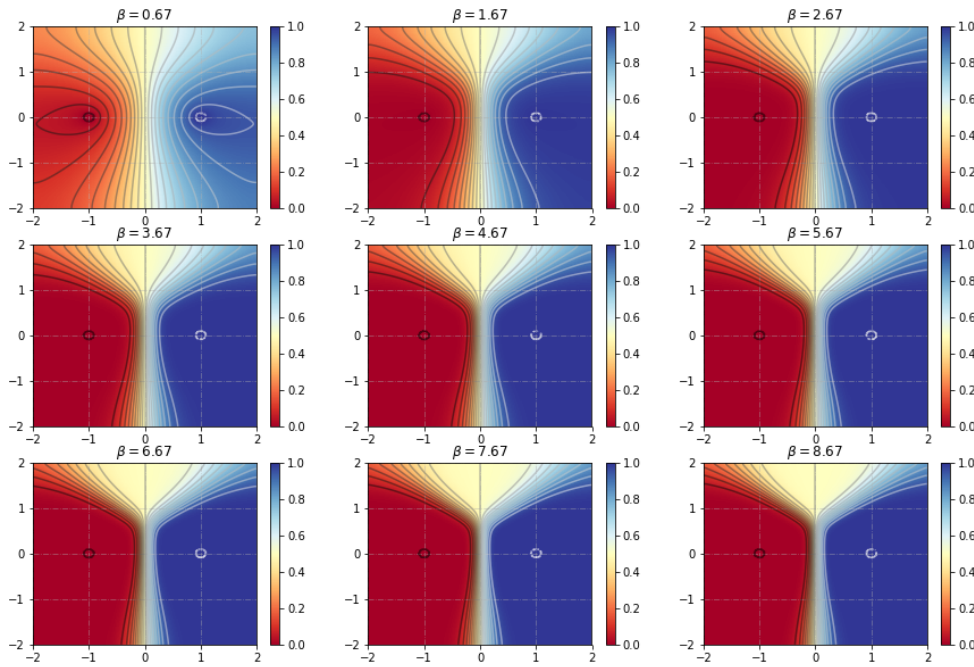
Figure 4.16: Illustrations of committor functions for different temperatures.
