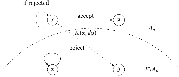
Figure 1.3: The construction of a P_{A_n} -invariant kernel.
