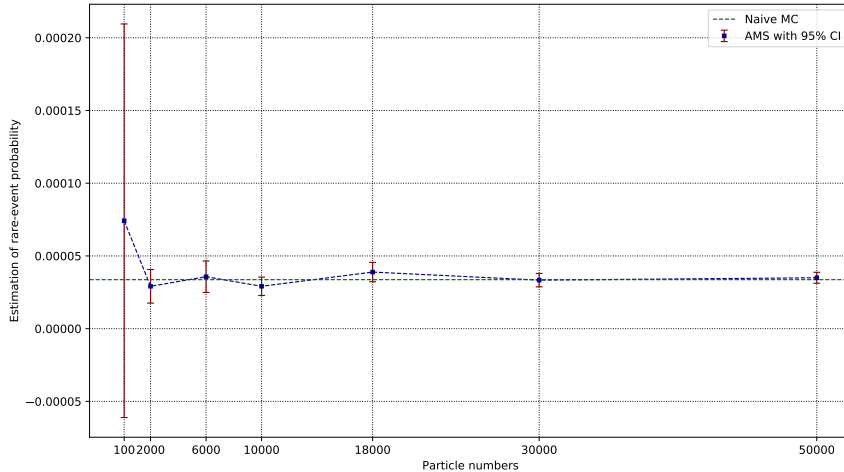
Figure A.1: An illustration for the estimation of AMS method along with 95% confidential interval. The number of particles N varies from 100 to 50000 and \iota = 0.01 .
