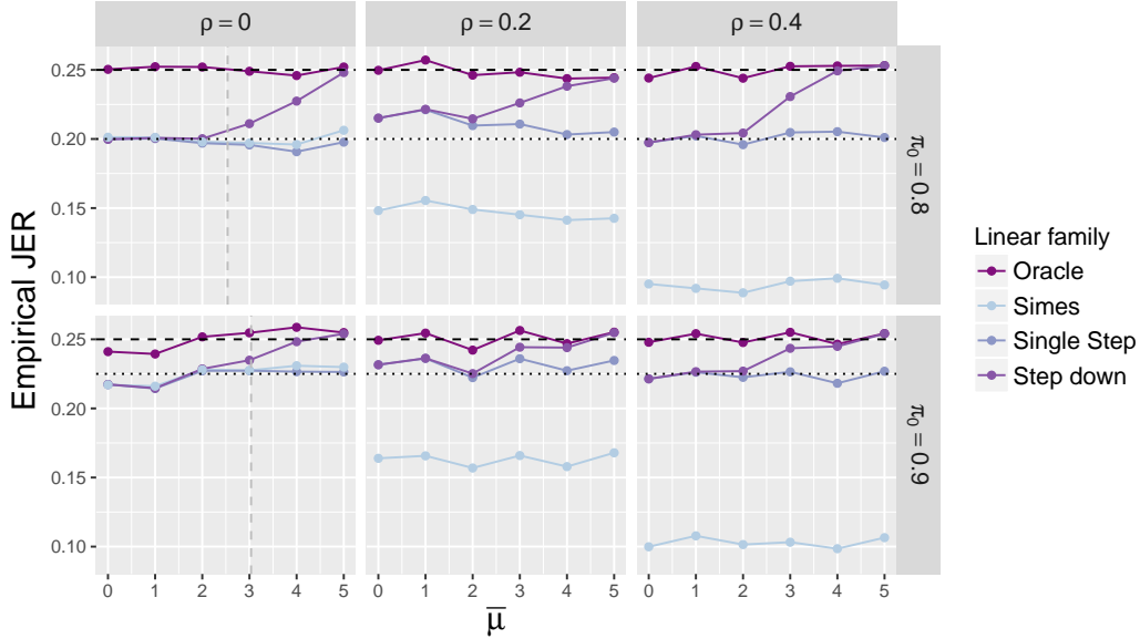
Figure 5.5: JER control based on the linear template for equi-correlated test statistics: \lambda -calibration by sign-flipping in the location model.
