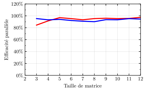
(b) EPYC
