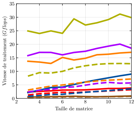
(a) HSW
