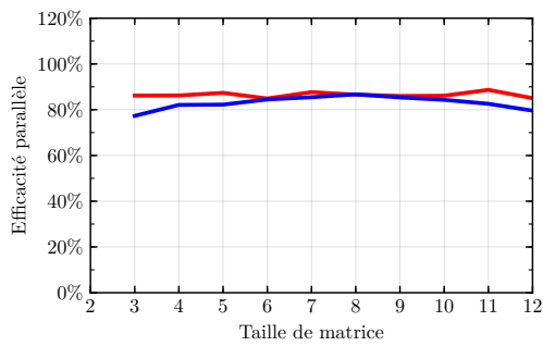
(e) A72
