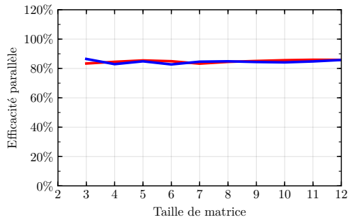
(a) HSW
