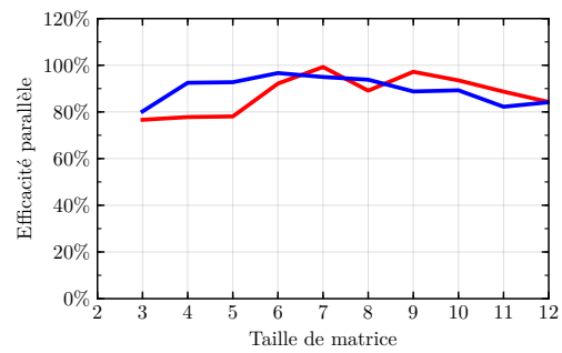
(f) Power8
