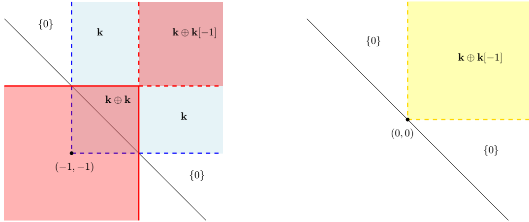
Figure 4.3 – On the left, the value of the MV system \mathcal{L}_*(f) where the blue part is a birth block and the red part are a death block and its dual. On the right, the value of the MV system \mathcal{L}_*(p) where the yellow part refers to the (reunion of) two birthblocks. The dashed lines pictures boundary which are not inside the blocks.
