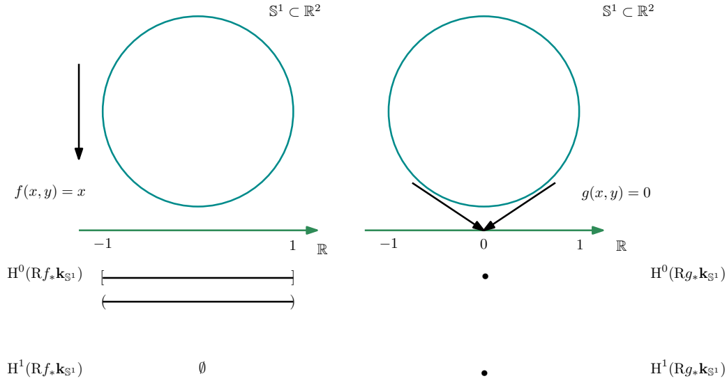
Figure 3.1 – The maps f and g and the graded-barcodes of Rf_*\mathbf{k}_X and Rg_*\mathbf{k}_X .
