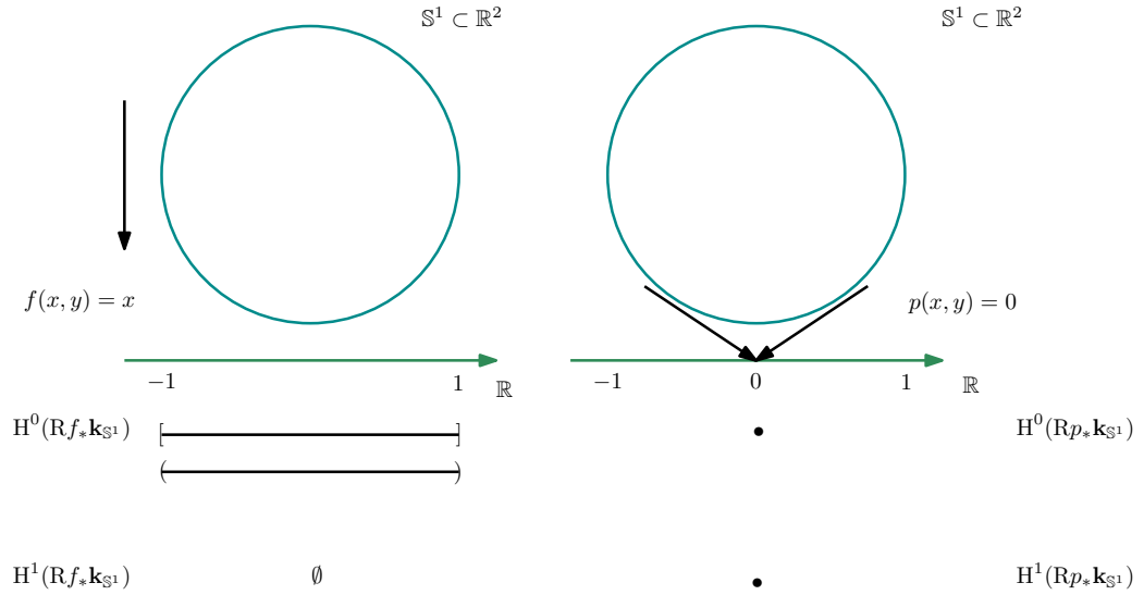
Figure 4.2 – The map f and p together with the intervals on which are supported the degree 0 and 1 part of the associated sheaves, see (4.37) and proposition 4.5.1.
