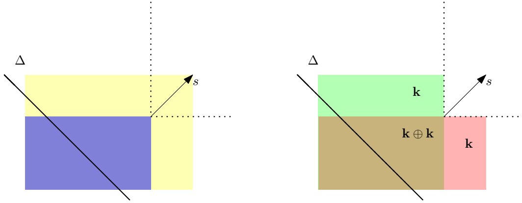
Figure 4.1 – On the left: A deathblock B in yellow (and blue) and the translated deathblock B - s = B[s] in blue where s is the vector drawn. The dotted lines are the boundary of the dual birth block B^\dagger[s] . On the right: The value of \mathbf{k}^B[s_x] \oplus \mathbf{k}^B[s_y] in every region where the green region is the translated death block B - s_x , the red is the translated death block B - s_y . The value is 0 on the white region and below the antidiagonal.
