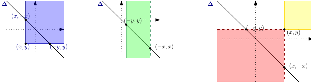
Figure 2.1 – On the left a block of type \mathbf{bb}^- pictured in blue. On the middle a block of type \mathbf{vb} pictured in green. On the right a block of type \mathbf{db} in red and its dual block of type \mathbf{bb}^+ in yellow. The various coordinates refers to the intersection points of the boundaries of the blocks with the anti-diagonal \Delta as well as the extremum of the birth or death blocks. The dashed boundary lines means that the boundary line is not part of the block.
