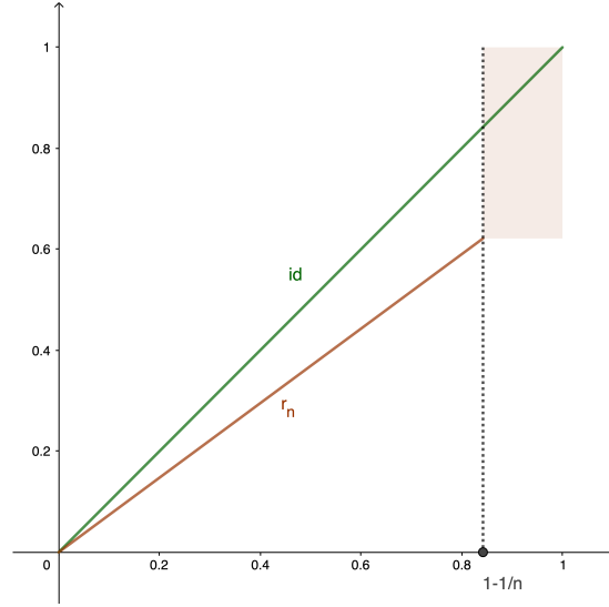
Figure 3.2 – Graphical representation of r_n
