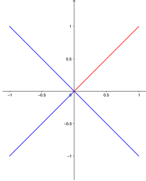
Figure 2.2 – The topological space X in \mathbb{R}^2 and its subset X' in red.
