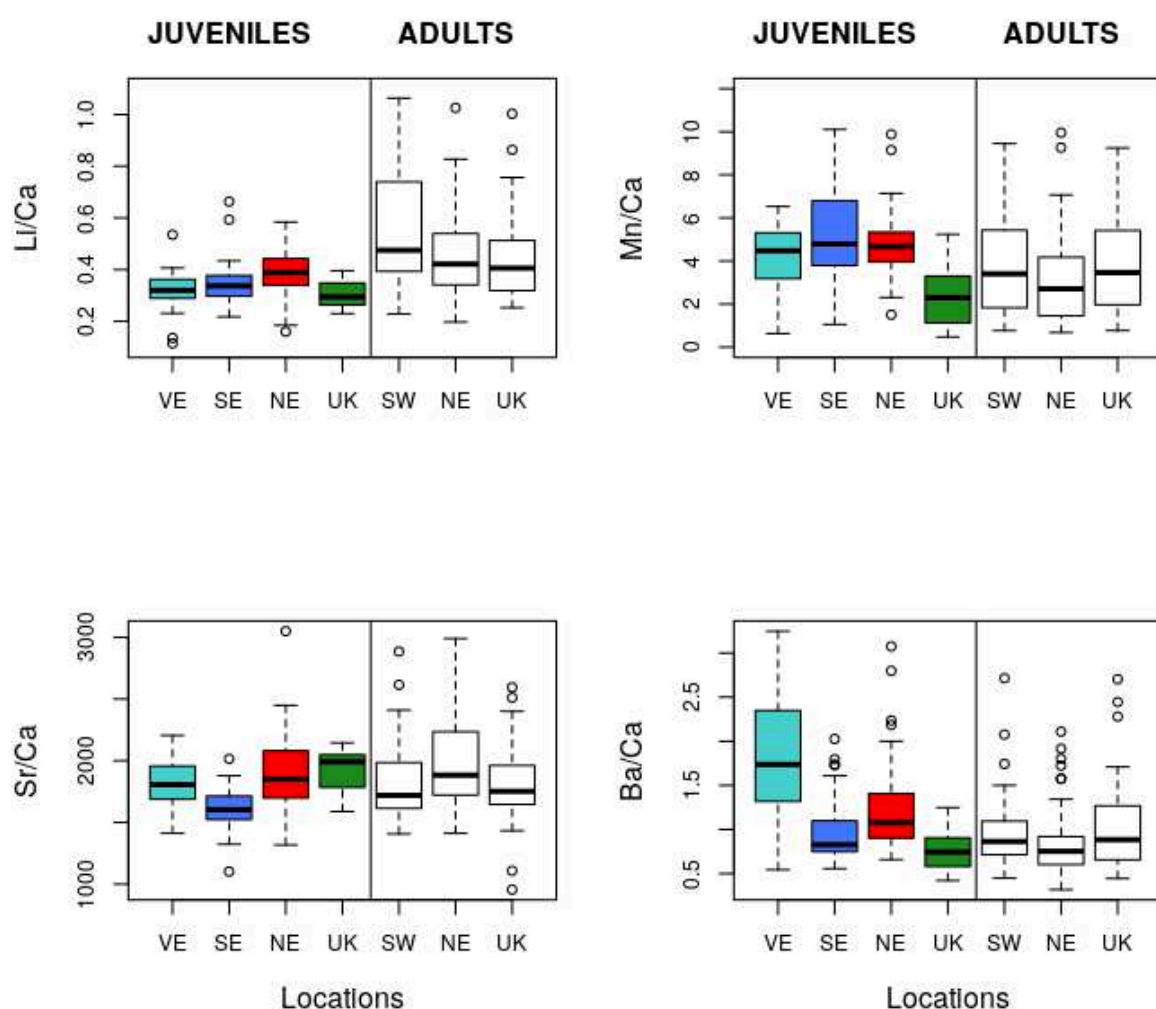
Figure. C.2. Juvenile (i.e. nursery) elemental concentrations in ratio Ca ( \mu\text{g.g}^{-1} ) of juvenile and adult soles at each location of the EEC.
