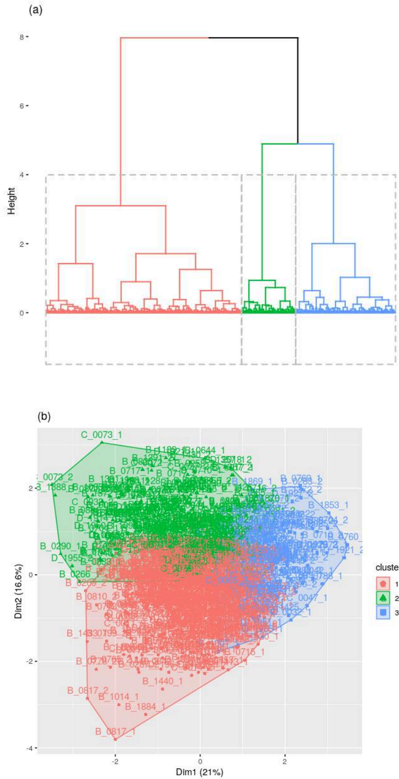
Figure. B.5. (a) Dendrogram and (b) principal components scatterplot of hierarchical clustering analysis on residual matrix ( S' ) of EFDs.
