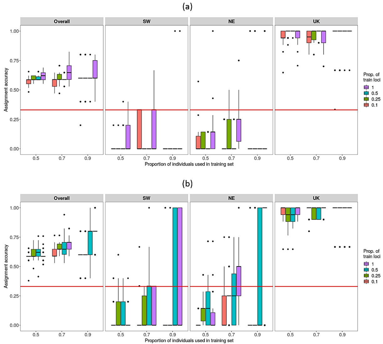
Figure. 3.5. Assignment accuracy estimates performed by Monte Carlo cross-validation and support vector machine methods using (a) only genetic and (b) genetic, otolith shape and microchemistry datasets. Training datasets were composed of four proportions of training loci (top 10% in orange, 25% in green and 50% in blue of the highest F_{ST} loci and all loci in purple), four shape indices and four otoliths elemental measurements. Three subsets of the datasets were considered for training (0.5%, 0.7% and 0.9%) and 30 iterations were computed. The horizontal red line represented the null subunit assignment rate (0.33 in the case of three subunits).
