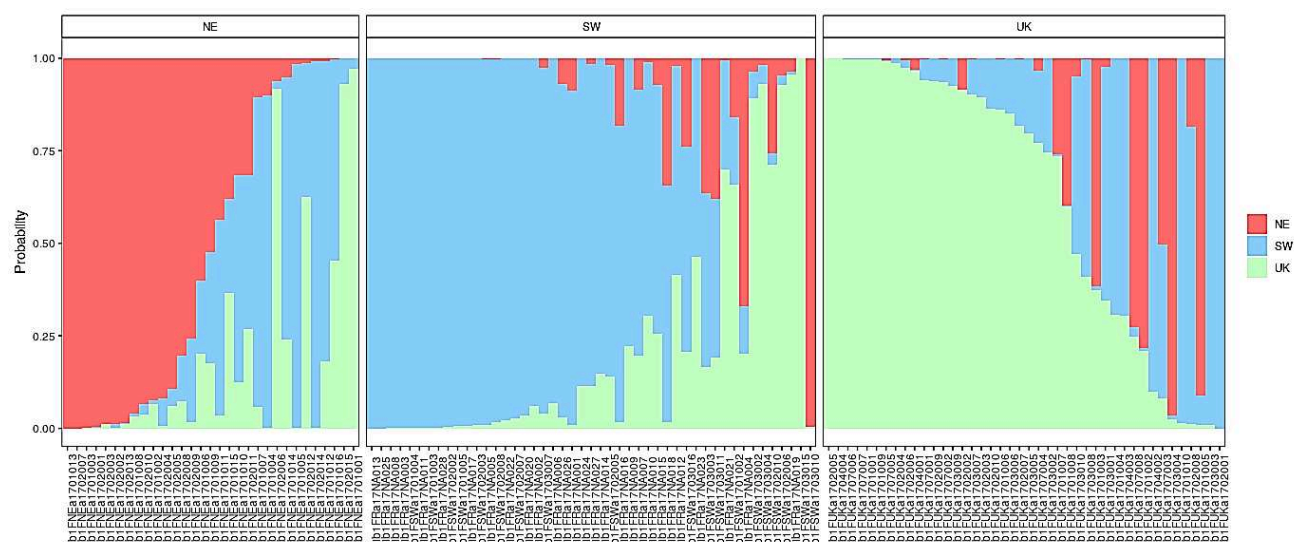
Figure. A.2. Probabilities of reallocation of individuals in the three subunits using only the SNP genotypes of 2017. Panels correspond to the subunits where individuals were sampled. Probabilities were estimated using the K-fold cross-validation method ( K = 3 ) and all loci (2302 SNPs).
