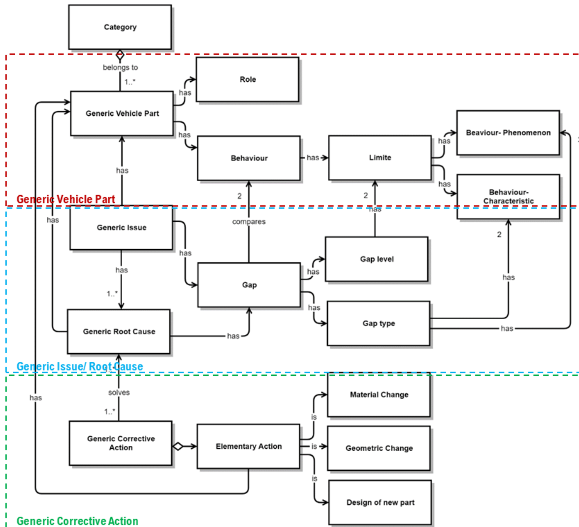
Figure 5: The reasoning level of the CSPP Ontology
