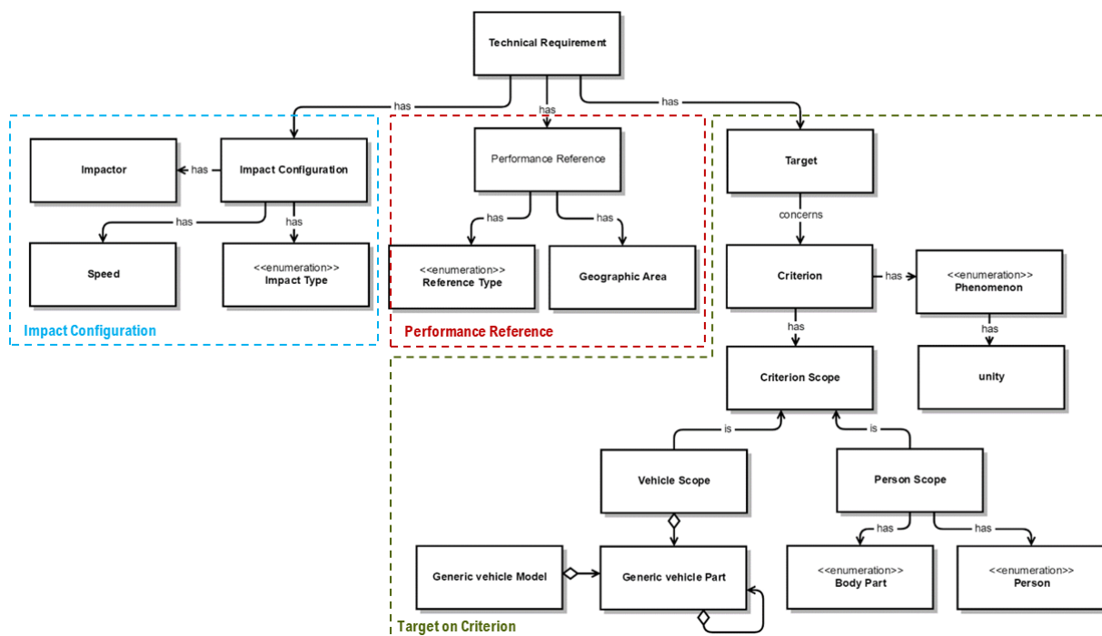
Figure 3: The context level of the CSPP Ontology
