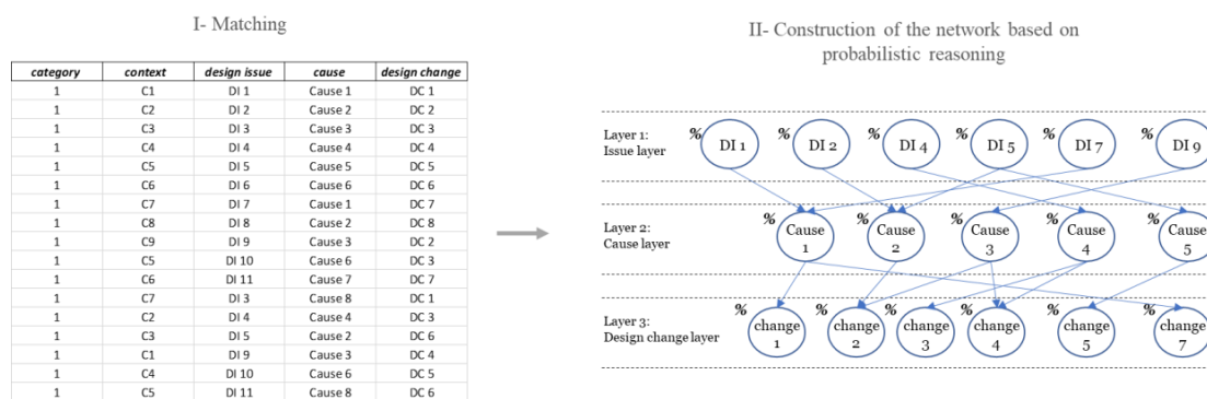
Figure 4.10 (I) presents the list of design issues and their resolution that results from the matching algorithm. (II) explains the construction of the network, where design issues (DIs) are presented with their respective causes and design changes, and the % represents the probability of each node.
