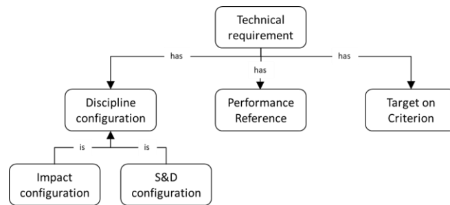
Figure 4.14 Simplification of the context level of a generic ontology. Since configuration concepts depend on the simulation discipline, the concept "Discipline Configuration" would group different configurations such as the impact configuration for crash simulation and the S&D configuration for S&D simulation. The configuration could be multiplied according to the disciplines considered in the vehicle development.
