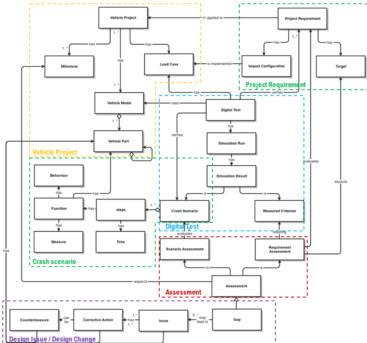
Figure 4: The Project level of the CSPP Ontology
