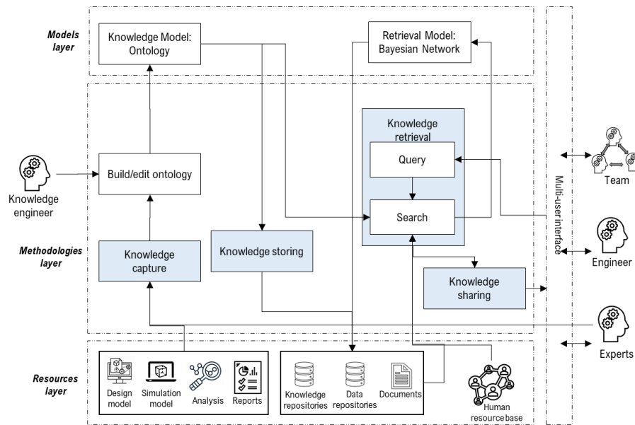
Figure 4.8 A proposal, in Paper 4, of an ontology-based knowledge management system architecture to support simulation-aided design. The support system consists of 3 layers and a multi-user interface (MUI). The resources layer refers to the repositories of different types of knowledge and the human resource base. The methodologies layer represents the methodologies used to carry out KM activities. The models layer consists of the models developed to ensure the implementation of the system.
