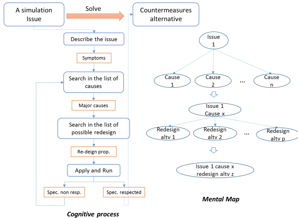
Figure 3. Cognitive Process and resulting Mental Map
