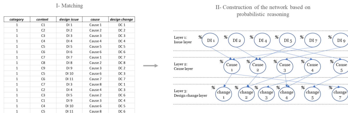
Figure 5: (I) presents the list of design issues and their resolution that is the result of the matching algorithm for the design issue under study. (II) explains the construction of the network, where some design issues (DIs) are presented with their respective causes and design changes. The % represents the probability of each node, which is calculated based on a statistical calculation of occurrence from part (I).
