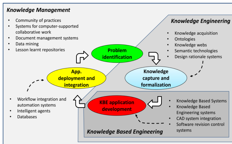
Figure 2.1 The explanation of the complementarity between knowledge management, knowledge engineering and knowledge-based engineering, from (La Rocca, 2012).
