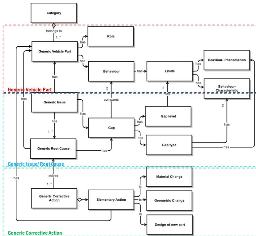
Figure 4.7 The reasoning level of the CSPP ontology
