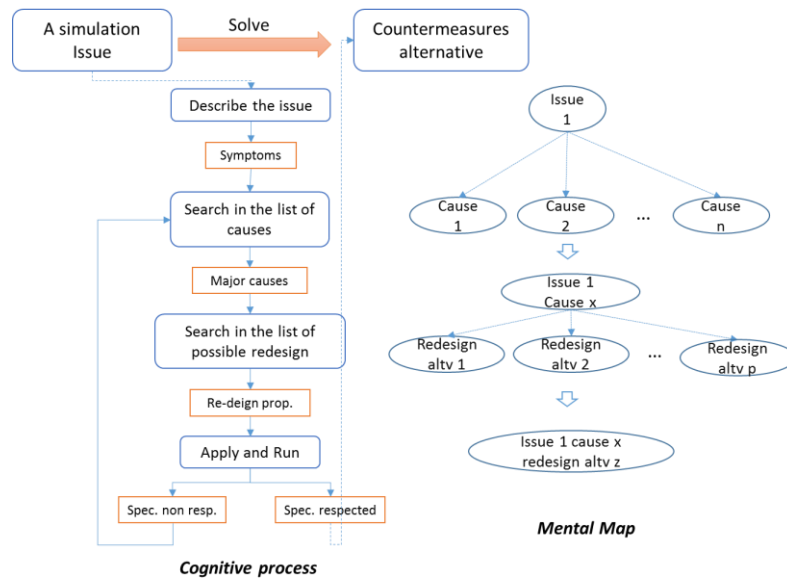
Figure 4.2 The developed cognitive process and its resulting mental map presented in Paper 1. The cognitive process describes the activities that analysts execute when facing a design issue. The mental map describe how issues are related to their causes and then to the design changes. Each design issue has a limited list of root causes, and for each root cause, a limited list of possible design changes is considered.
