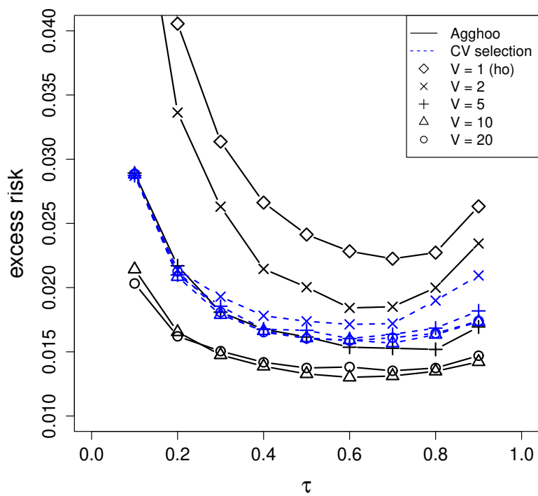
Figure 3.3: Classification performance of Agghoo and CV for the k -NN family
