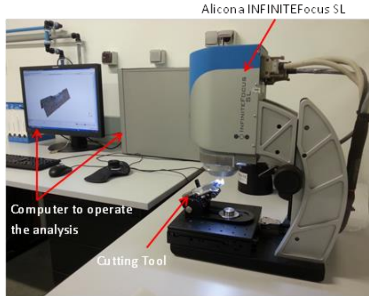
Fig. 4.2.2: Alicona INFINITEFocus SL to measure tool sharpness
