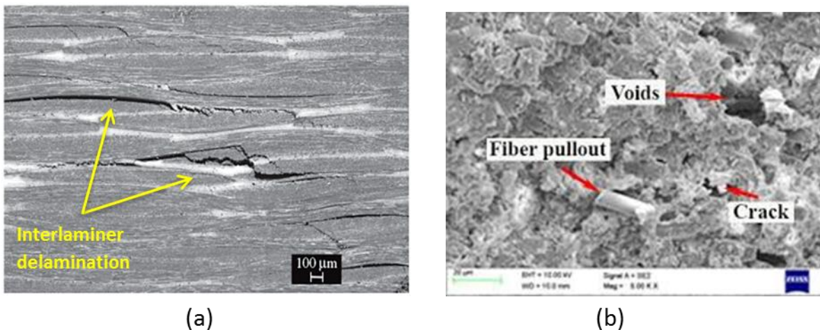
Fig. 1.III: Generated defects in CFRP machining; (a) interlaminar delamination [Paiva et al., 2005] and (b) crack and voids [Vijayan et al., 2018]
