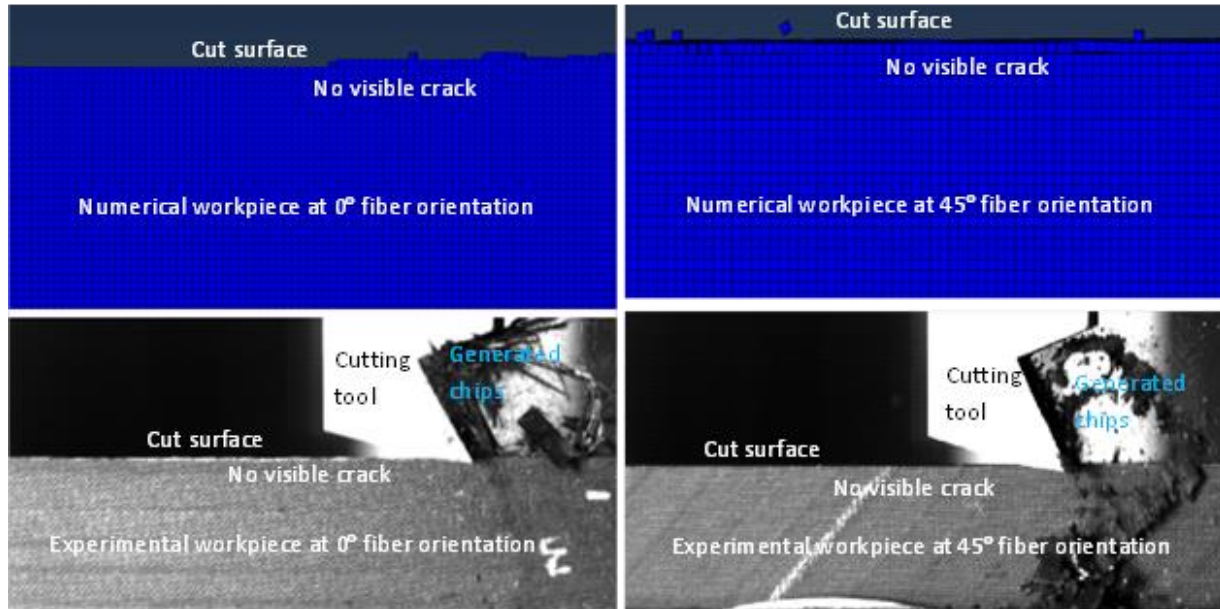
Fig. 3.4.1: Numerical and experimental surface state at (a) 0° and (b) 45° fiber orientation.
