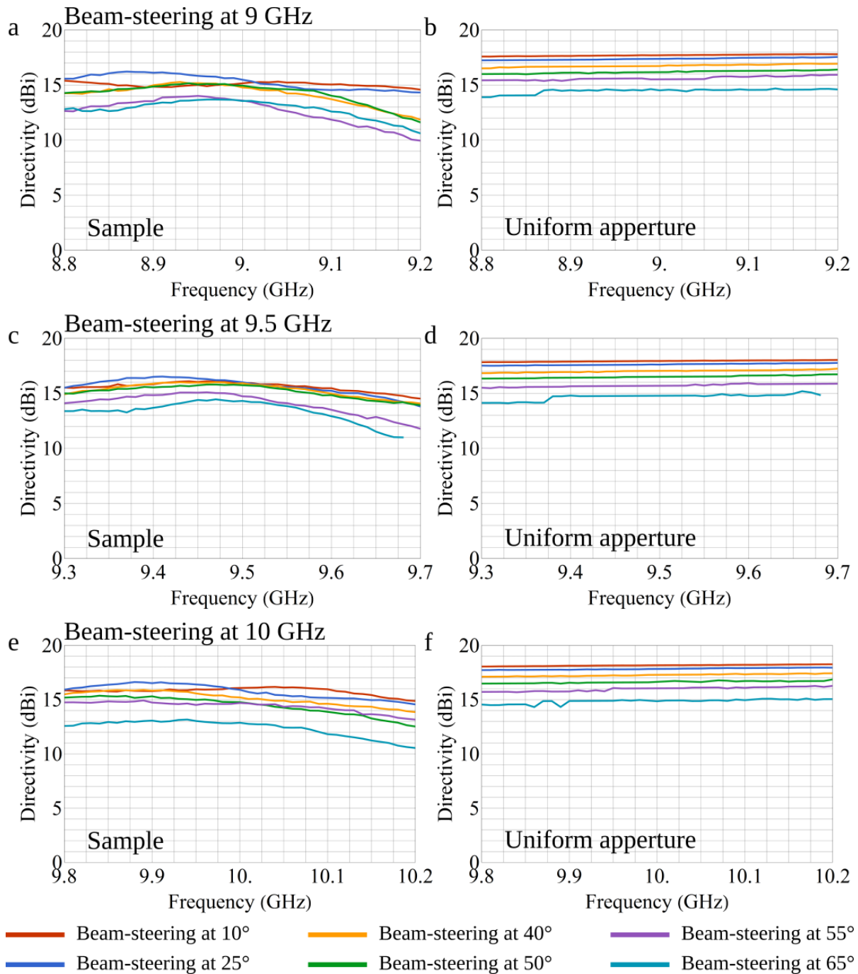
Figure 5.15: Calculated 2D directivity of the radiation patterns created by the sample in different configurations compared to the corresponding directivity of a uniform aperture. The panels (a), (c), (e) correspond to the sample and the panels (b), (d), (f) correspond to the uniform aperture. The panels (a) and (b) correspond to the panel (a) of Fig. 5.12, the panels (c) and (d) correspond to the panel (b) of Fig. 5.12 and the panels (e) and (f) correspond to the panel (c) of Fig. 5.12. The color code corresponds to the one of Figs. 5.12(a)–(c).
