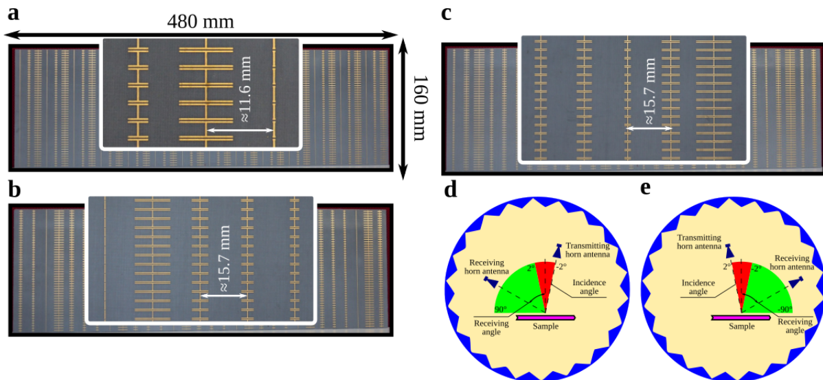
Figure 3.11: (a)–(c) Photograph of the first, second and third samples (from top to bottom, respectively). (d), (e) Schematics of the experimental setup: to measure the scattering range of angles from -90^\circ to 90^\circ the experiment is performed in the two steps illustrated by figures (d) and (e).
