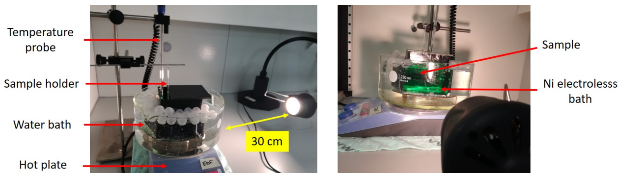
Figure 5.4: Experimental setup used to assess the impact of illumination on Ni electroless deposition.
