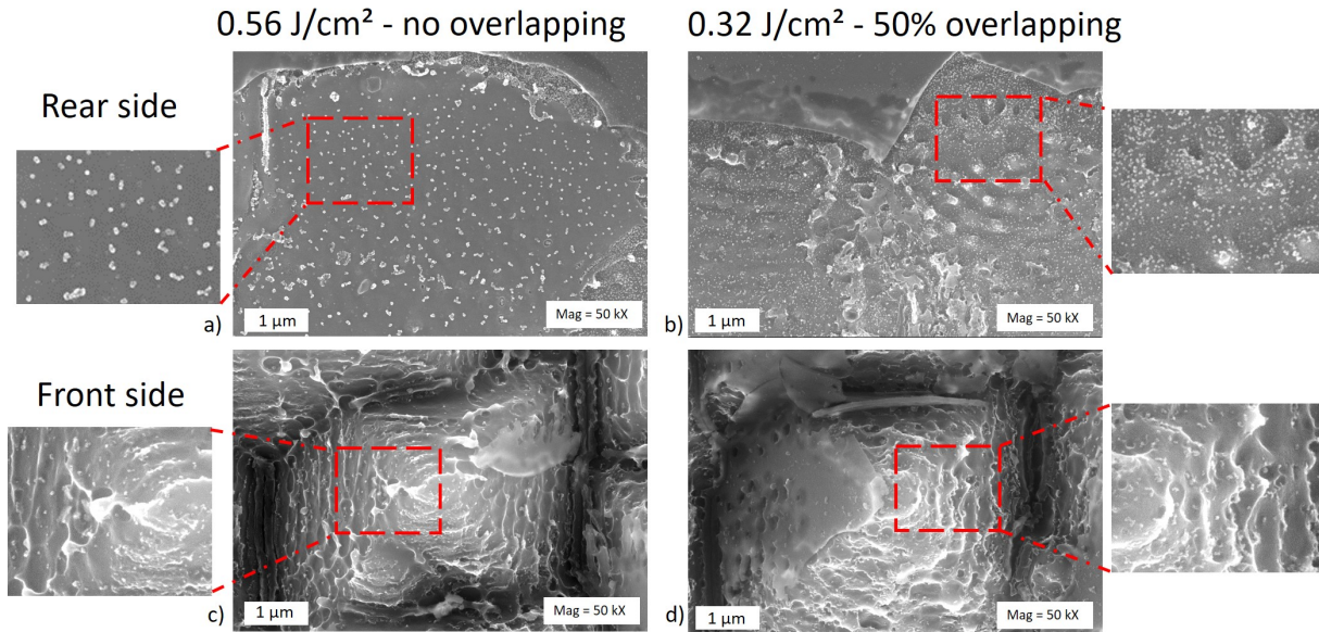
Figure 4.50: SEM images after deoxidation in \text{NaHF}_2 0.16 M 1 min 30 and activation in \text{NaHF}_2 0.16M + \text{PdSO}_4 5.10^{-5} M 30 sec on rear and front sides for both optimized laser parameters.
