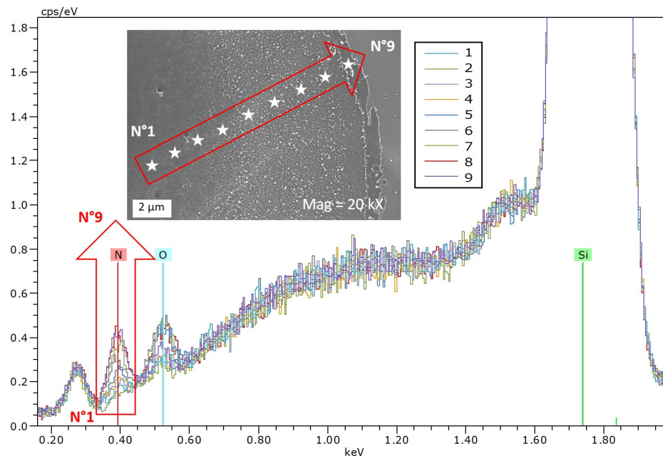
Figure 3.29: EDS spectra on laser ablated sample with Si-rich \text{SiO}_x\text{N}_y layer using F_{peak} = 10.50 \text{ J/cm}^2 .
