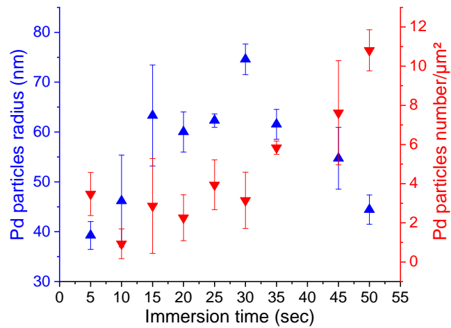
Figure 4.32: Evolution of Pd particles number and mean radius with immersion time in HF 0.5 M + \text{PdSO}_4 5.10^{-4} M (no stirring).
