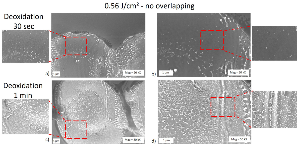
Figure 4.49: SEM images on rear side opened with laser 1 after deoxidation in \text{NaHF}_2 0.5 M 30 seconds (a and b) or 1 minute (c and d) followed by immersion in \text{NaHF}_2 0.16 M + \text{PdSO}_4 2.5 \cdot 10^{-4} M during 30 sec.
