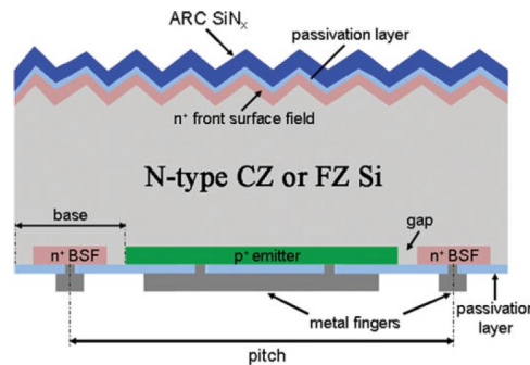
Figure 1.21: Illustration of IBC structure of c-Si solar cell [37].
