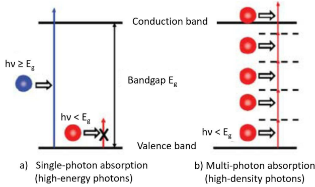
Figure 3.2: Illustration of photon absorption through a) single-photon absorption when E_{ph} \geq E_g , b) multi-photon absorption in case of high photon flux with E_{ph} \leq E_g [149].
