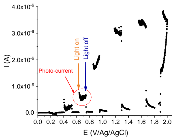
Figure 4.14: Evolution of the photo-current with the applied potential on n-type bare Si.
