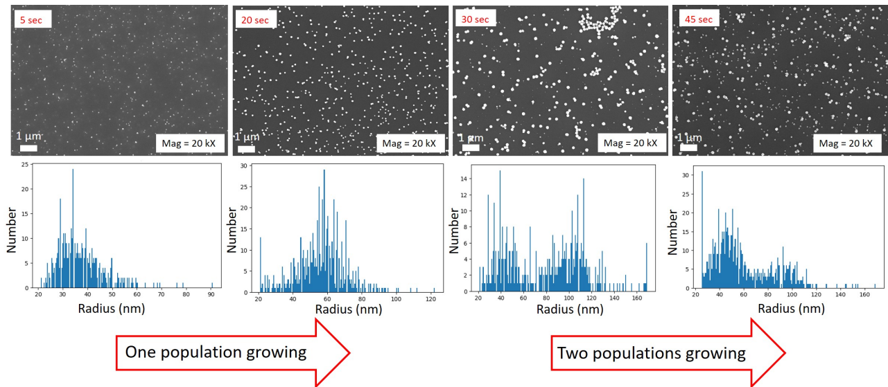
Figure 4.33: SEM images and Pd particles radius dispersion after 5, 20, 30, 45 seconds immersion in HF 0.5 M + \text{PdSO}_4 5.10^{-4} M (no stirring).
