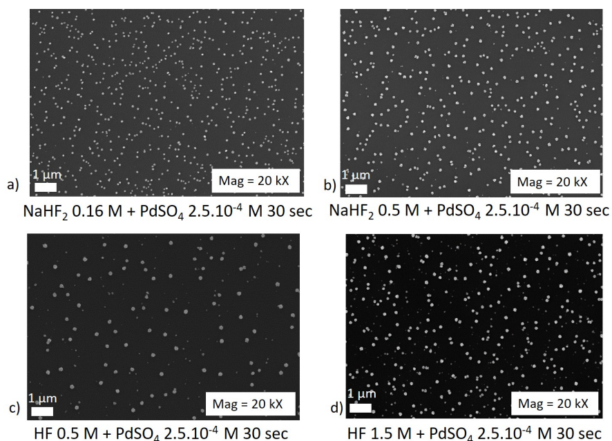
Figure 4.46: SEM images after 30 seconds in \text{PdSO}_4 2.5 \cdot 10^{-4} M + a) \text{NaHF}_2 0.16 M, b) \text{NaHF}_2 0.5 M, c) HF 0.5 M, d) HF 1.5 M (with stirring).
