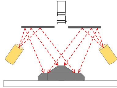
Figure 3.5: Diffuse lighting
