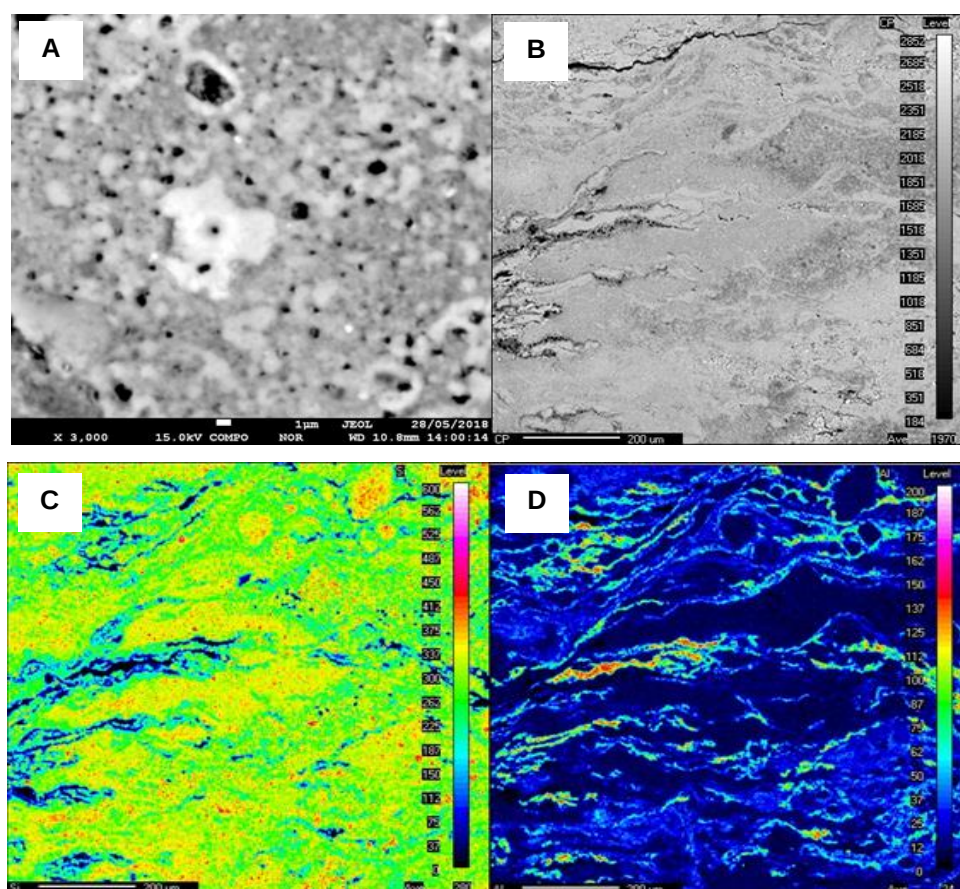
Figure 29: SEM image coupled with microprobe of Catal_ref at two different scales: A) clear visualisation of two different phases of \text{Al}_2\text{O}_3 and \text{SiO}_2 ; B) morphology of the catalyst at 200 μm; mapping of the Si (C) and Al (D) elements present in Catal_ref
