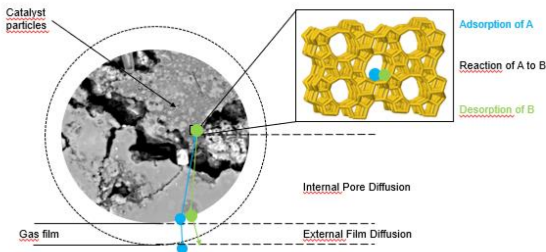
Figure 13: Mass transfer and reaction steps for a catalyst particle
