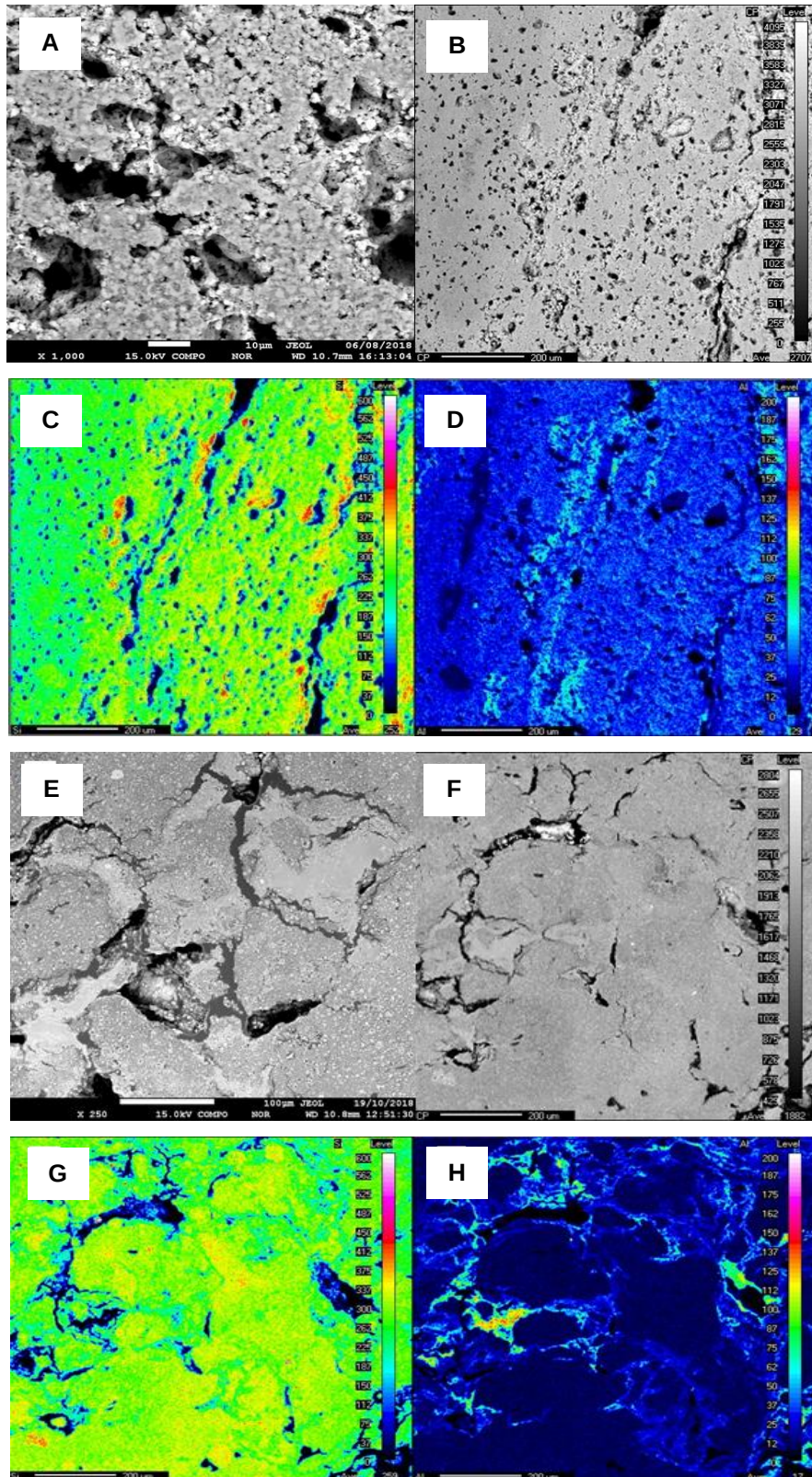
Figure 30: A) clear visualization of macropores in Catal_10Propyl; B) morphology of Catal_10Propyl at 200 μm; mapping of the (C) Si and (D) Al elements present in Catal_10Propyl; (E) clear visualization of macropores in Catal_P123; (F) morphology of Catal_P123 at 200 μm; mapping of the (G) Si and (H) Al elements present in Catal_P123
