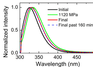
Fig. 6. Normalized emission spectra for native BChE, measured before the pressure cycle (black), at 1120 MPa (green), immediately after pressure release from 1120 MPa (red), and after additional waiting time of 160 min (dashed blue line overlapping with the solid red line). The spectra are deformed in the short-wavelength range below about 305 nm due to the excitation cut-off filter used.
