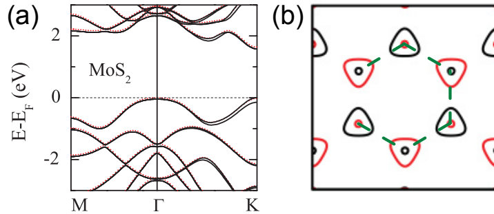
Figure 1.4: Electronic structures of monolayer MoS 2 by DFT calculations of Ref. [25]. (a) Band structure with (black line) and without (dotted red line) spin-orbit interaction. The monolayer MoS 2 has a direct band gap at K point. (b) Energy contour of spin-split hole pocket pairs for a binding energy of 0.8 eV. Electron spin orientations and BZ, which is consistent with Figure 1.3, are indicated by black and red colors, and dashed green line, respectively. Reprint from Ref. [25]. Copyright (2011) American Physical Society.
