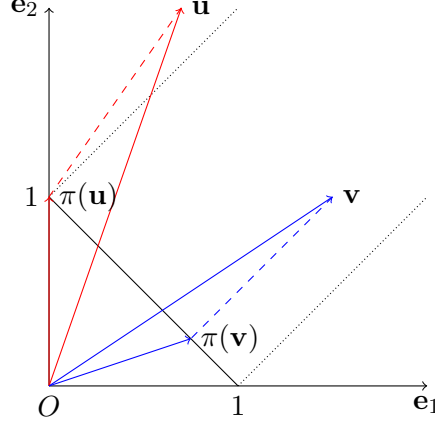
Figure 2.2: The Euclidean projection onto the simplex \mathbb{S}_+^1 .
