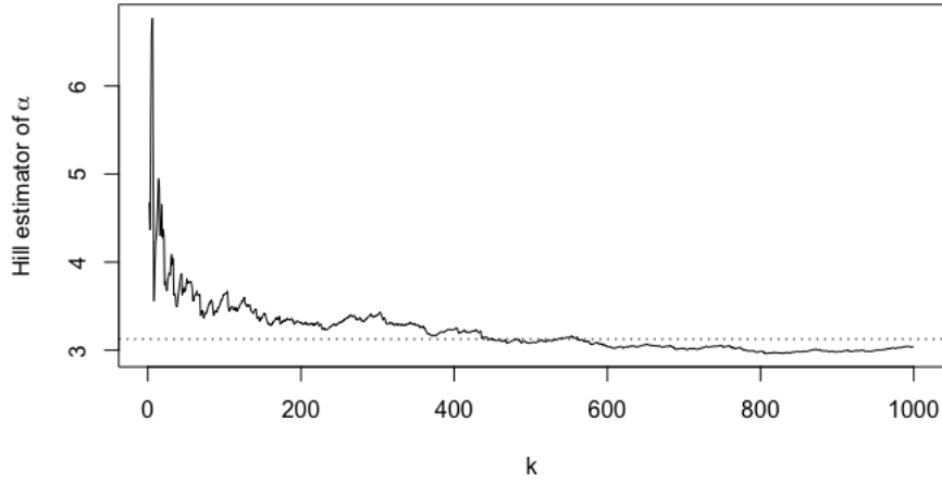
Figure 3.8: Evolution of the Hill estimator \hat{\alpha} .
