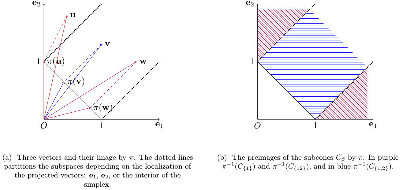
Figure 3.2: Euclidean projection onto the simplex \mathbb{S}_+^1 .
