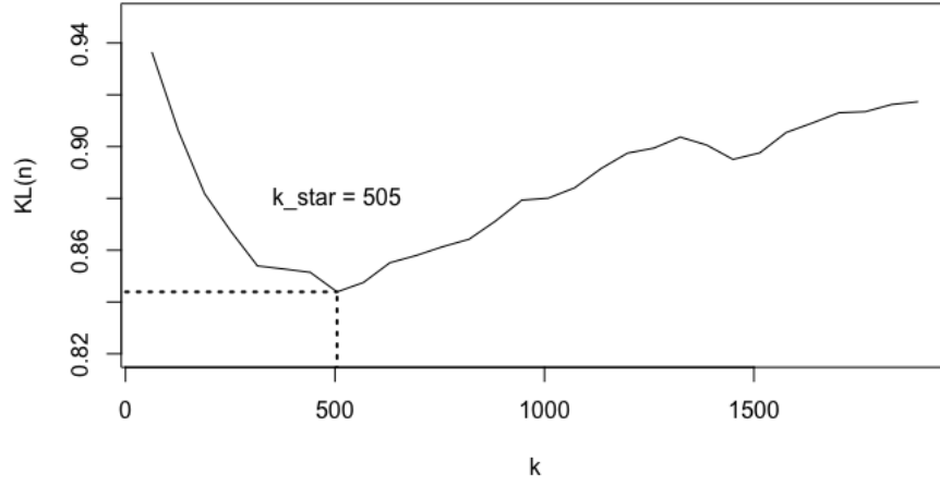
Figure 3.9: Evolution of the estimator of KL(\mathbf{P}_n \| \mathbf{M}(n; \tilde{\mathbf{p}}')) .
