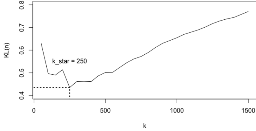
Figure 3.6: Evolution of the estimator of KL(\mathbf{P}_n \parallel \mathbf{M}(n; \tilde{\mathbf{p}}')) in a dependent case.
