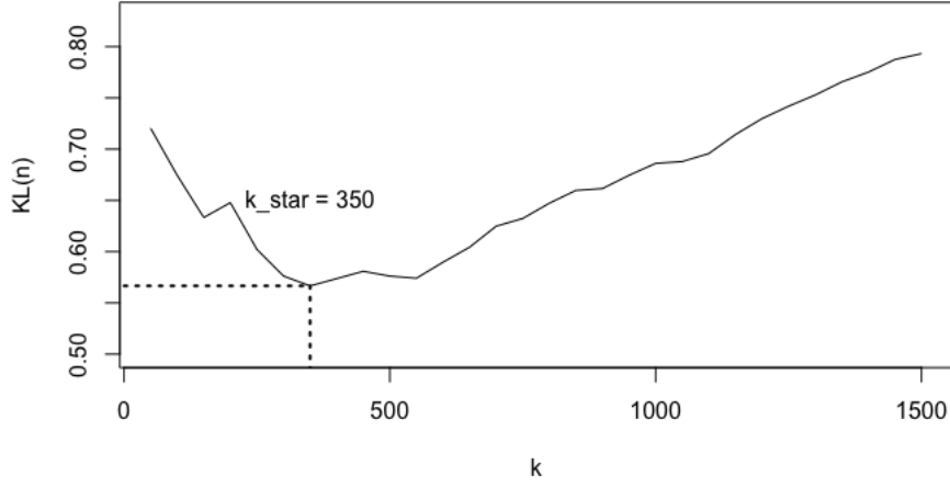
Figure 3.4: Evolution of the estimator of KL(\mathbf{P}_n \parallel \mathbf{M}(n; \tilde{\mathbf{p}}')) in an independent case.
