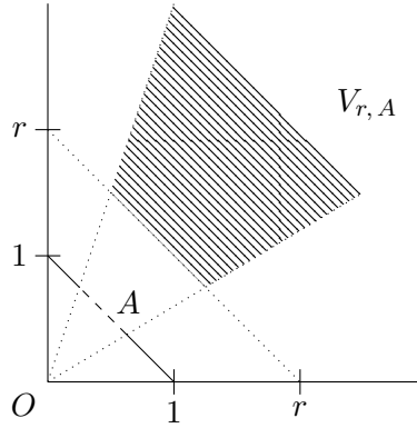
Figure 1.2: Illustration of the sets V_{r,A} .
