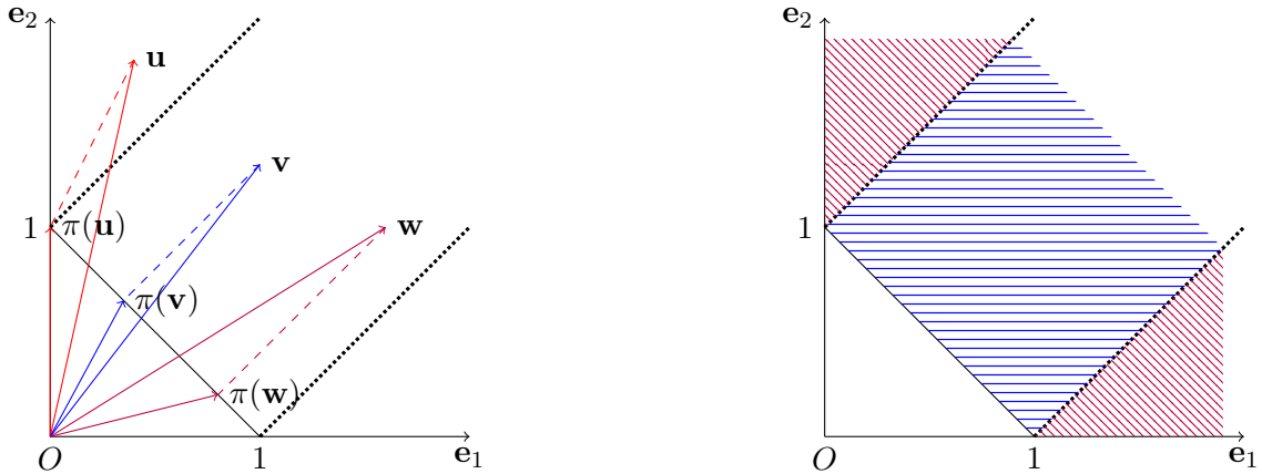
(a) Three vectors and their image by \pi . The dotted lines partitions the subspaces depending on the localization of the projected vectors: \mathbf{e}_1 , \mathbf{e}_2 , or the interior of the simplex.
