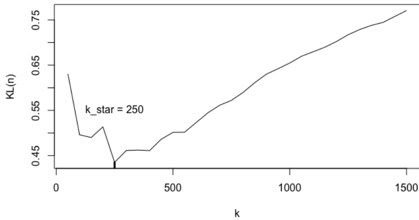
Figure 3.6: Evolution of the minimizer of KL(n) in a dependent case.
