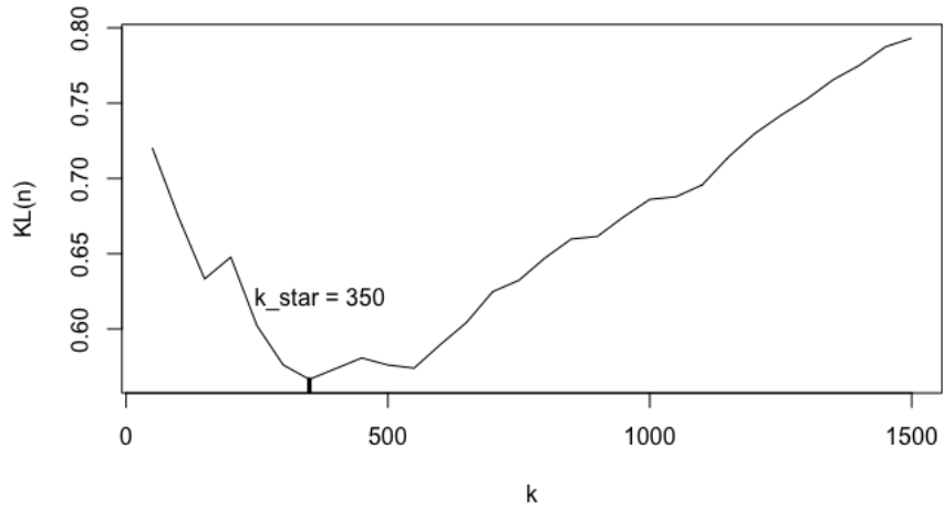
Figure 3.4: Evolution of the minimizer of KL(n) in an independent case.
