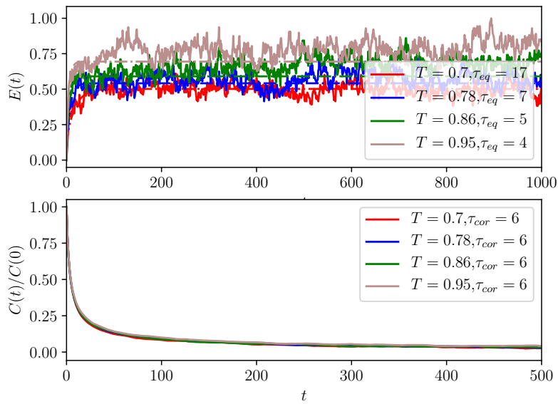
Figure 2.2: Plot of the energy per site (top) and the autocorrelation function (bottom) with Glauber dynamics from an initial state where h_i = 0 , for different temperatures.
