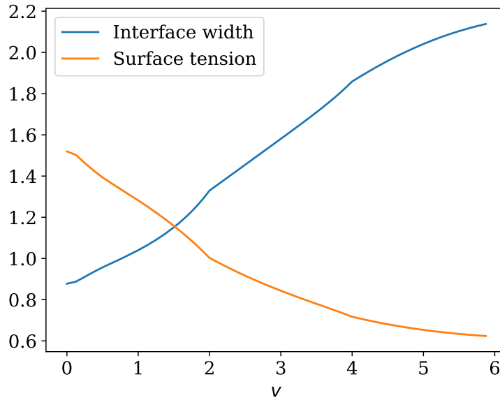
Figure 5.4: Interface width w = \sqrt{\langle h^2 \rangle - \langle h \rangle^2} and surface tension \sigma computed from the integral (5.66) with respect to the drive \nu , with L' = 256 , L = 200 , \langle h \rangle = 4.5 , and \beta = J = 1 for 5 \cdot 10^7 MC steps.
