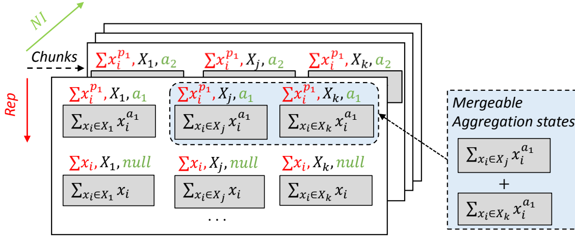
FIGURE 4.3: SUDAF cache.
