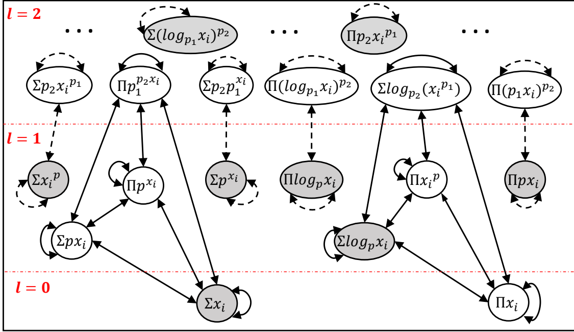
FIGURE 4.1: The digraph G of \text{saggs}_2(X) .
