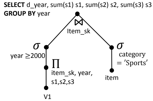
FIGURE 3.8: Plan of the subquery of RQ3'.
