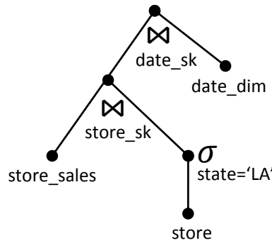
FIGURE 3.3: Plan of the query Q1.
