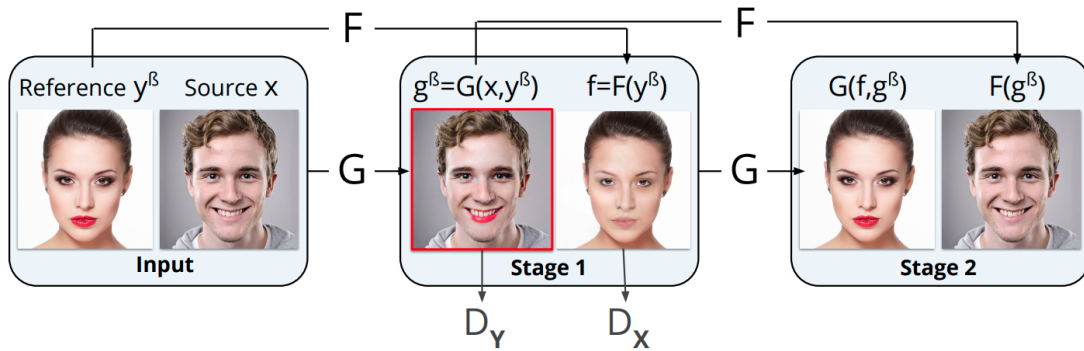
FIGURE 2.16: Pipeline of the method proposed in [Chang et al., 2018].
