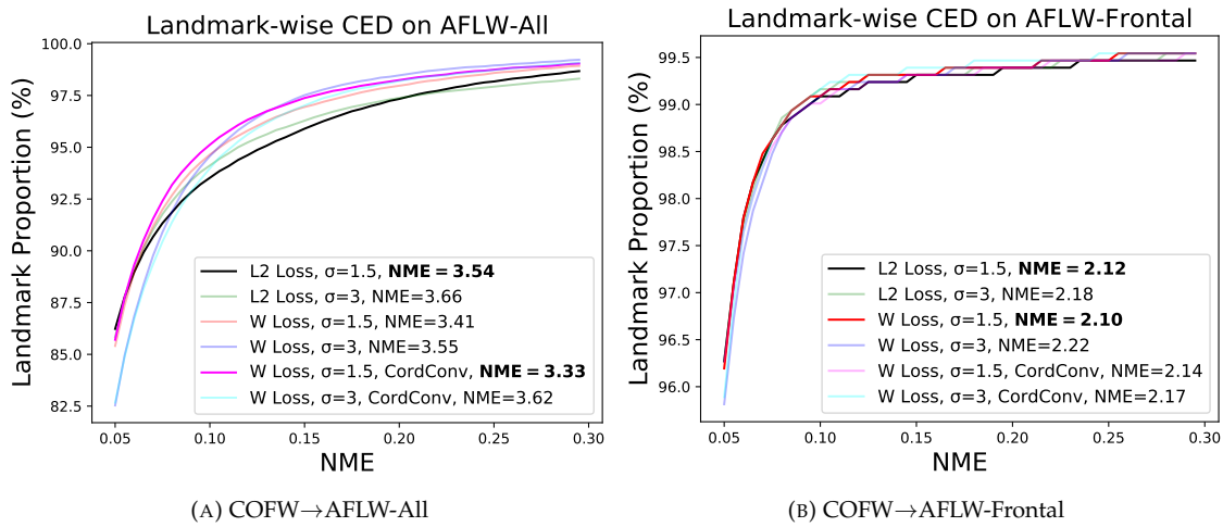
FIGURE 4.8: Landmark-wise CED of COFW→AFLW cross-dataset validation using HRNet.
