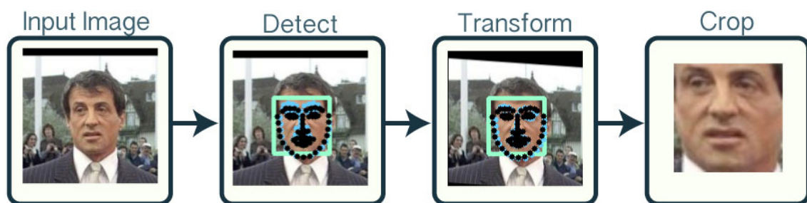
FIGURE 1.8: A standard pre-processing pipeline of face recognition. This figure is adopted from Open Face [Amos et al., 2016].
