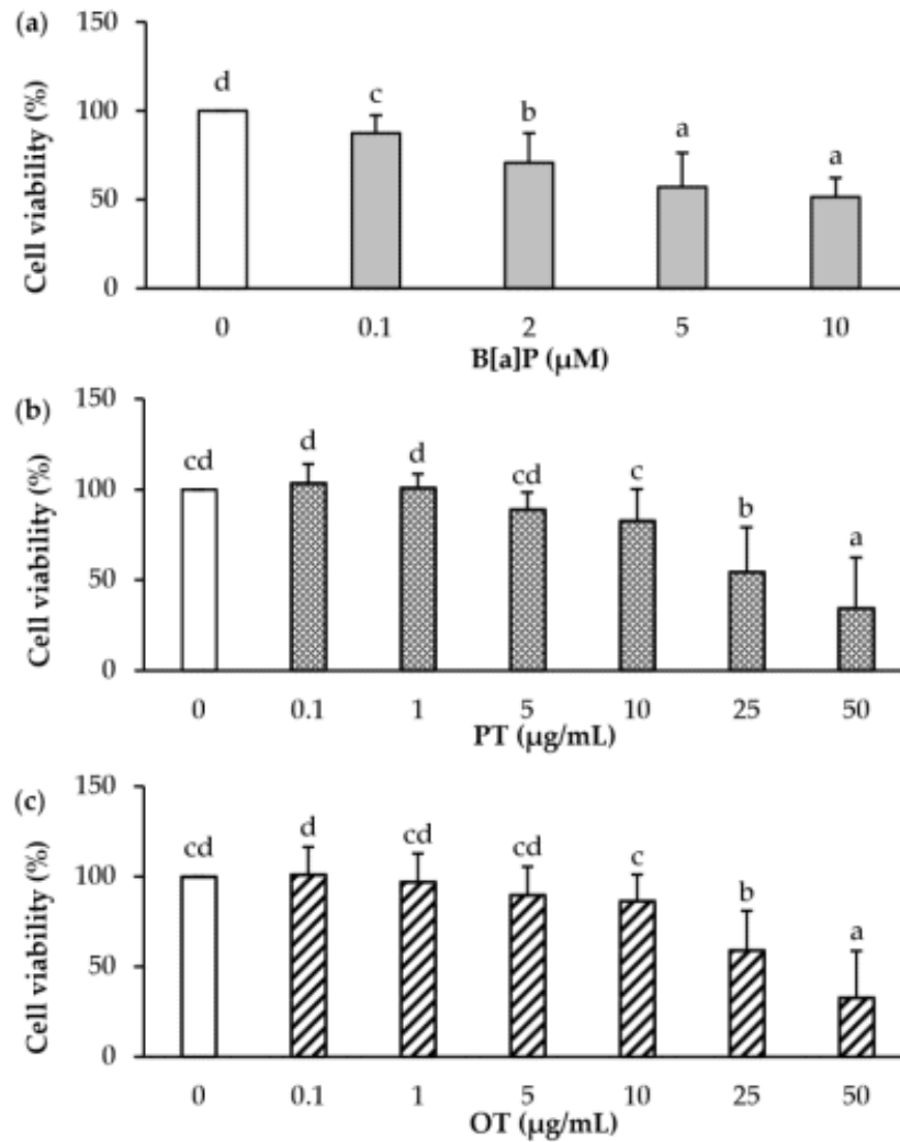
Figure 1. Cytotoxicity of B[a]P, P. tricornutum , and O. tauri extracts in endothelial HMEC-1 cells. HMEC-1 cells were exposed to vehicle (DMSO) or different concentrations of (a) B[a]P 0.1 \mu\text{M} to 10 \mu\text{M} or (b) P. tricornutum (PT) extract and (c) O. tauri (OT) extract at 0.1 to 50 \mu\text{g/mL} for 24 h. Results are represented as mean values \pm SD from at least 3 independent experiments. Mean values assigned with different letters are significantly different ( p < 0.05 ) with a < b < c < d .
