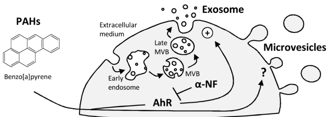
Figure 30 : Résumé graphique "PAHs increase the production of extracellular vesicles both in vitro in endothelial cells and in vivo in urines from rats". (Issue de Le Goff et al., 2019b).
