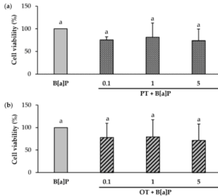
Figure 2. Effect of co-exposure to B[a]P and extracts of P. tricornutum or O. tauri on cytotoxicity in endothelial HMEC-1 cells. HMEC-1 cells were exposed to 2 µM B[a]P and (a) P. tricornutum (PT) extract and (b) O. tauri (OT) extract at 0.1 to 5 µg/mL for 24 h. Cell viability upon B[a]P treatment was set at 100% and then compared with HMEC-1 cells co-exposed with microalgal extracts. Results are represented as mean values ± SD from at least 3 independent experiments. Mean values assigned with the same letters are not significantly different ( p < 0.05 ).
