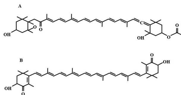
Fig. 1. Chemical structures of the main high added value bioactive xanthophylls produced by microalgae. A: fucoxanthin, B: astaxanthin.
