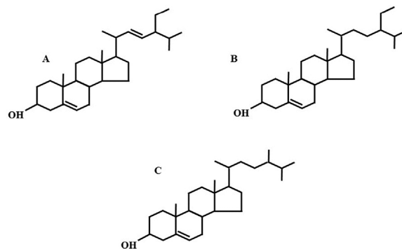
Fig. 2. Chemical structures of bioactive phytosterols produced by microalgae. A: stigmasterol, B: β-sitosterol, C: campesterol.
