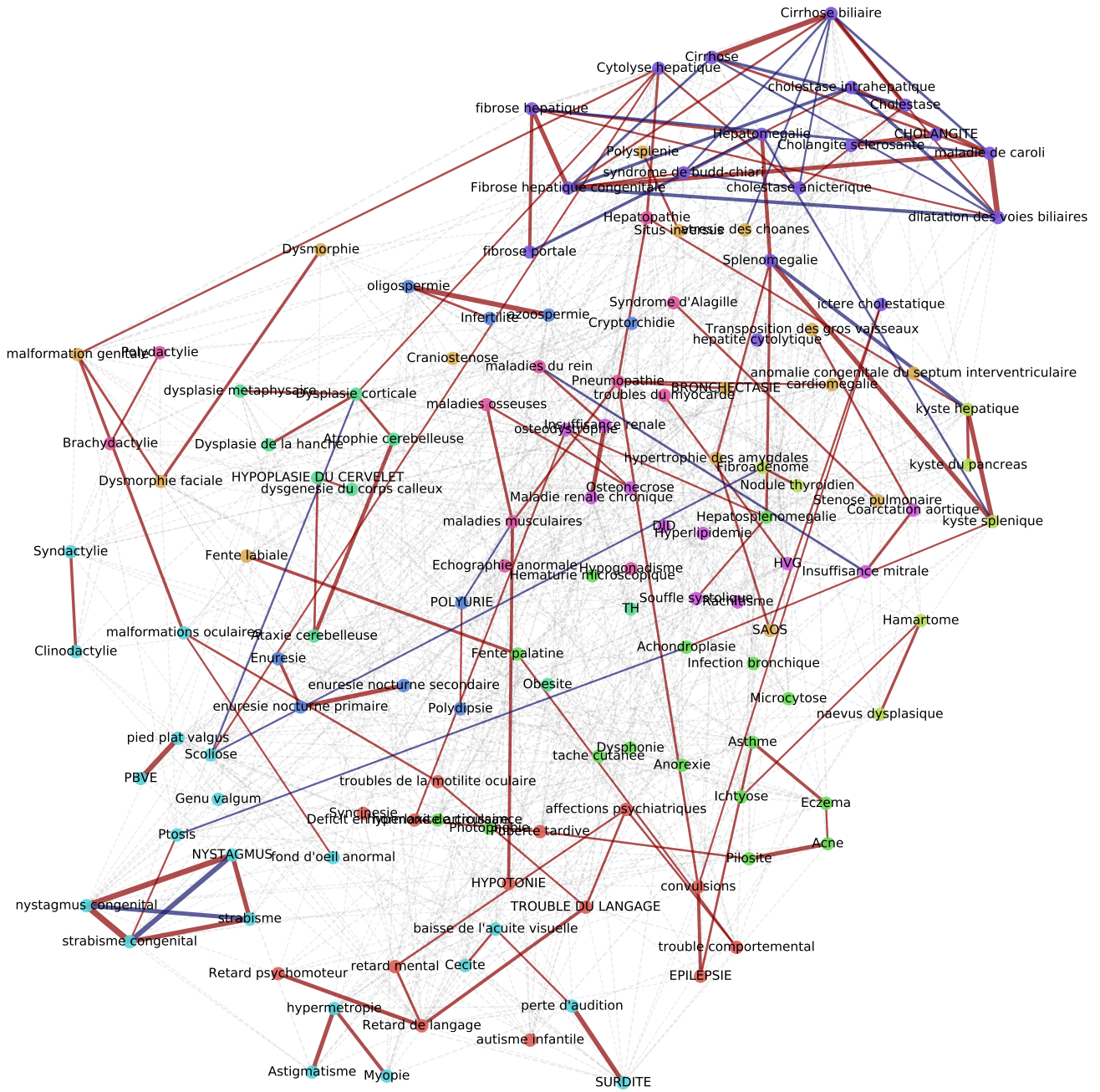
Figure 7.4: Graph prior.
