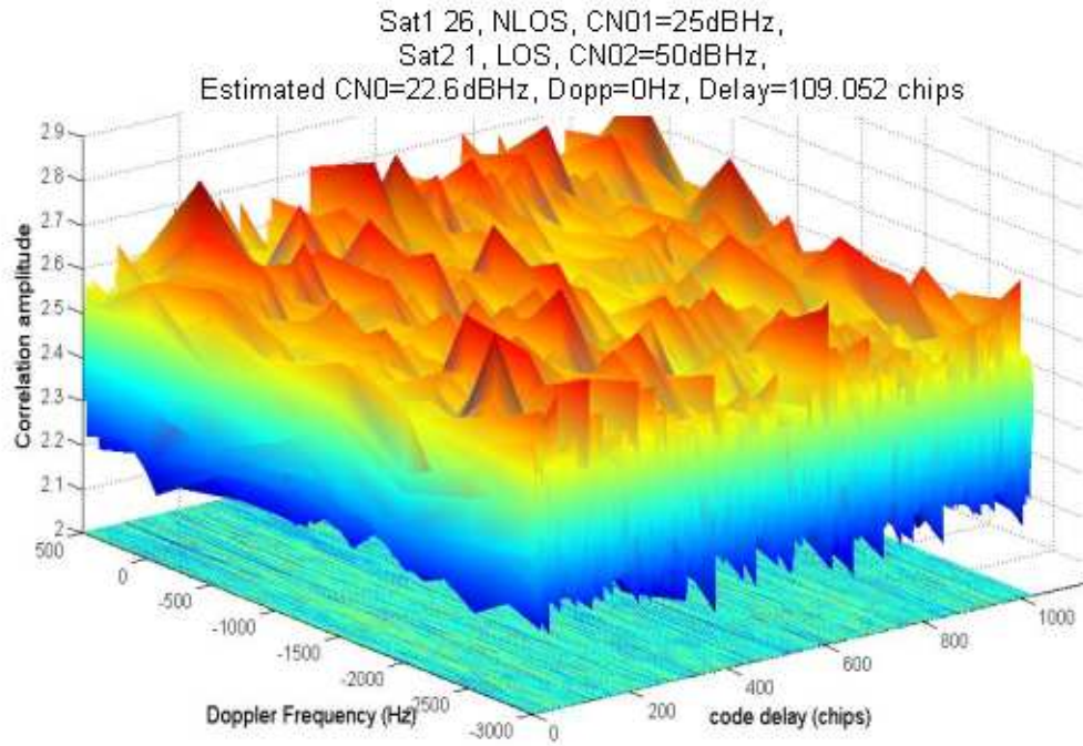
Fig III-12: Cross-correlation between 2 GPS signals: 1- Non LOS signal of satellite number 26 (just multipath replicas), true Doppler 4000 Hz , true delay 604.03 chips, initial C / N_0 = 25 dBHz 2- LOS signal of satellite number 1 with multipath replicas, true Doppler 0 Hz , true delay 608.27 chips, initial C / N_0 = 50 dBHz .
