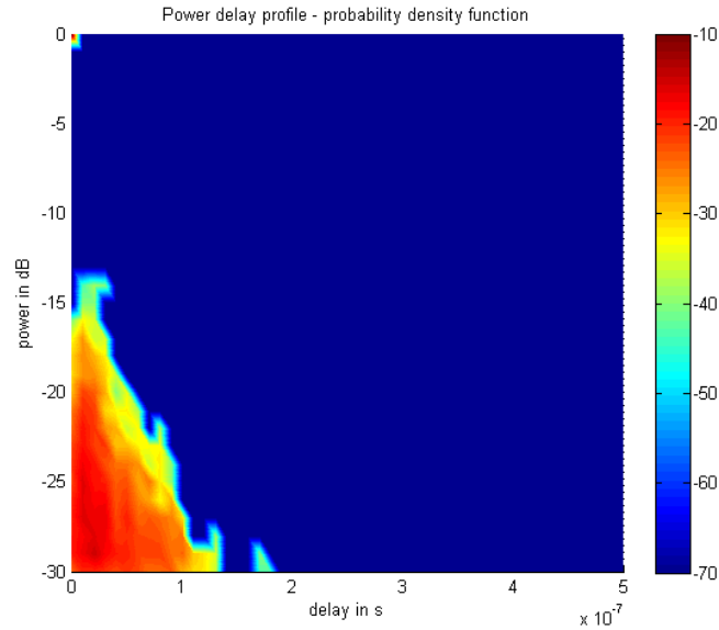
Fig III-16 : PDP and PDF for a satellite elevation angle of 90° and an azimuth of -30°, for test A (downtown environment)
