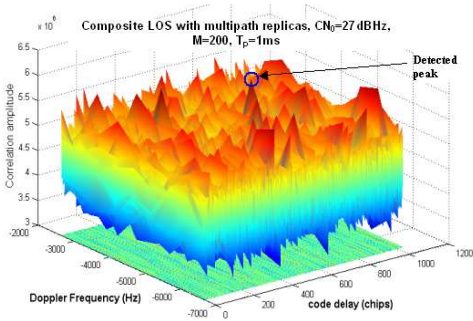
Fig III-8: Composite LOS with multipath replicas; C/N_0 = 27 dBHz true values: Doppler frequency – 4666 Hz , code delay 608.27 chips; estimated values: Doppler frequency – 4666 Hz , code delay 608.27 chips,
