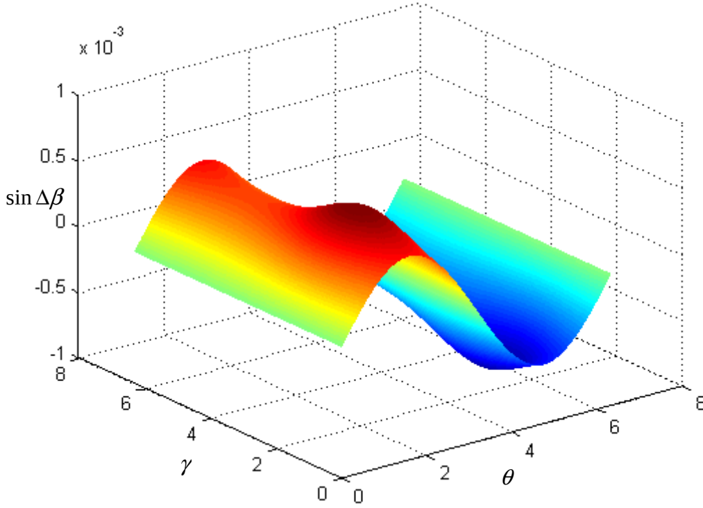
Fig. C-3: \sin \Delta\beta as a function of \gamma and \theta
