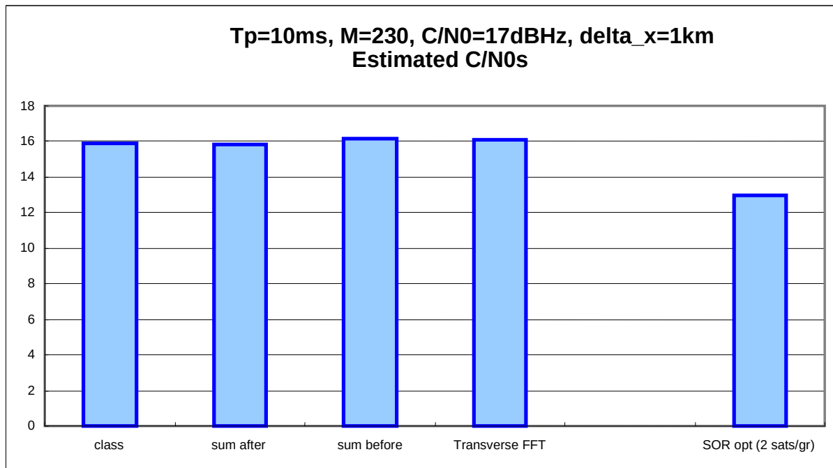
Fig VI-13: Estimated C / N_0 for a signal of 17\text{ dBHz} , with fixed M and T_p
