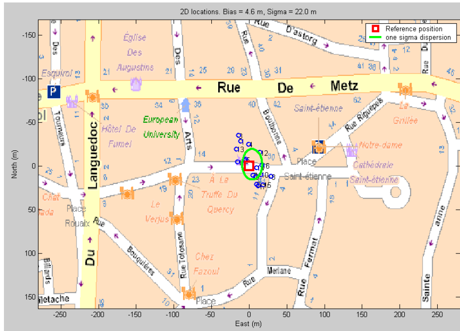
Fig IV-26 : Alcatel demonstrator 2D error
