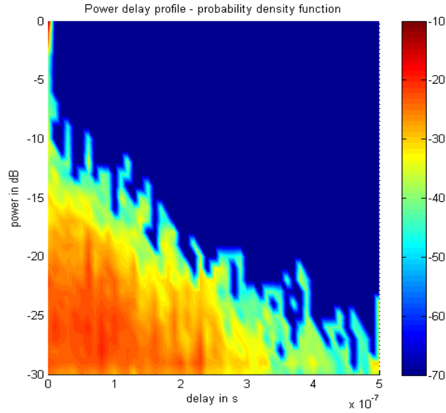
Fig III-17 : PDP and PDF for a satellite elevation angle of 30° and an azimuth of 60°, for test B (urban canyon)
