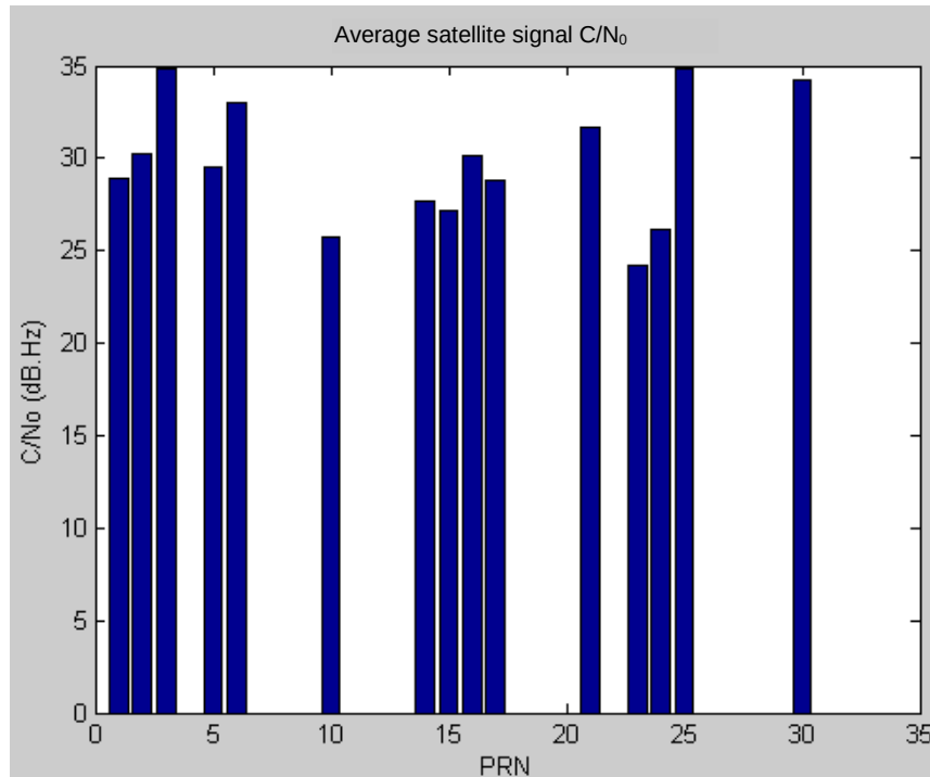
Fig IV-18 : Alcatel demonstrator average satellite signal C/N_0
