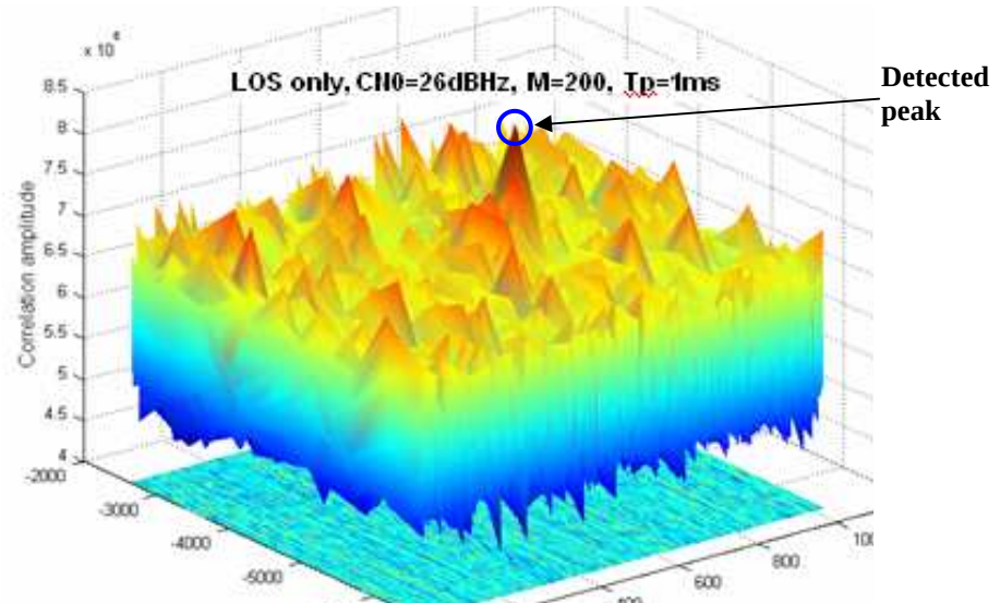
Fig III-7: LOS without multipath replicas; C/N_0 = 26\text{ dBHz} ; true values: Doppler frequency -4666\text{ Hz} , code delay 608.27\text{ chips} ; estimated values: Doppler frequency -4666\text{ Hz} , code delay 608.27\text{ chips}
