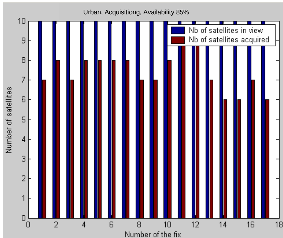
Fig IV-25 : Alcatel demonstrator number of satellites and availability percentage
