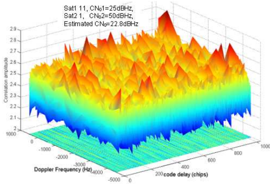
Fig III-10: Cross-correlation between 2 GPS signals: 1- LOS signal of satellite number 11 with multipath replicas, true Doppler – 4075 Hz , true delay 608.27 chips, initial C / N_0 = 25 dBHz 2- LOS signal of satellite number 1 without multipath replicas, true Doppler 0 Hz , true delay 604.03 chips, C / N_0 = 50 dBHz . The signal acquired is that of PRN 11. Estimated values: Doppler frequency 0Hz, code delay 280.24 chips, C / N_0 = 22.8 dBHz
