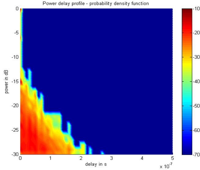
Fig III-15 : PDP and PDF for a satellite elevation angle of 60° and an azimuth of 60°, for test A (downtown environment)
