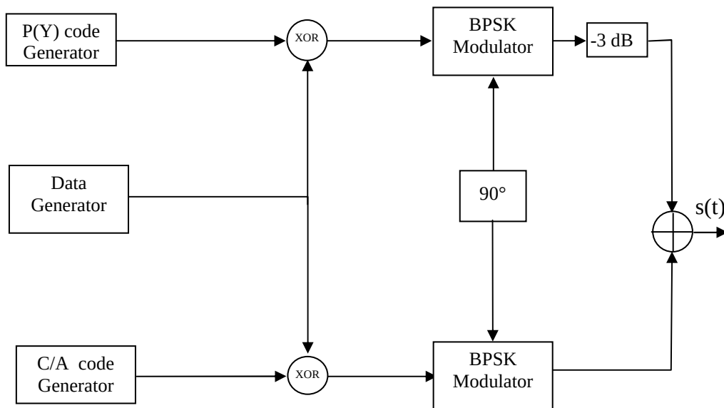
Fig II-2: GPS L_1 carrier modulation
