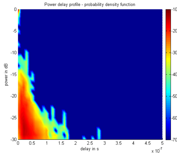
Fig III-18 : PDP and PDF for a satellite elevation angle of 60° and an azimuth of 0°, for test B (urban canyon)
