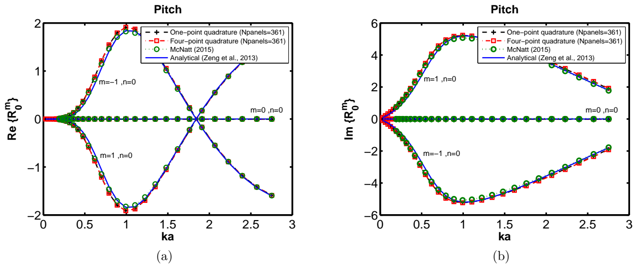
Figure I.11: Real and imaginary parts of the Radiation Characteristics progressive terms for a truncated vertical cylinder of 3m radius (a), 6m draft moving in pitch in a 10m water depth.
