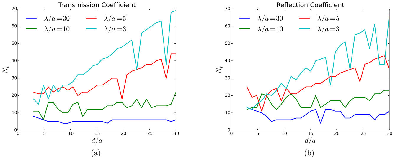
Figure 6.7: Number of angular discretization samples N_t as a function of the separating distance between bodies d for both the transmission a) and reflection b) coefficients of an array of 3 truncated vertical cylinders as shown in Figure 6.5a.
