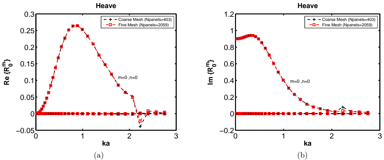
Figure I.7: Real and imaginary parts of the Radiation Characteristics progressive terms for a square box of 6m side (2a), 6m draft moving in heave in a 10m water depth.
