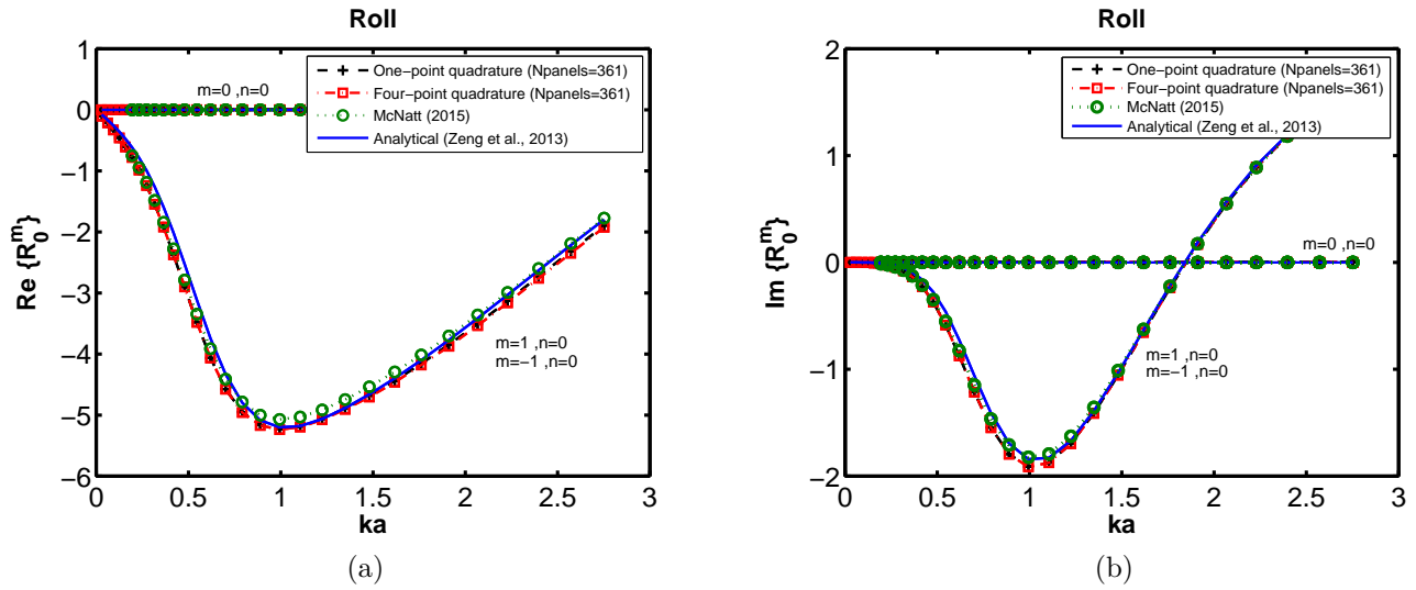
Figure I.10: Real and imaginary parts of the Radiation Characteristics progressive terms for a truncated vertical cylinder of 3m radius (a), 6m draft moving in roll in a 10m water depth.
