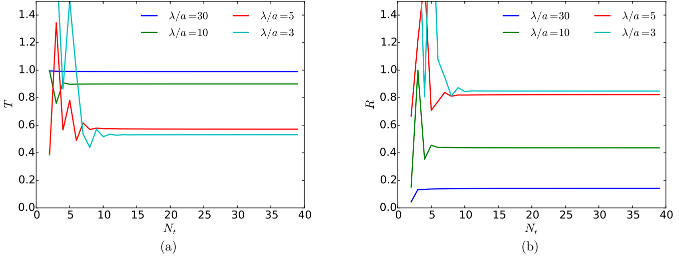
Figure 6.6: Transmission a) and reflection b) coefficient as a function of the angular variable sampling N_t for an array of 3 truncated vertical cylinders disposed parallel to the Y axis as in Figure 6.5a and with d/a = 4
