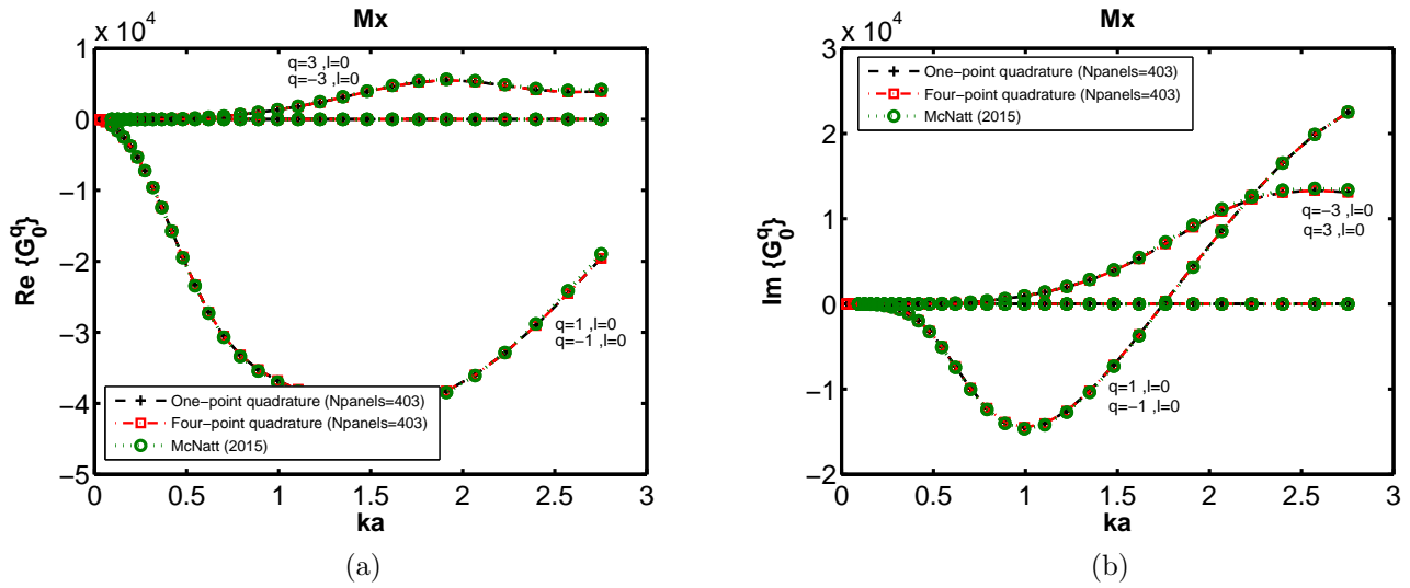
Figure I.19: Real and imaginary parts of the Force Transfer Matrix progressive M_x terms for a square box of 6m side (2a), 6m draft in a 10m water depth.
