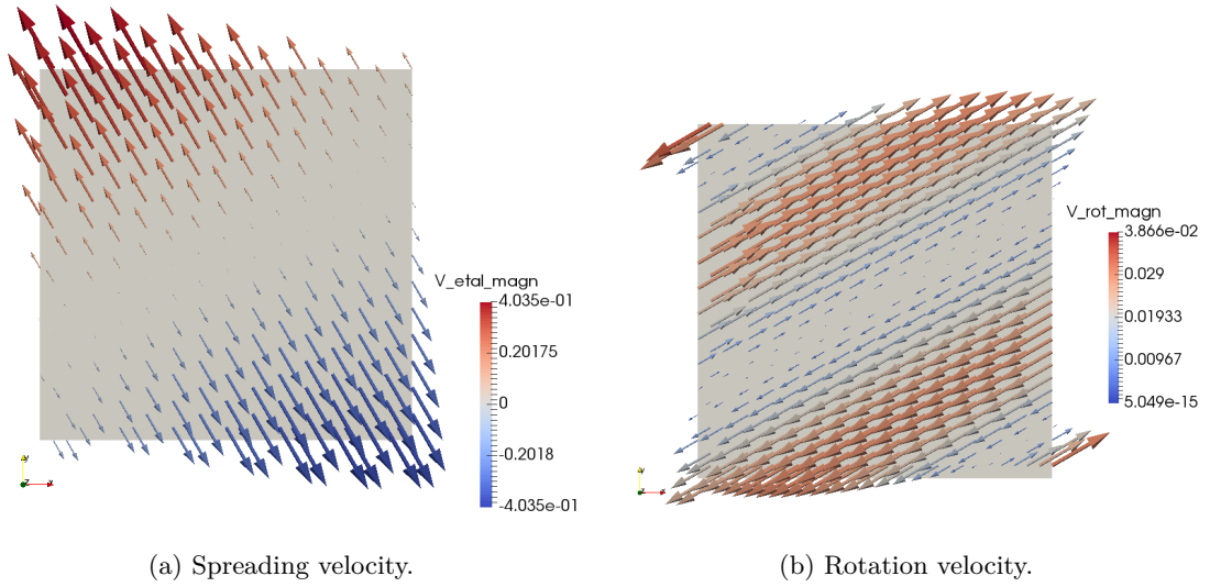
Figure 3.9 – Decomposition of the velocity field in the middle of the lower ply. The velocity is expressed in \text{mm.s}^{-1} .
