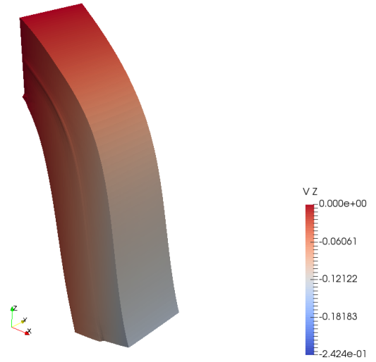
(c) Z-axis velocity ( \text{mm.s}^{-1} ) at 15s (30 th timestep).
