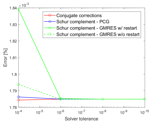
(a) Error on the velocity, expressed in %.
