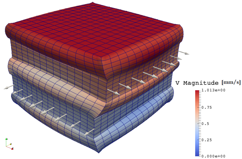
Figure 3.5 – Velocity magnitude expressed in \text{mm.s}^{-1} . The bottom ply is oriented at 0^\circ and the top one at 90^\circ .
