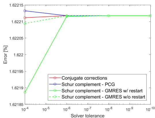
(b) Error on the pressure, expressed in %.
