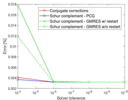
(c) Error on the fibre tension, expressed in %.
