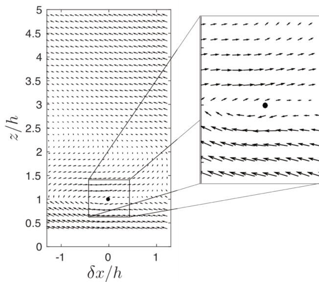
Figure 6.16. Conditional average of u' and w' based on a forward scatter event at z/h = 1 .
