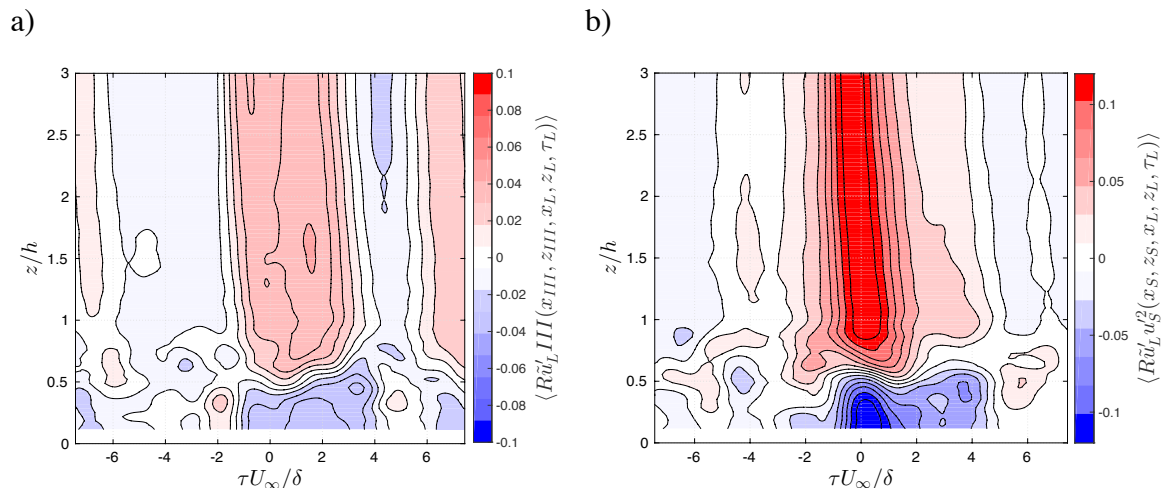
Figure 7.8. a) Spatially averaged spatial Correlation Coefficient \langle R_{\tilde{u}'_L III} \rangle where x_L = x_{III} and z_{III} = 1 ; b) Spatially averaged spatial Correlation Coefficient \langle R_{\tilde{u}'_L u'_S{}^2} \rangle where x_L = x_S and z_S = 1 .
