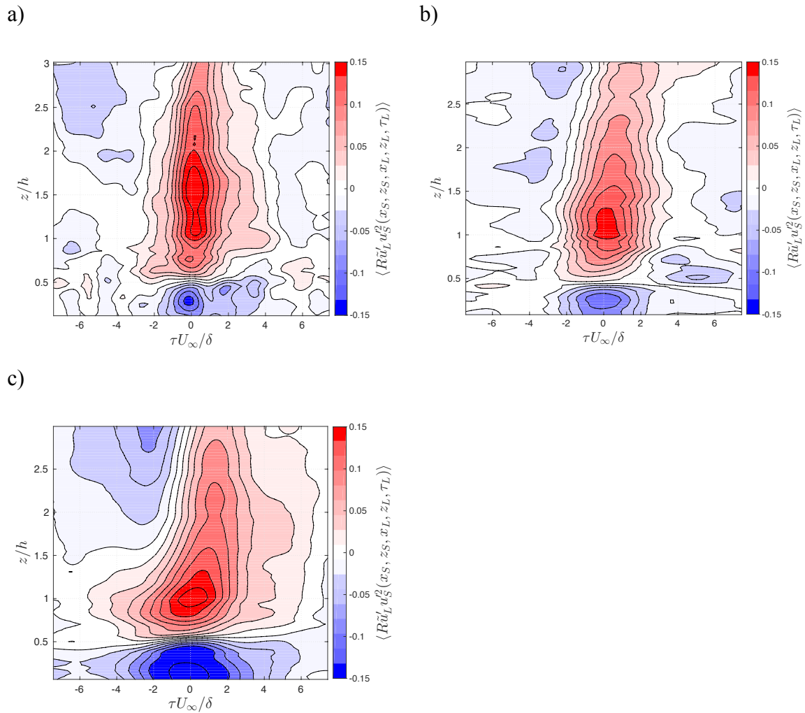
Figure 5.6 Spatially averaged Correlation Coefficient \langle R_{\tilde{u}'_L u'^2_S} \rangle where x_L = x_S and z_L = z_S .of a) Rcu; b) R1h; c) R3h.
