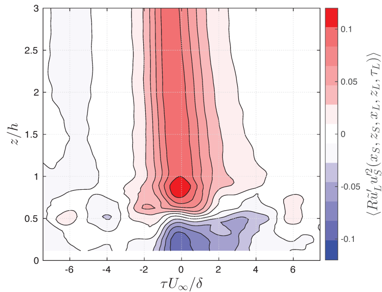
Figure 4.11. Spatially averaged spatial Correlation Coefficient \langle R_{\tilde{u}'_L \tilde{u}'_S} \rangle where x_L = x_S and z_S = .0.75 .
