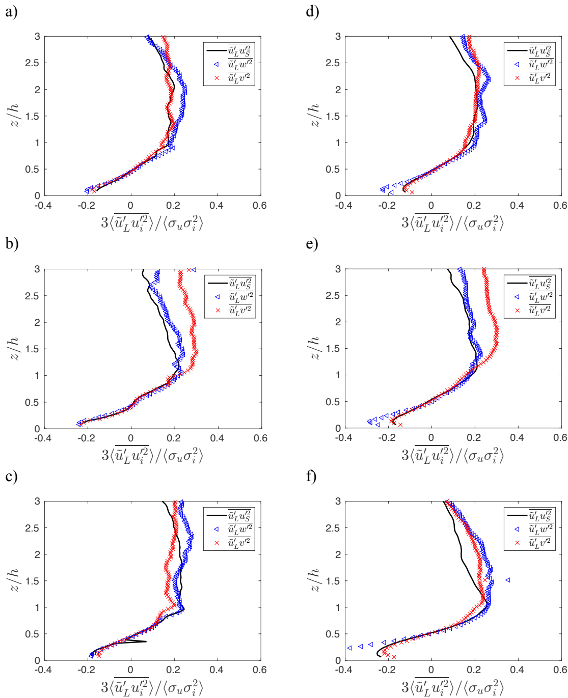
Figure 5.11. Non-linear skewness terms 3\langle \bar{u}'_L u_i'^2 \rangle (-), 3\langle \bar{u}'_L w'^2 \rangle ( \triangleleft ) and 3\langle \bar{u}'_L v'^2 \rangle ( \times ) all spatially averaged over canyon width and normalized by \langle \sigma_u \sigma_i^2 \rangle for a) C1hRcu; b) C1hR1h; c) C1hR3h; d) C3hRcu; e) C3hR1h; f) C3hR3h.
