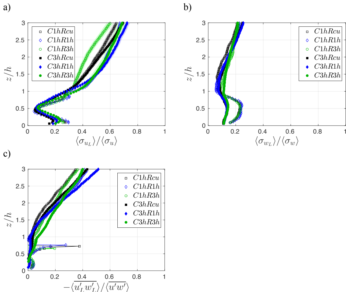
Figure 5.9. Contribution of the large-scales, \widetilde{u}'_L to a) \langle \sigma_u \rangle , b) \langle \sigma_w \rangle and c) \langle \overline{u'w'} \rangle spatially averaged over canyon width. Outlying points in \langle \overline{u'_L w'_L} \rangle are due to normalization by zero.
