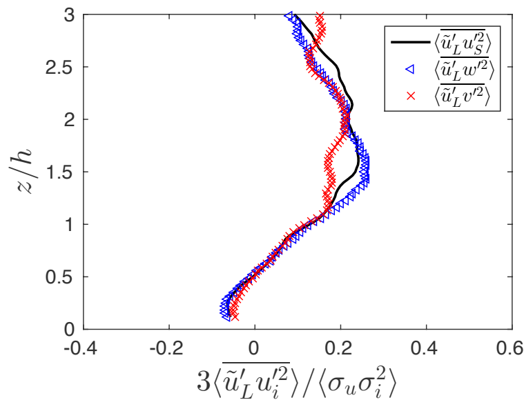
Figure 4.9. Non-linear skewness terms 3 \langle \tilde{u}'_L u'^2_S \rangle (-), 3 \langle \tilde{u}'_L w'^2 \rangle ( \triangleleft ) and 3 \langle \tilde{u}'_L v'^2 \rangle ( \times ) all spatially averaged and normalized by \langle \sigma_u \sigma_i^2 \rangle .
