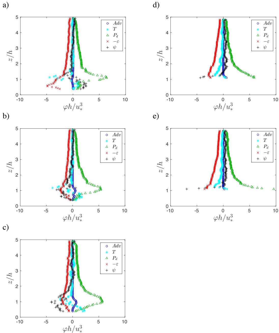
Figure 6.6. Turbulent Kinetic Energy Budget with \varepsilon_{LE-PIV} dissipation from the x - z plane (left column) at a) A; b) B; c) C and from the y - z plane (right column) at d) D; e) E with all terms normalized by h/u_*^3 .
