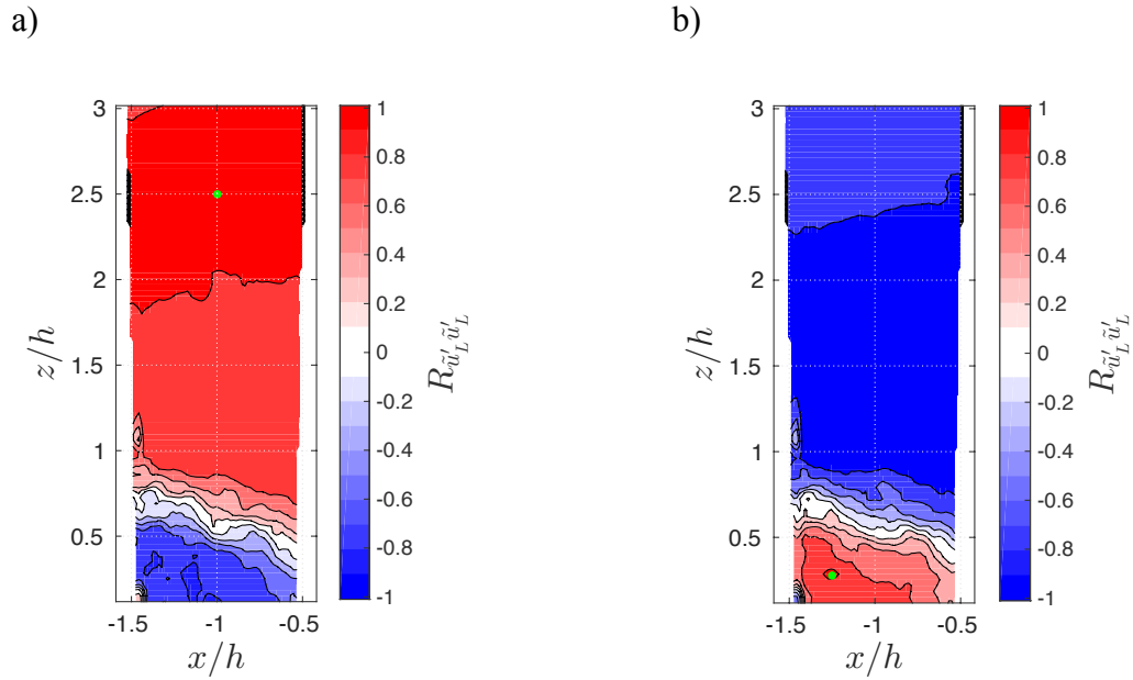
Figure 4.2. Spatial correlation coefficient ( R_{\tilde{u}'_L \tilde{u}'_L} ) of the streamwise velocity fluctuations predicted by the LSE model ( \tilde{u}'_L ) with reference point ( \bullet ) of a) x/h = -1, z/h = 2.5 and b) x/h = -1.25, z/h = 0.25 .
