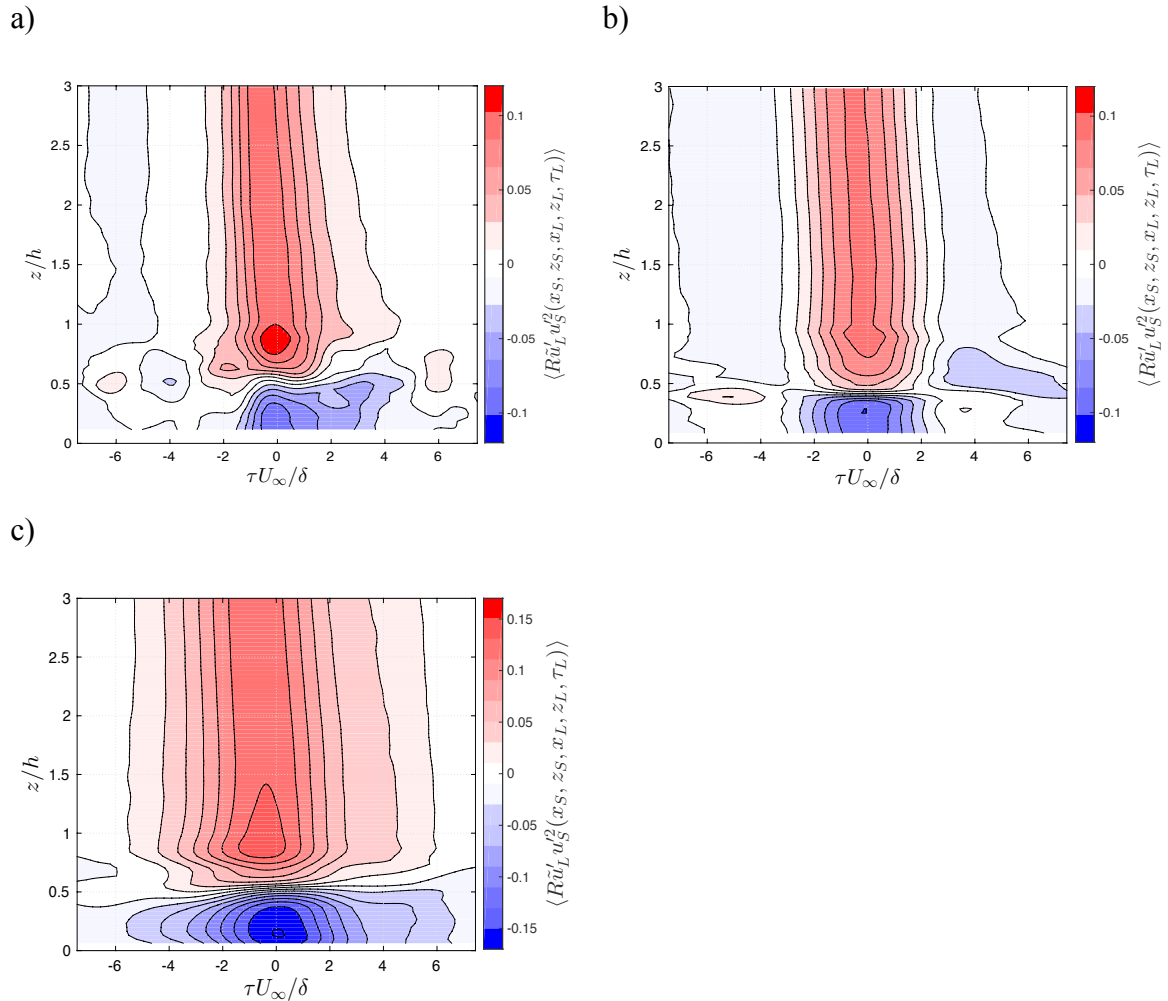
Figure 5.7 Spatially averaged spatial Correlation Coefficient \langle R_{\tilde{u}'_L \tilde{u}'_S} \rangle where x_L = x_S and z_S = 0.75 of a) Rcu; b) R1h; c) R3h.
