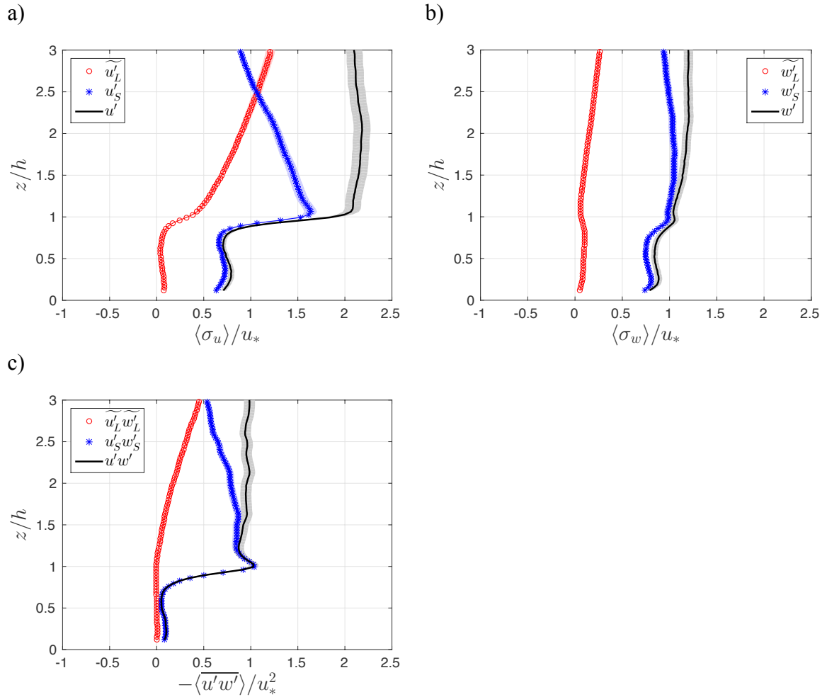
Figure 4.1. Contribution of the large-scales, \widetilde{u}'_L (o) and small-scales, \widetilde{u}'_S (*) to spatially averaged a) \langle \sigma_u \rangle , b) \langle \sigma_w \rangle and c) \langle \overline{u'w'} \rangle .
