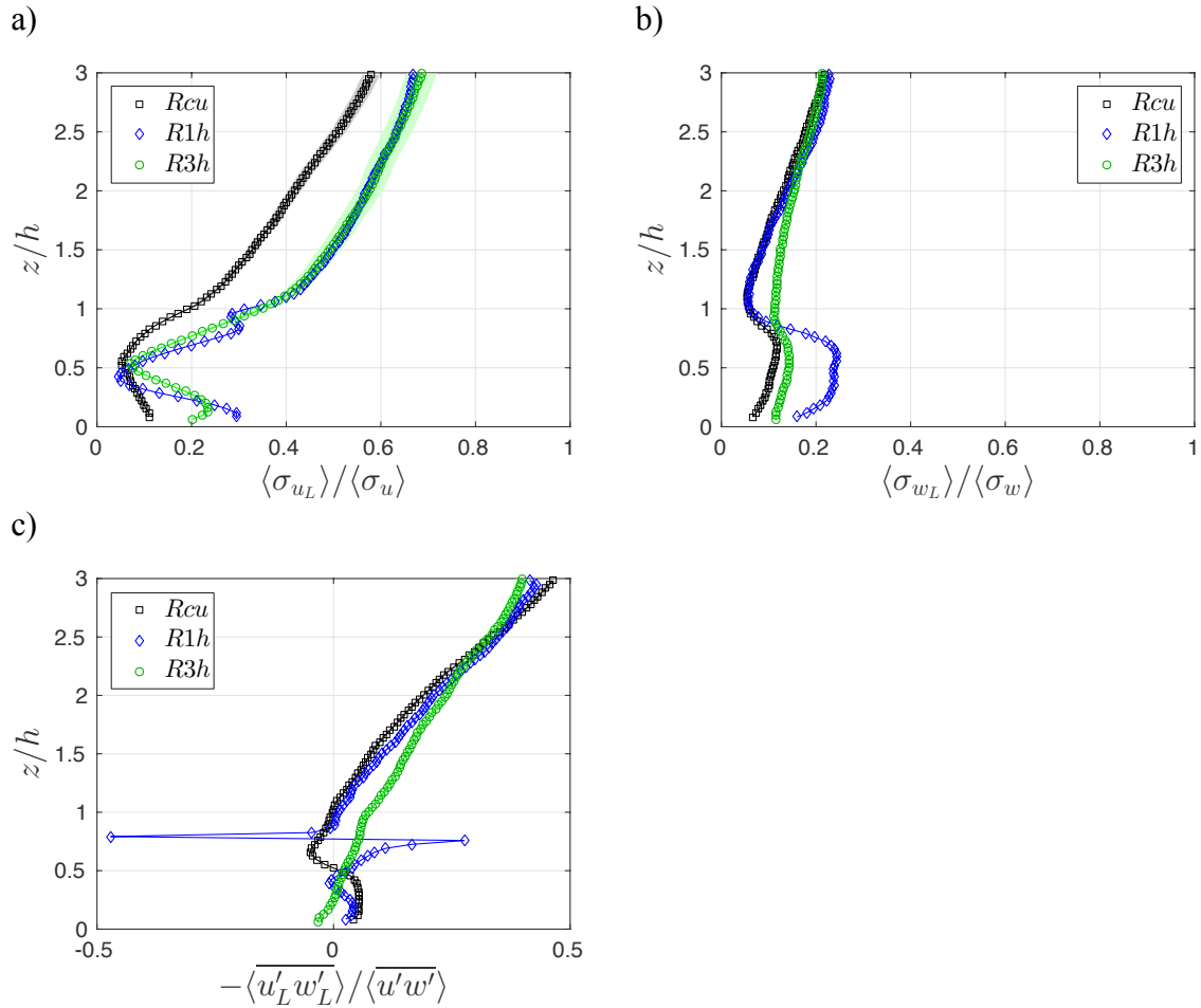
Figure 5.3 Contribution of the large-scales, \widetilde{u}'_L to spatially averaged a) \langle \sigma_{u_L} \rangle , b) \langle \sigma_{w_L} \rangle and c) \langle \overline{u'_L w'_L} \rangle . Outlying points in \langle \overline{u'_L w'_L} \rangle are due to normalization by zero.
