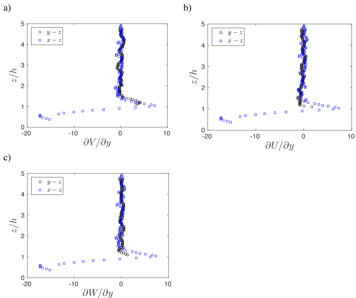
Figure B.1 a) \partial V/\partial y calculated from the y - z plane compared with estimation from divergence free condition in the x - z plane; b) \partial U/\partial y and c) \partial W/\partial y calculated from the y - z plane compared with estimation from isotropy condition in the x - z plane.
