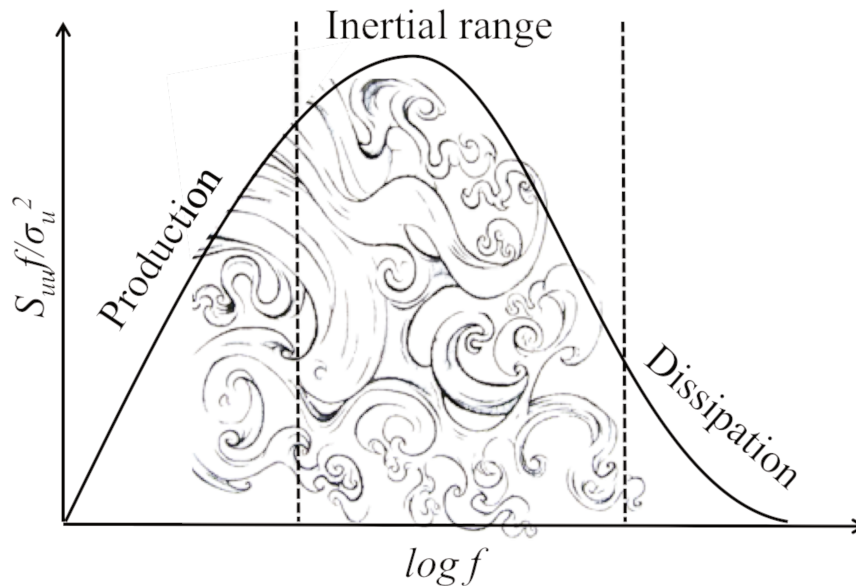
Figure 1.2. The turbulence spectra
