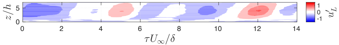
Figure 4.5. Temporal evolution of streamwise velocity fluctuations predicted by the LSE model ( \tilde{u}'_L ) at x/h = 0 .
