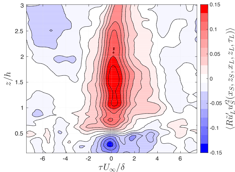
Figure 4.10. Spatially averaged Correlation Coefficient \langle R_{\tilde{u}'_L u'_S{}^2} \rangle where x_L = x_S and z_L = z_S .
