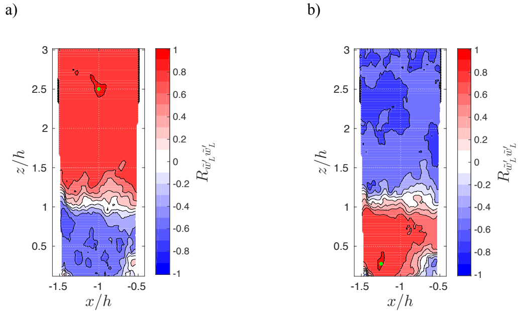
Figure 4.3. Spatial correlation coefficient ( R_{\tilde{w}'_L \tilde{w}'_L} ) of the vertical velocity fluctuations predicted by the LSE model ( \tilde{w}'_L ) with reference point ( \bullet ) of a) x/h = -1, z/h = 2.5 and b) x/h = -1.25, z/h = 0.25 .
