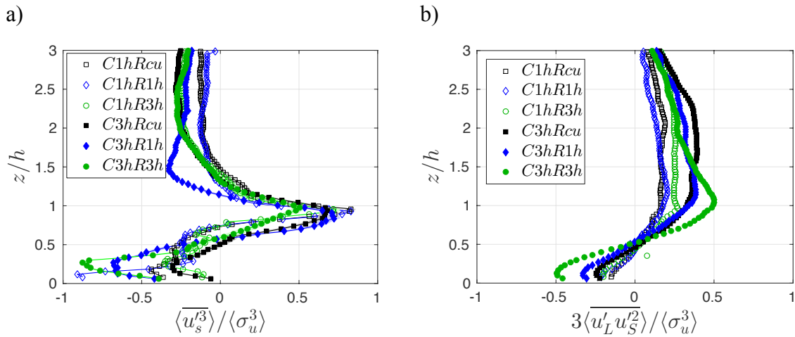
Figure 5.10 Contribution of a) \langle u'^3_s \rangle and b) 3 \langle \overline{u'_L u'^2_S} \rangle to the streamwise skewness spatially averaged over canyon width and normalized by the value of maximum skewness.
