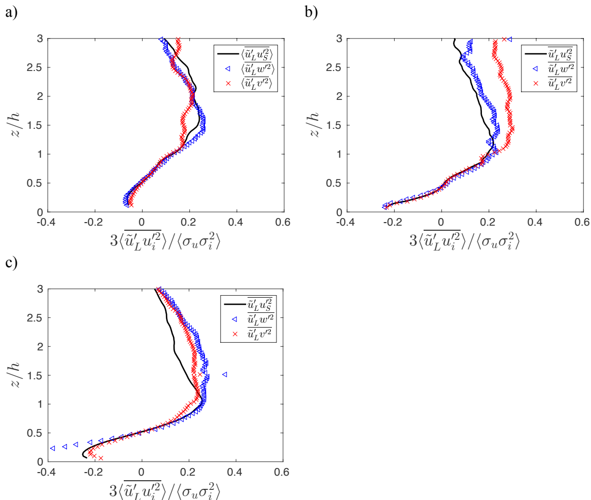
Figure 5.5 Non-linear skewness terms 3\overline{\langle \tilde{u}'_L u'^2_S \rangle} (-), 3\overline{\langle \tilde{u}'_L w'^2 \rangle} ( \triangleleft ) and 3\overline{\langle \tilde{u}'_L v'^2 \rangle} ( \times ) all spatially averaged and normalized by \langle \sigma_u \sigma_i^2 \rangle for a) Rcu; b) R1h; c) R3h.
