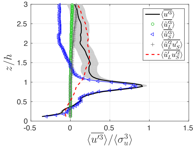
Figure 4.8. Triple decomposition of streamwise skewness, \langle \overline{u'^3} \rangle (-) including \langle \overline{u_L'^3} \rangle (o), \langle \overline{u_S'^3} \rangle ( \triangleleft ), 3 \langle \overline{u_L'^2 u_S'} \rangle (+), 3 \langle \overline{u_L' u_S'^2} \rangle (- -) all spatially averaged and normalized by \langle \sigma_u^3 \rangle .
