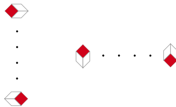
Figure 4.2: Flip lines with mixed orientations.
