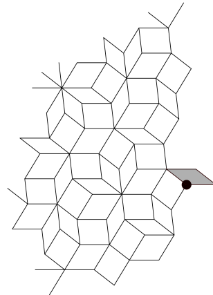
6. The new tile is forced via shadow vote two shadows vote for it.
