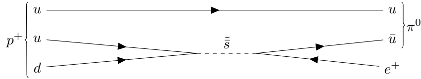
FIGURE 2.5: Example Feynman diagram for the decay of the proton in the case of R-parity violation.
