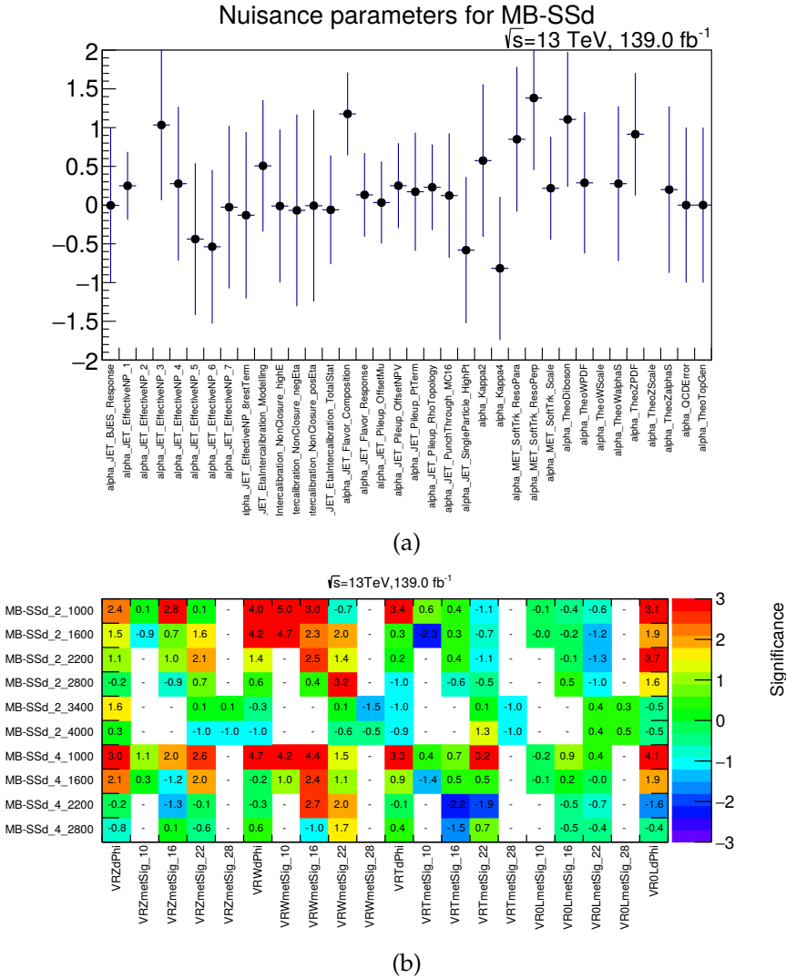
FIGURE 4.15: (a) The fitted nuisance parameters from the background-only fit for the MB-SSd search and (b) the significance, as defined in Eq. 4.13, in the validation regions of the MB-SSd search. The y-axis labels in Figure (b) correspond to the bins of the MB search according to the following format: region _N_j^{low} m_{eff}^{low} . For example, SR.2.1600 in the MB-SSs search corresponds to the SR bin with N_j=[2,4] , m_{eff}=[1600,2200] . One normalisation factor per background process is considered in the background-only fit.
