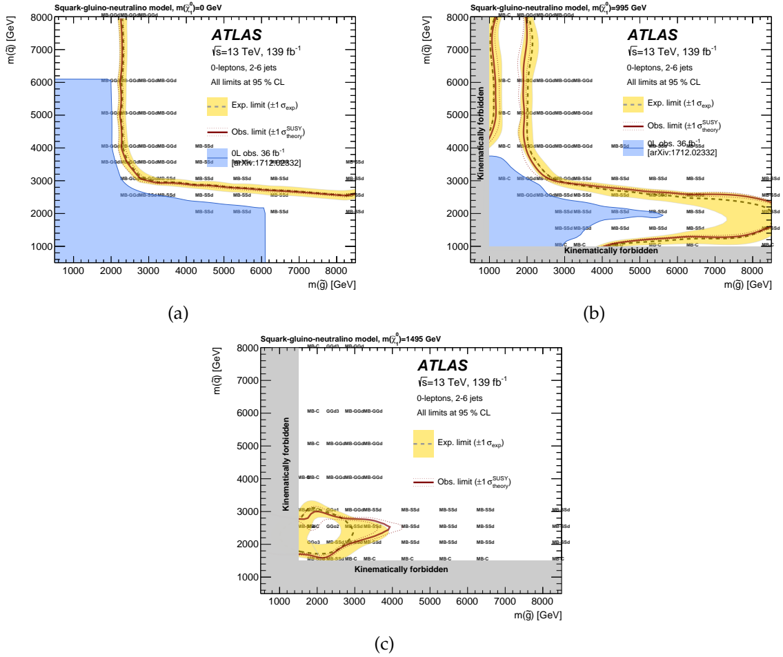
FIGURE B.4: Exclusion limits for the model with combined production of squark pairs, gluino pairs, and of squark-gluino pairs, for different assumptions on the neutralino mass: (a) m(\tilde{\chi}_1^0) = 0 GeV, (b) m(\tilde{\chi}_1^0) = 995 GeV and (c) m(\tilde{\chi}_1^0) = 1495 GeV varying values of m(\tilde{g}) and m(\tilde{q}) and assuming a purely bino \tilde{\chi}_1^0 . The gray text corresponds to the signal regions with the best expected sensitivity at each point, which is used to obtain the limits.
