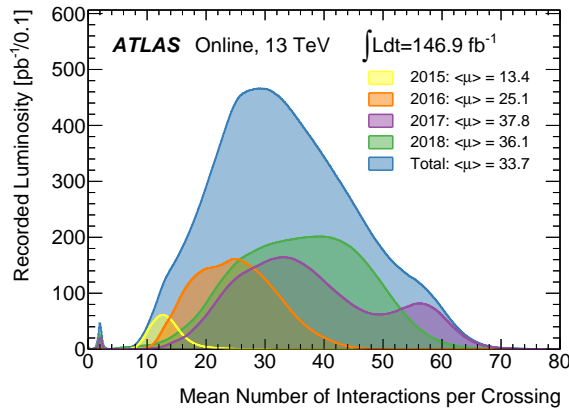
FIGURE 3.3: Distribution of the mean number of interactions per bunch-crossing for each year of the Run 2 pp collision data at 13 TeV centre-of-mass energy [48].
