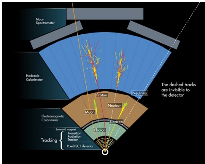
FIGURE 3.10: Transverse view of an ATLAS detector segment with a representation of the interaction of different types of particles in the different sub-detectors.
