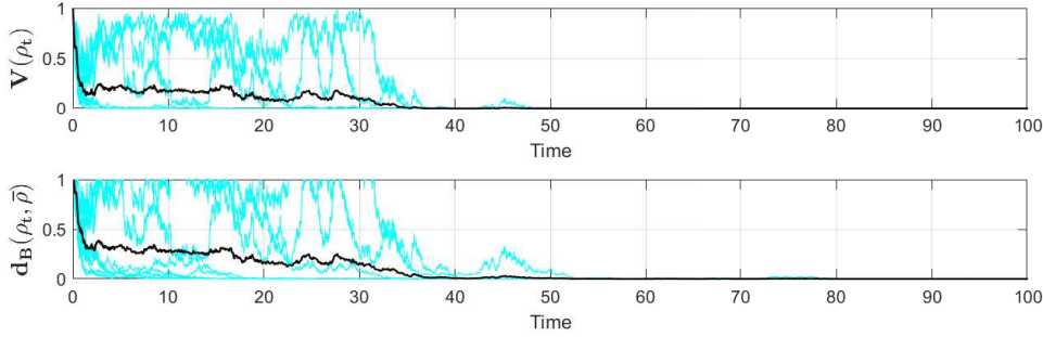
FIGURE 5.2 – Asymptotic stabilization of system (5.1) in this case towards \Psi_+ with the feedback laws (5.8) starting at \Phi_- , when \omega = 0.3 , \eta_1 = 0.3 , M_1 = 1 , \epsilon_1 = 0.1 , \epsilon_2 = 0.4 and \gamma = 8 : the black curve represents the mean value of the 10 arbitrary samples.
