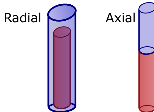
Figure 1.17: Illustration of the radial and axial NW heterostructures. The colors may represent different materials, or the same materials with different dopants. The radial geometry typically comprises an additional top segment due to the growth modes.
