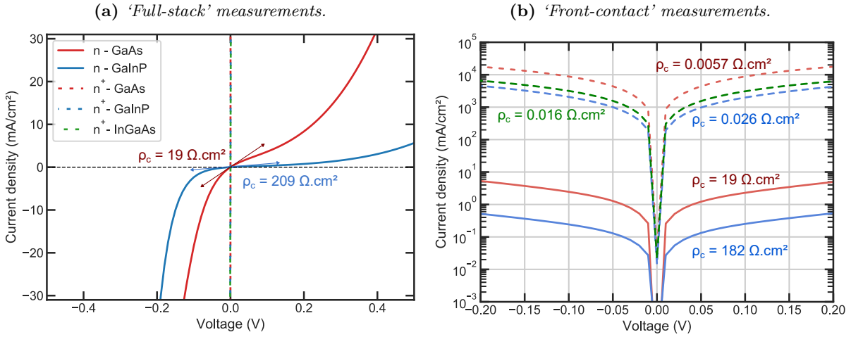
Figure 5.10: JV characteristic of an ITO contact on different III-V materials doped to n = (1.5 \pm 0.5) \times 10^{18} \text{ cm}^{-3} or n^+ = 1.7 \times 10^{19} \text{ cm}^{-3} . For n-GaAs, the substrate is directly used. (a) JV characteristic in linear scale in ‘full-stack’ configuration. The contact resistivity calculated according to Equation 5.1 is indicated. (b) Same samples measured in the ‘front-contact’ configuration. The contact resistivity calculated according to Equation 5.2 is indicated for all curves. [c1_b2,B281_b1], B272_b1, B268_b1, B273_b1
