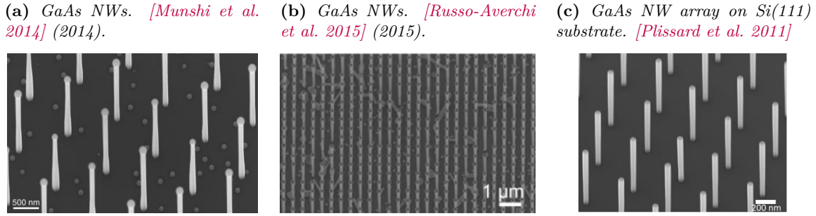
Figure 3.5: Examples of self-catalyzed GaAs NW arrays on silicon using MBE.
