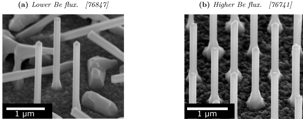
Figure 4.19: SEM details of GaAs NWs with direct Be doping during axial VLS growth. The droplet was consumed and an AlGaAs shell grown around the NWs. Viewed with a 45^\circ degree tilt.
