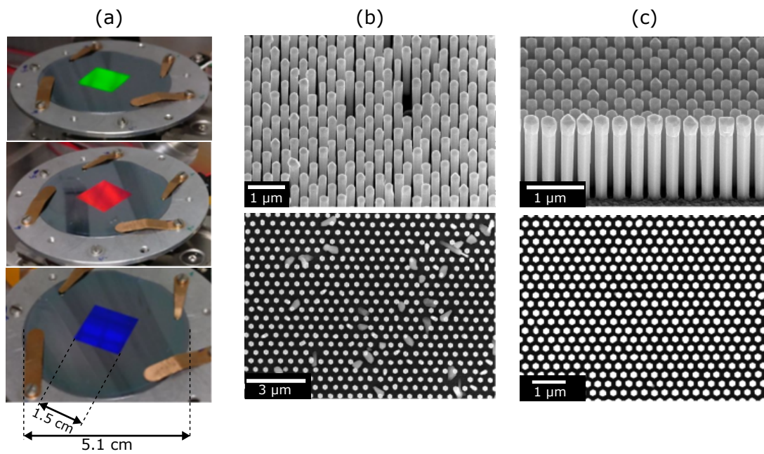
Figure 3.28: (a) Photographs of a 2" Si wafer patterned with a 1.5 cm × 1.5 cm array at the center. The periodic NW ensemble diffracts the white light in the room at different angles and colors. (b) SEM overview at the middle of the NW array at a 45° tilt (top) and in top-view (bottom). The yield is above 90%. (c) SEM overview at a pattern written 'pixel-by-pixel' (300 nm pitch, diameter P2 in the design described in Figure 2.19). The yield is 100%. [76838]
