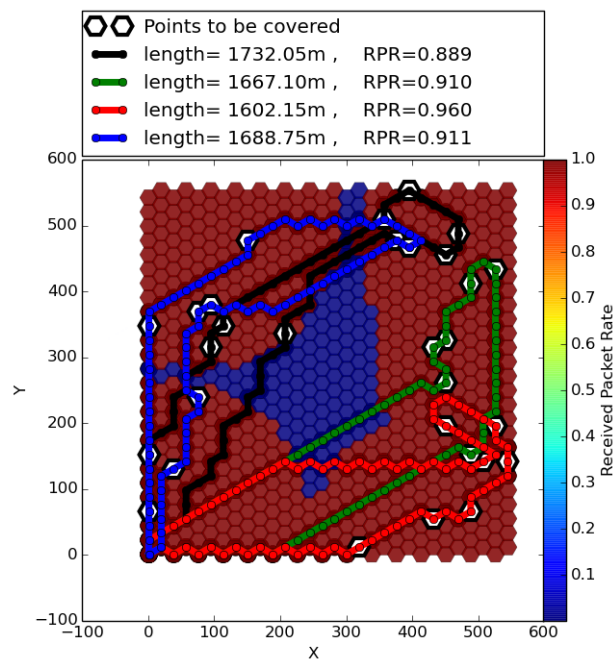
Fig. 5.2 RPR maps with path lengths with 0 jamming nodes
