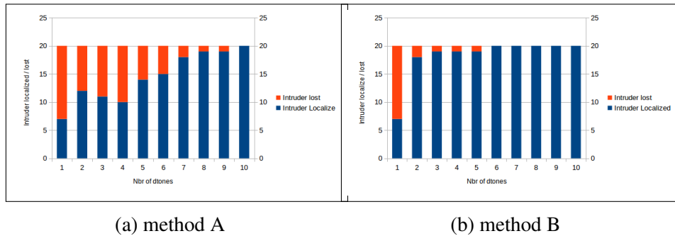
Fig. 6.7 Intruder Localization method comparison
