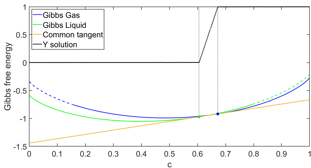
(b) NPIPМ
