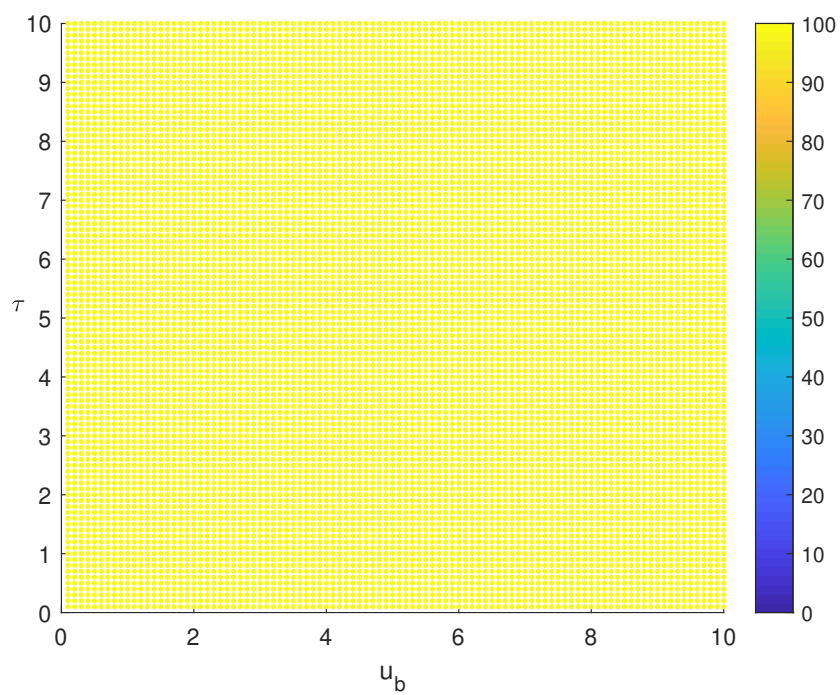
(b) NPIPМ
