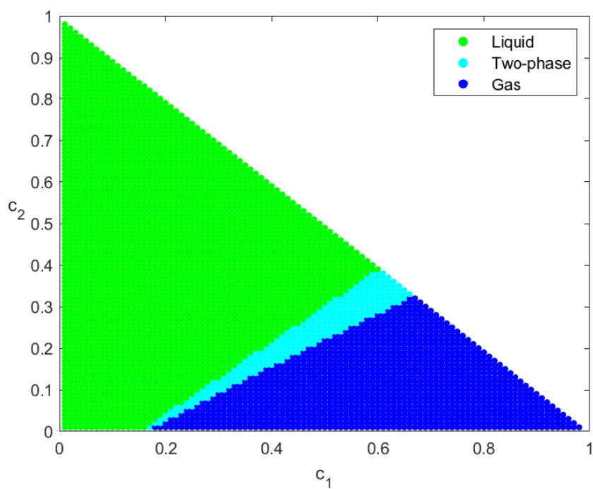
(b) NPIPIM
