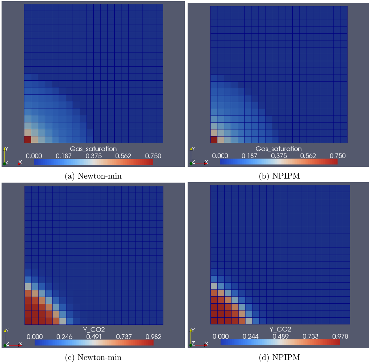
Figure 6.38: Gas saturation and partial fraction of component \text{CO}_2 in gas phase after 30 days: Newton-min method and NPIP.
