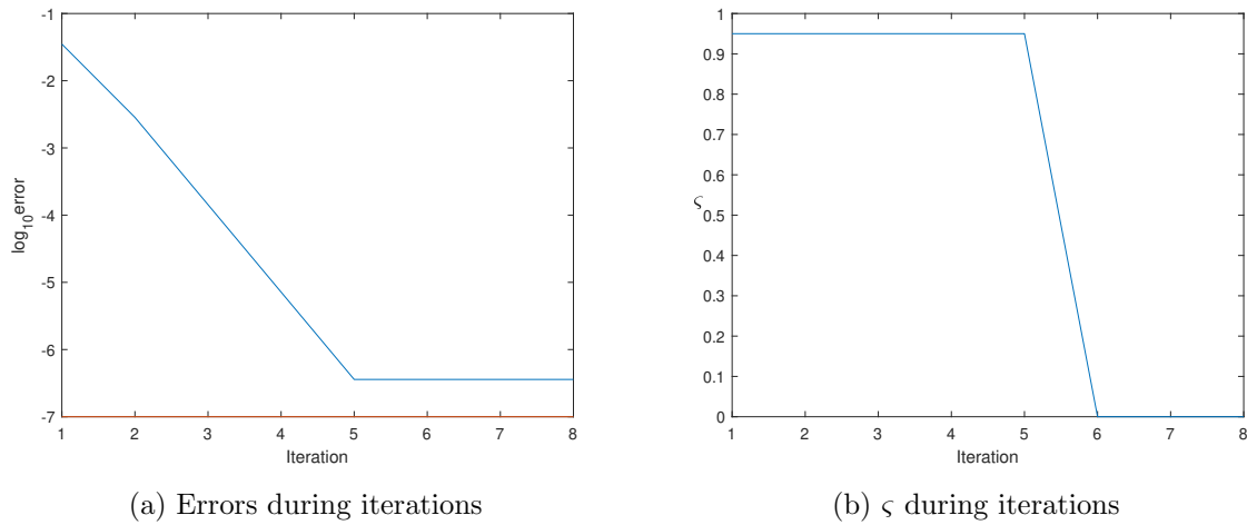
Figure 4.5: Stratigraphy model, Predictor-Corrector Mehrotra, u_b = 0.9 , \tau = 0.1 , u_0 = 0.54 , g_0 = 0.07 .
