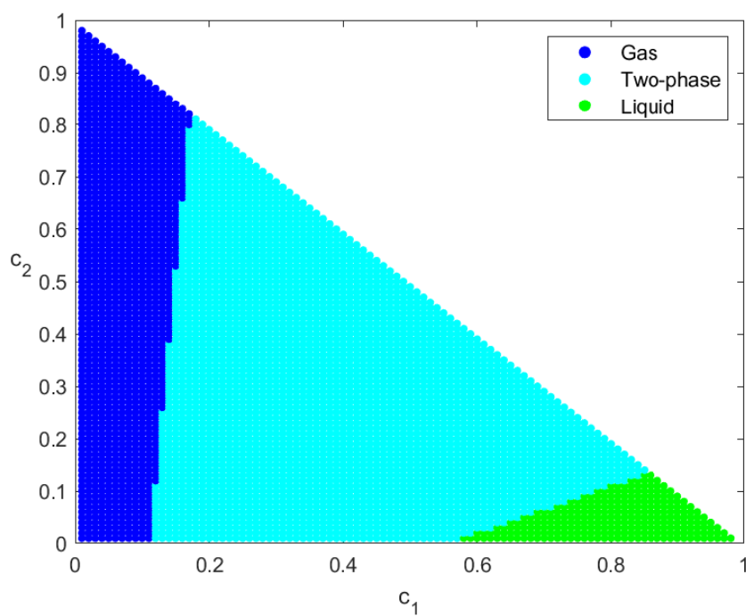
(b) NPIP
