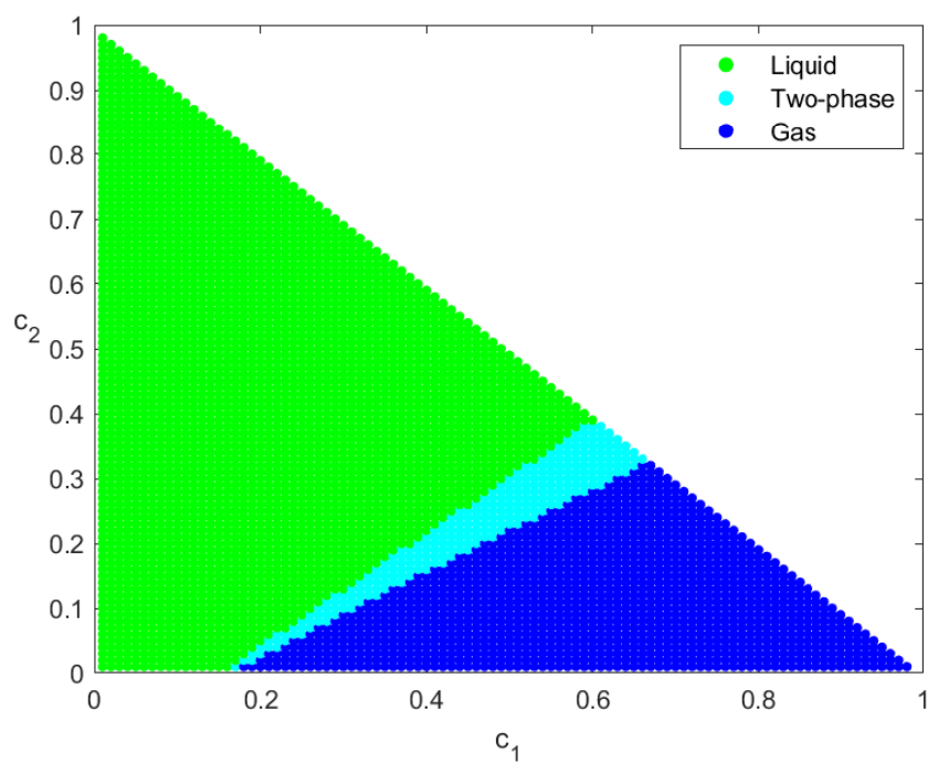
(b) NPIP
