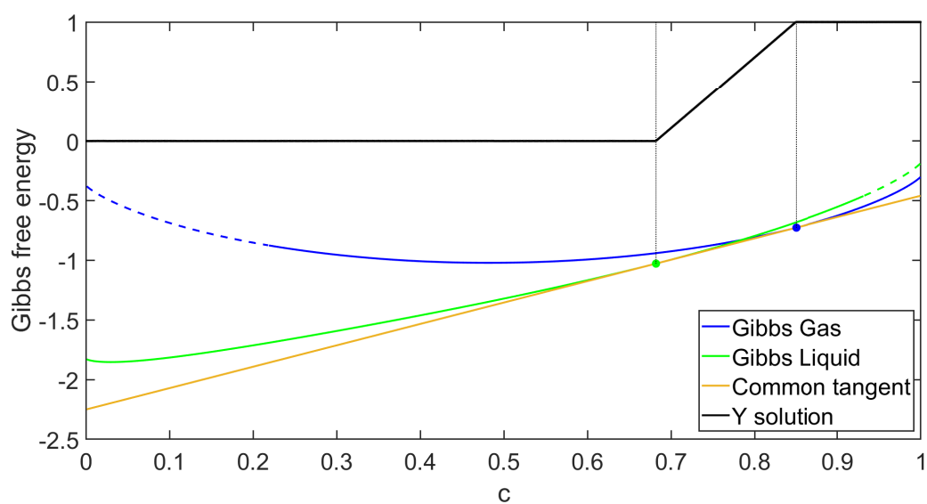
(b) NPIPМ
