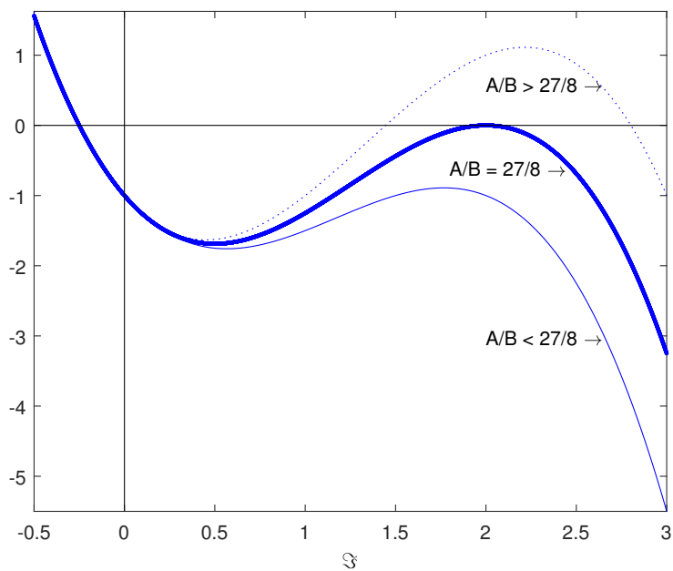
Figure 3.5: Plot of the function \mathfrak{X} \mapsto q_{A,B}(\mathfrak{X}) for various values of A/B .
