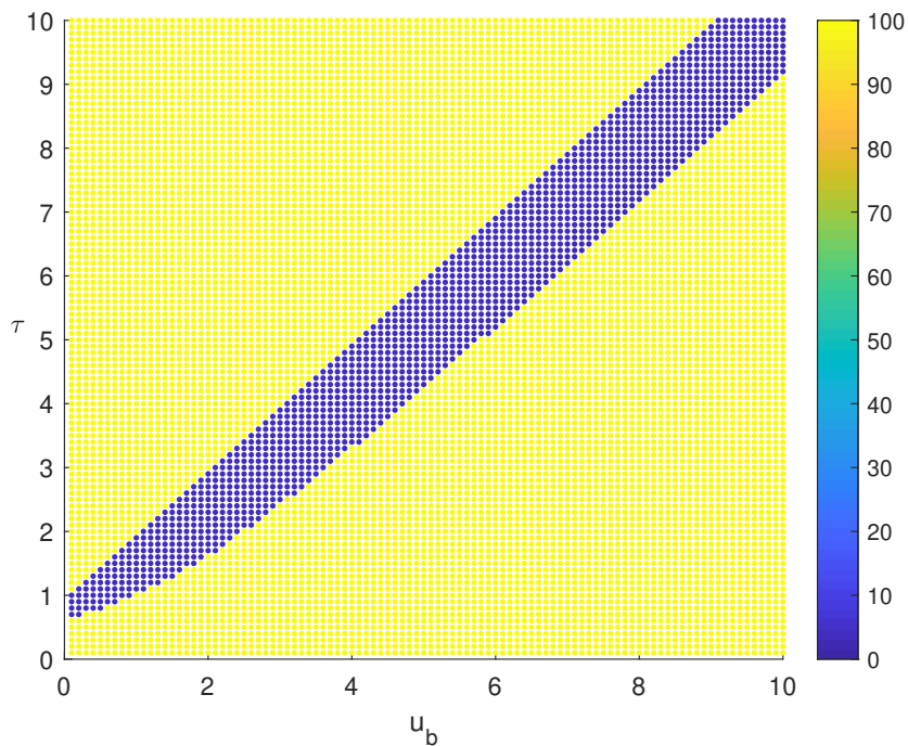
(a) Newton-min
