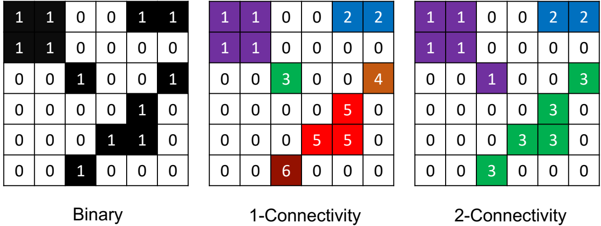
Figure 5.11: Pixel connectivity of the connected component labeling algorithm. Left: Binary image used as input for the algorithm. Center: Output of the algorithm using a 1-connectivity setting, the pixels positioned diagonally are not considered connected and are labeled separately, this results in a total of six pixel regions. Right: Output using a 2-connectivity setting, the diagonal pixels are considered connected and the result is three pixel regions.
