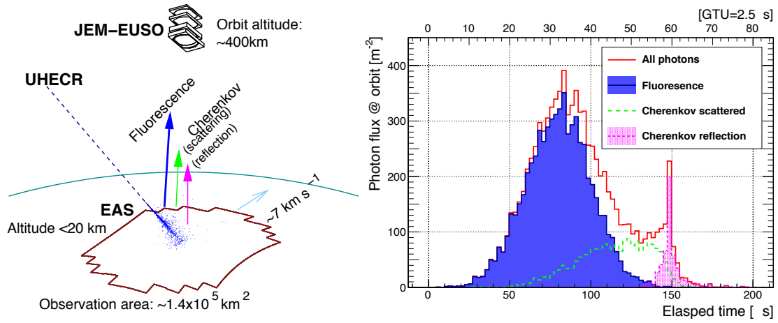
Figure 2.2: Observation principle of JEM-EUSO with an EAS in the FoV of the telescope. Left: The fluorescence emission of the EAS propagates through the atmosphere and arrives at the telescope, the scattered and reflected Cherenkov light arrives with a delay. Right: An EAS simulation showing the detected signal as a function of time. The fluorescence emission profile grows, achieves a maximum photon production and then decays. The last part of the signal is then dominated by the back-scattered Cherenkov photons and a reflected Cherenkov photon peak.
