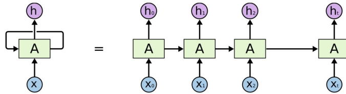
Figure 5.5: Architecture of recurrent networks
