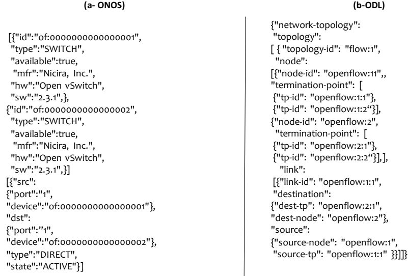
Figure 4.2: The heterogeneity of network data representation between ODL controller and ONOS controller
