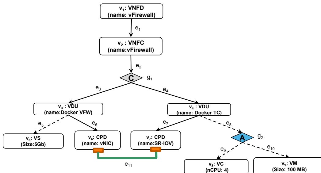
Figure 6.2: An example of a vFireWall VNFD represented graphically as a tree-like structure
