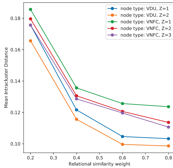
Figure 6.12: Intra-cluster mean similarity distance in terms of different relation weights
