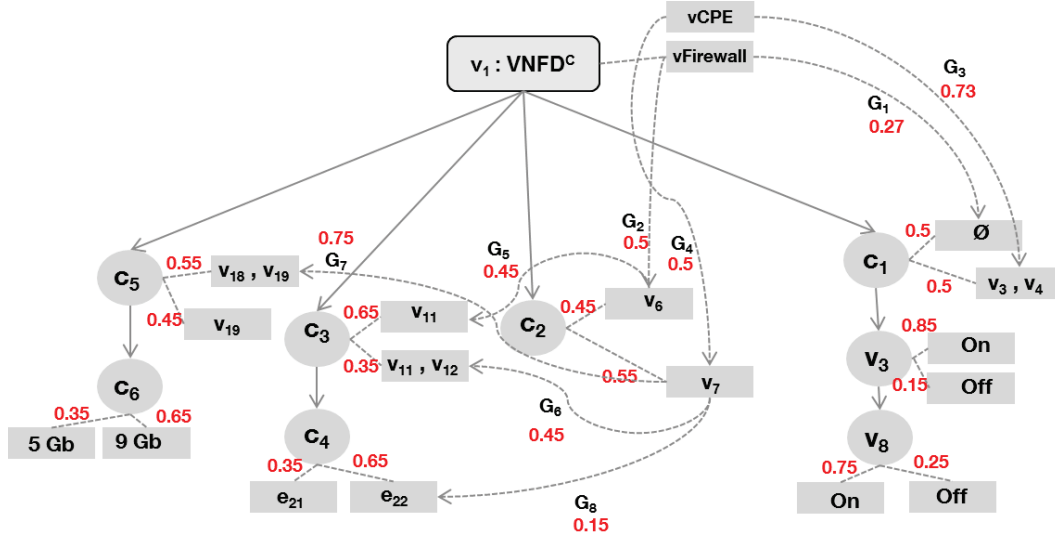
Figure 6.6: Representation of a configuration guidance model that is derived from the configurable deployment descriptor model in Figure 6.4
