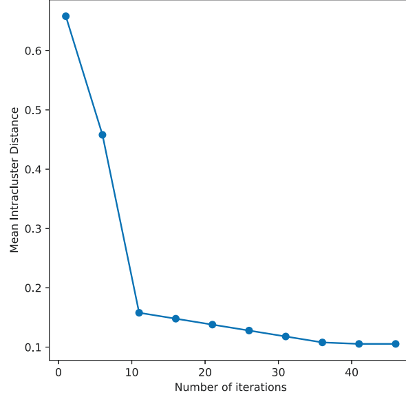
Figure 6.11: Intra-cluster mean similarity distance per iteration, VDU nodes, k=200
